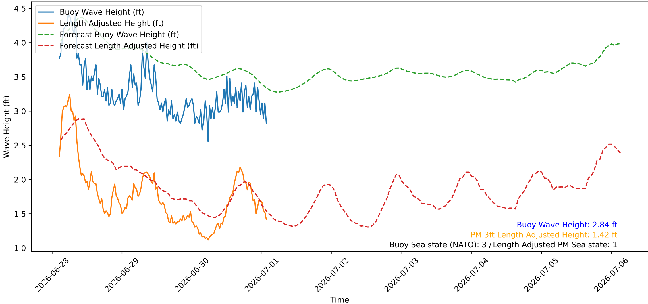
Wave Heights over Time for Oceanside Harbor at 2026-07-01 02:30:26
