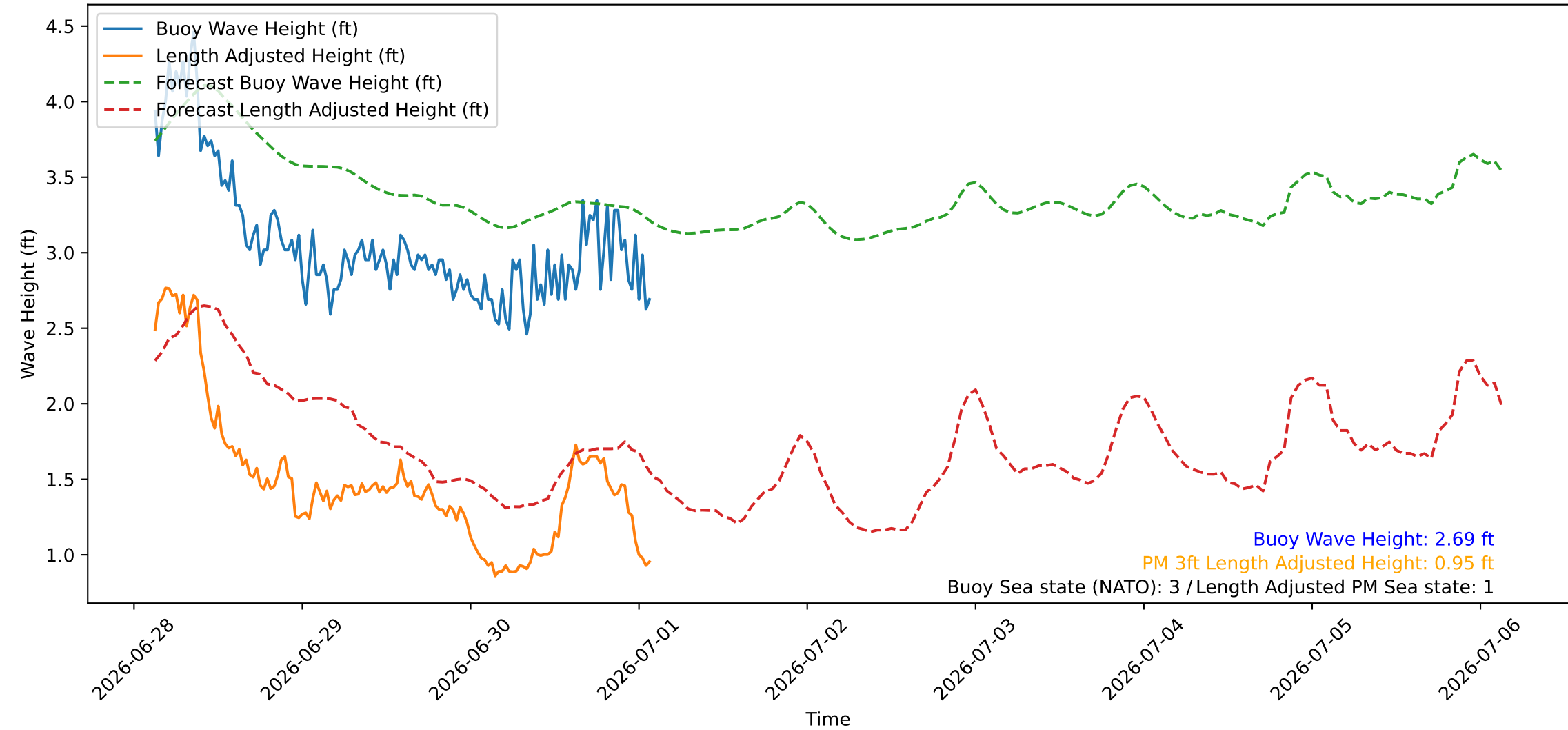
Wave Heights over Time for Red Beach at 2026-07-01 02:30:45
