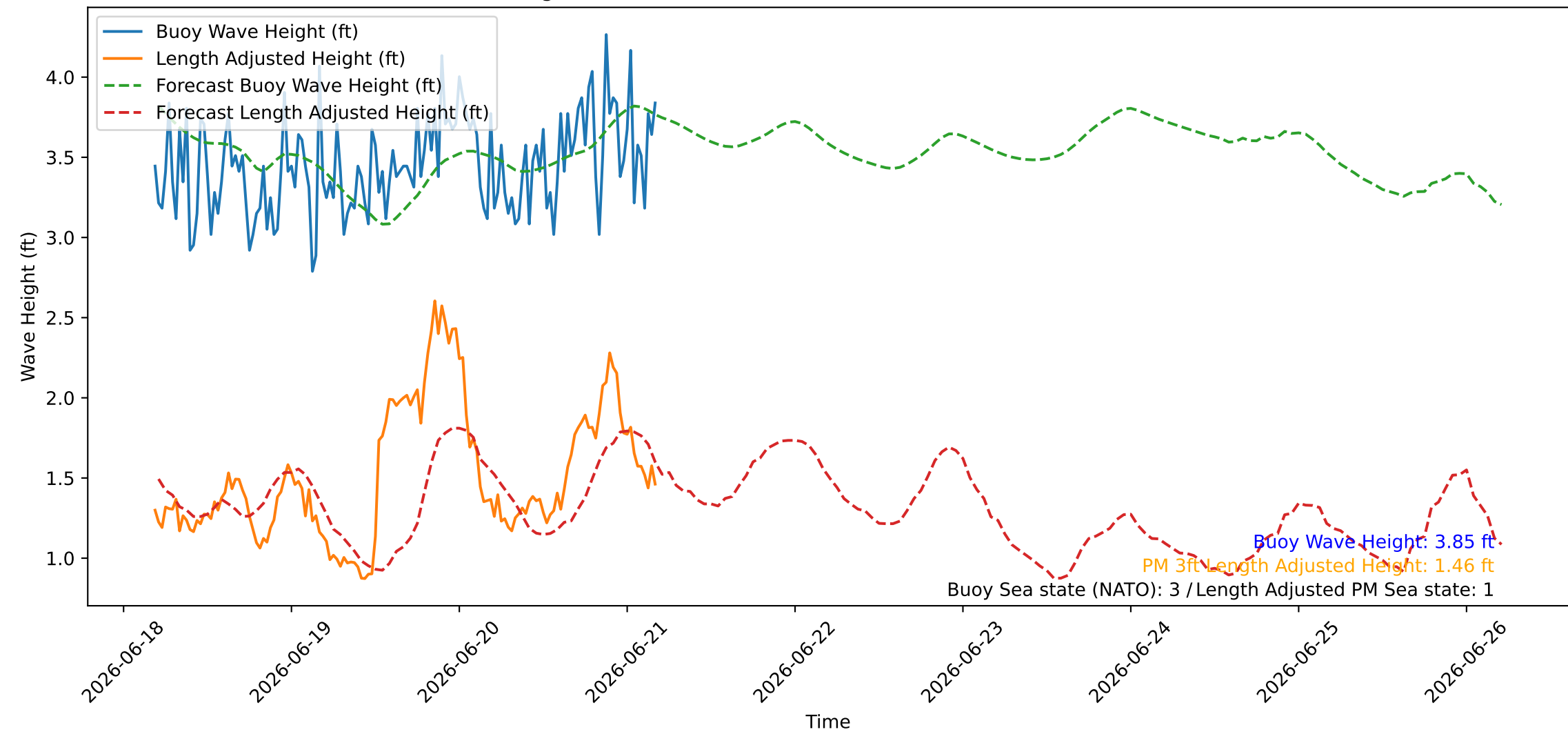
Wave Heights over Time for Oceanside Harbor at 2026-06-21 04:40:26
