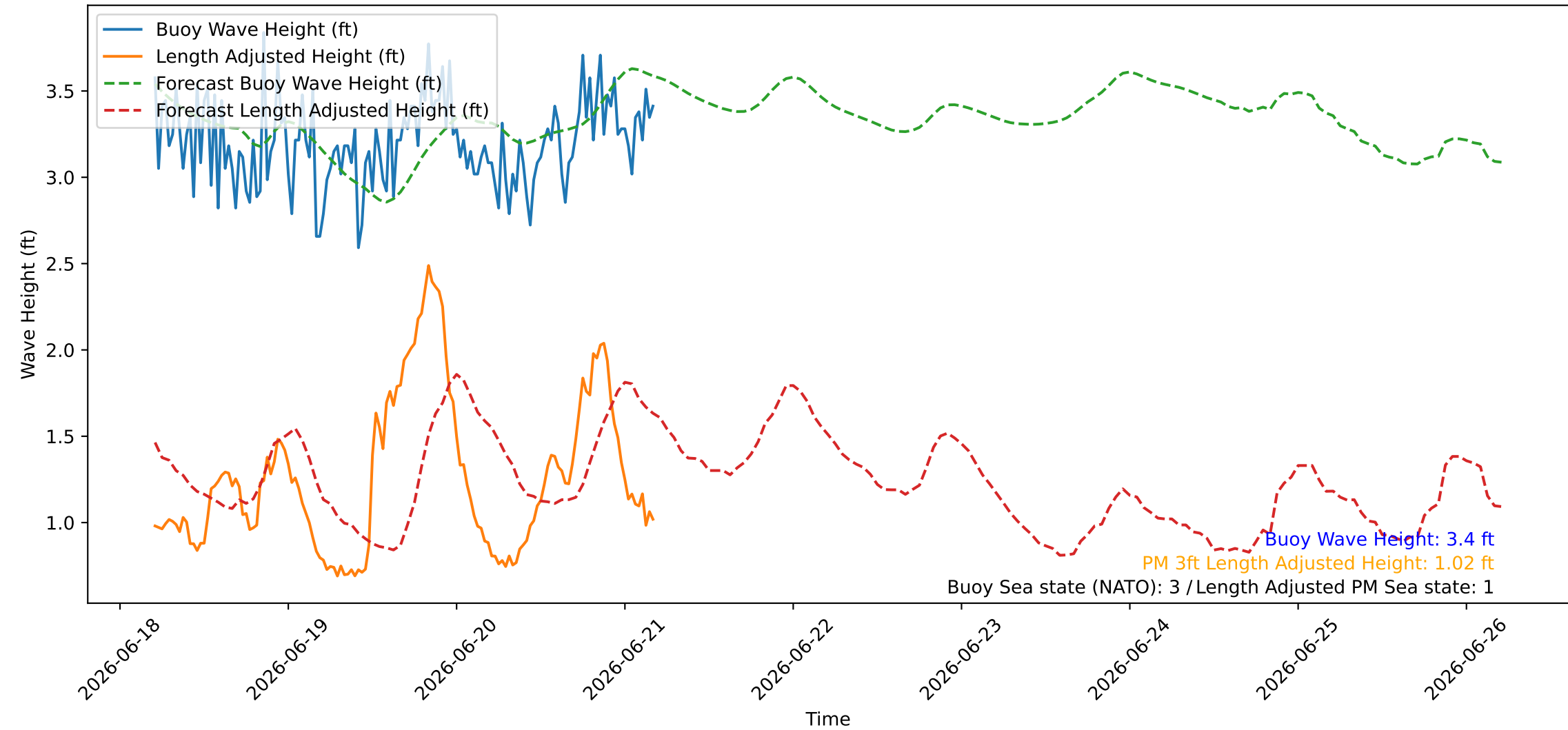
Wave Heights over Time for Red Beach at 2026-06-21 04:40:45
