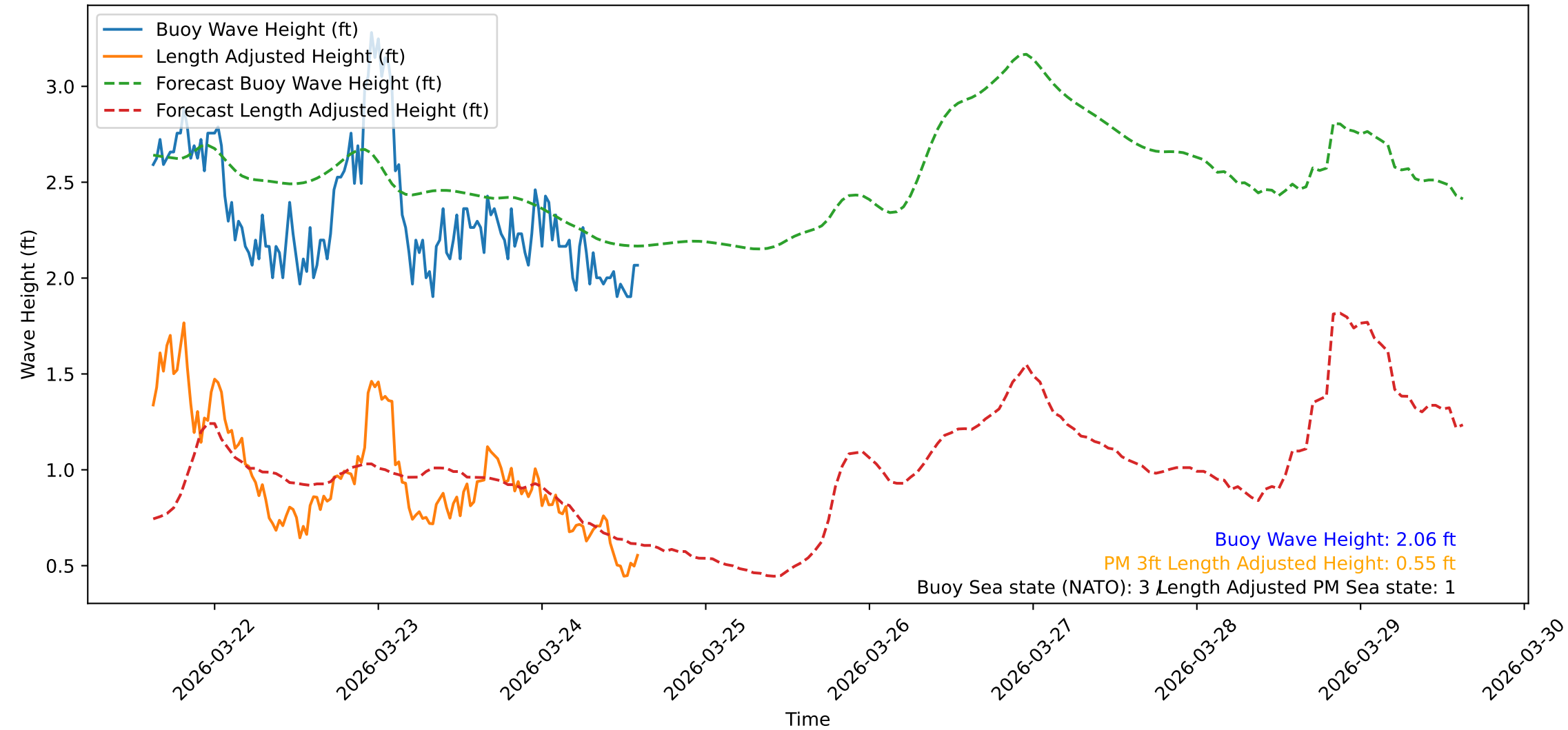
Wave Heights over Time for Green Beach at 2026-03-24 14:51:11
