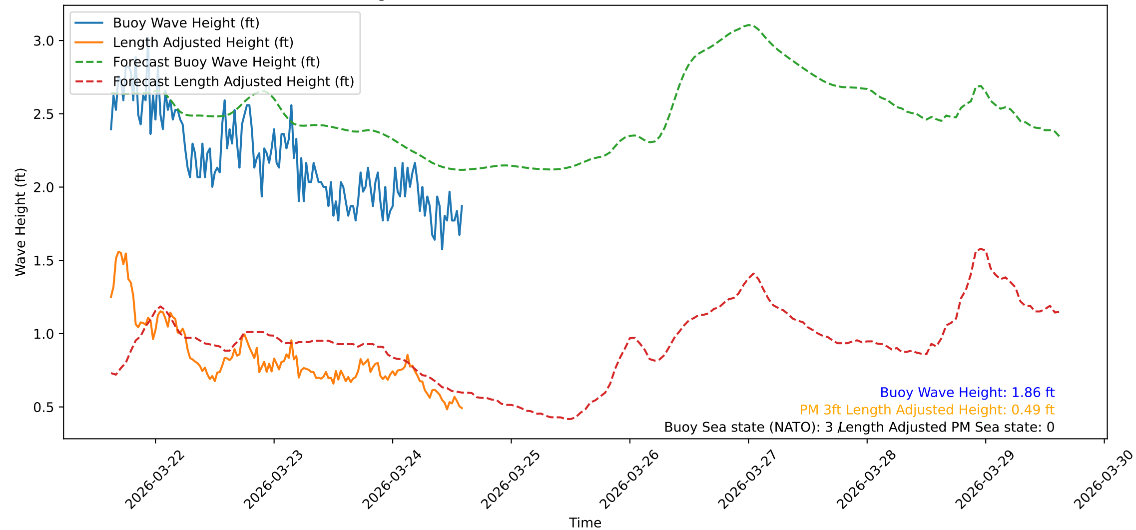
Wave Heights over Time for Oceanside Harbor at 2026-03-24 14:50:32
