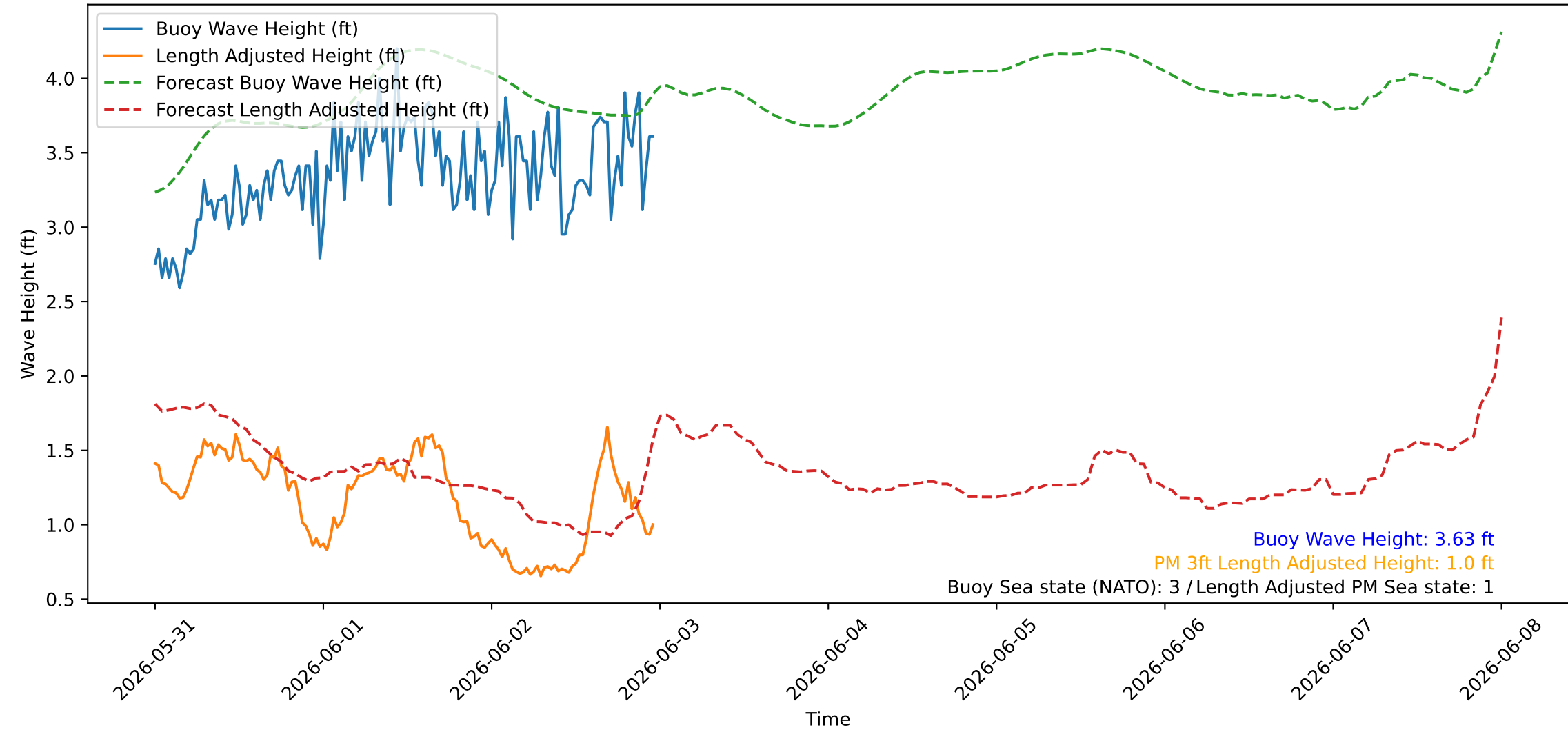
Wave Heights over Time for Red Beach at 2026-06-02 23:40:45
