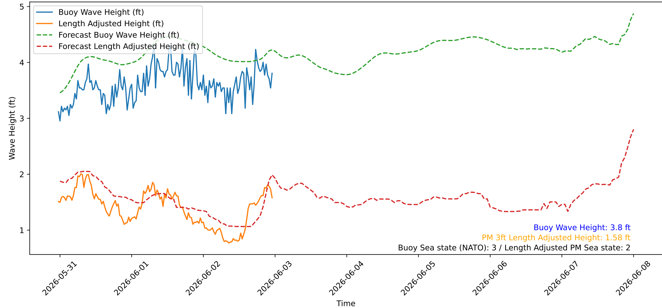
Wave Heights over Time for Green Beach at 2026-06-02 23:41:08
