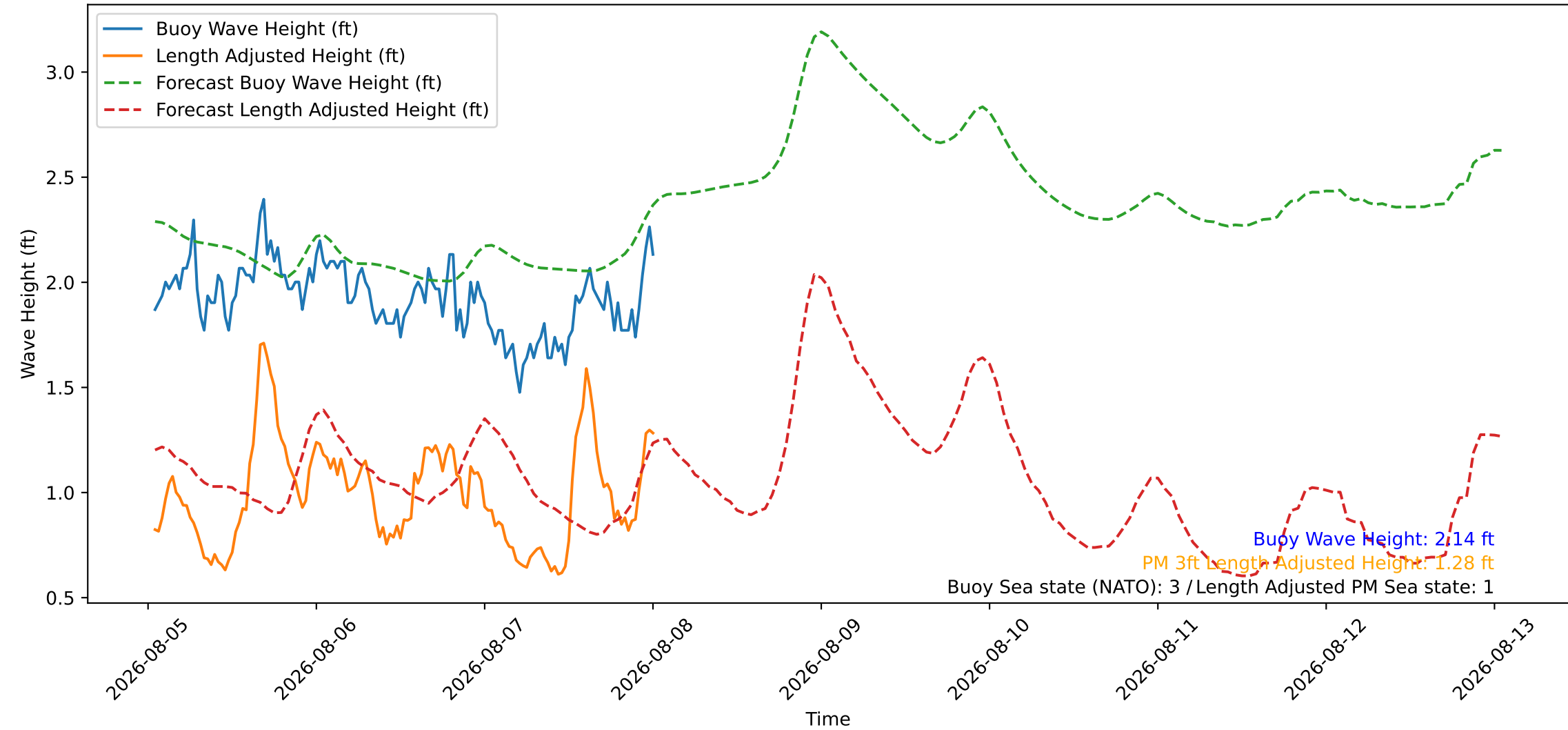
Wave Heights over Time for Red Beach at 2026-08-08 00:50:47
