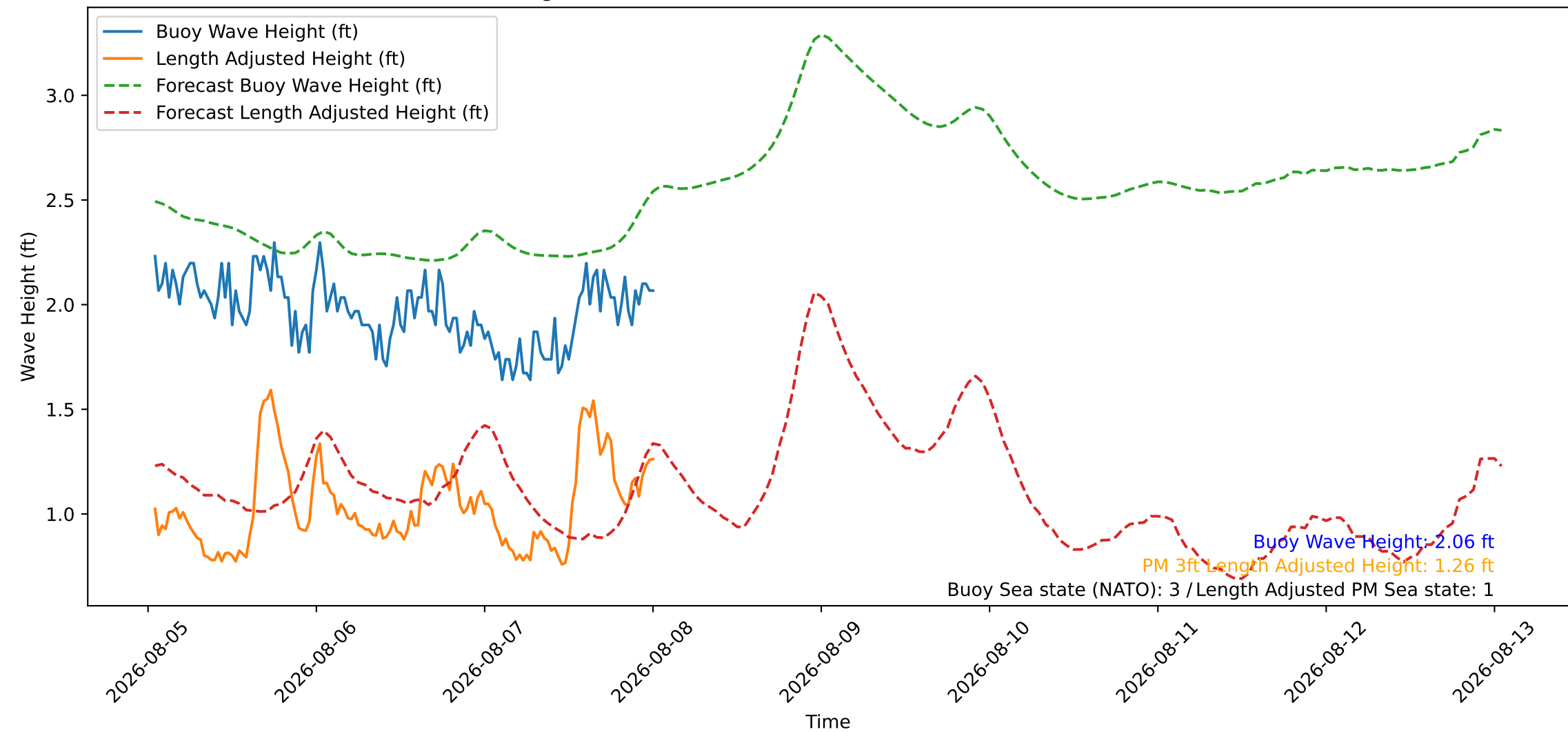
Wave Heights over Time for Oceanside Harbor at 2026-08-08 00:50:26
