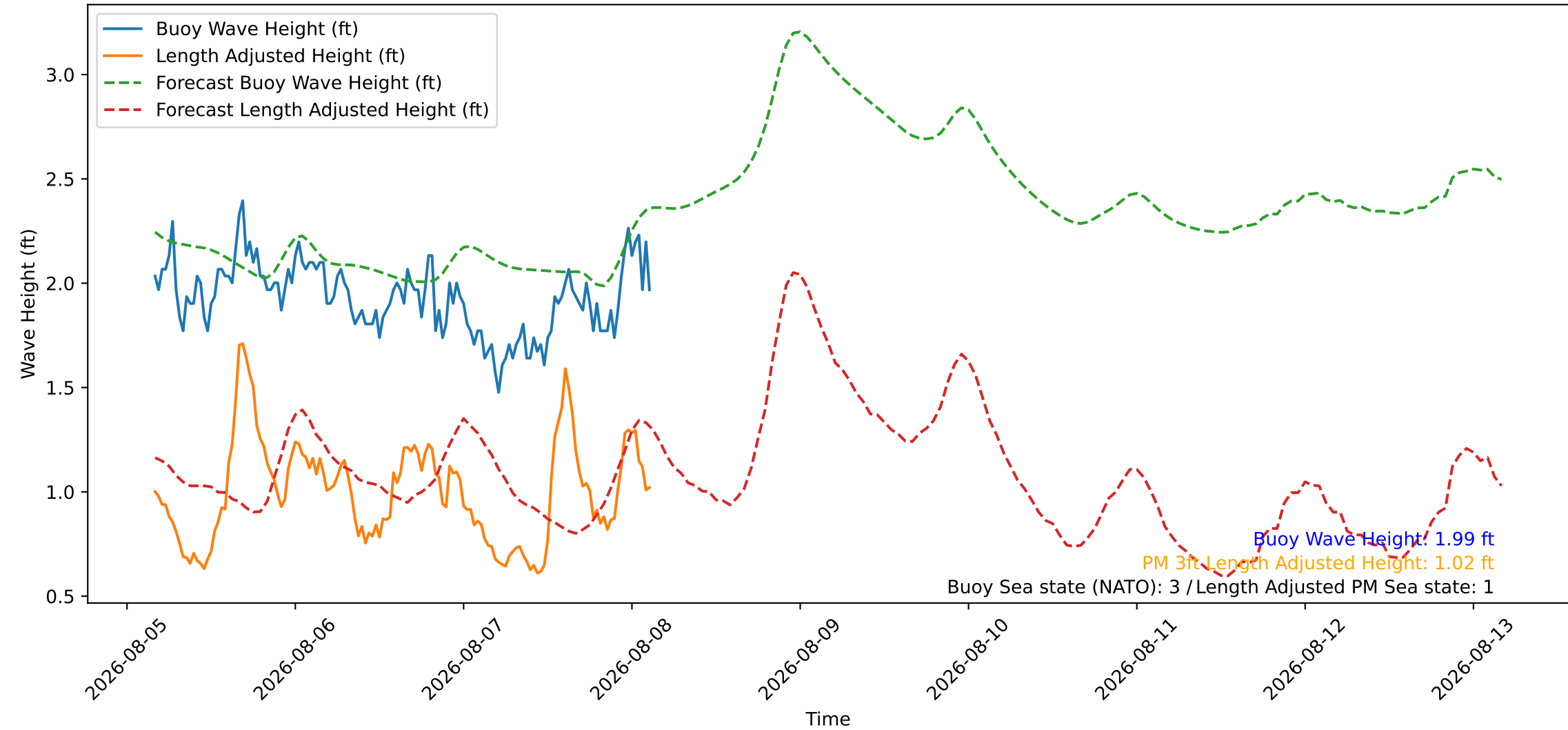
Wave Heights over Time for Red Beach at 2026-08-08 03:50:47
