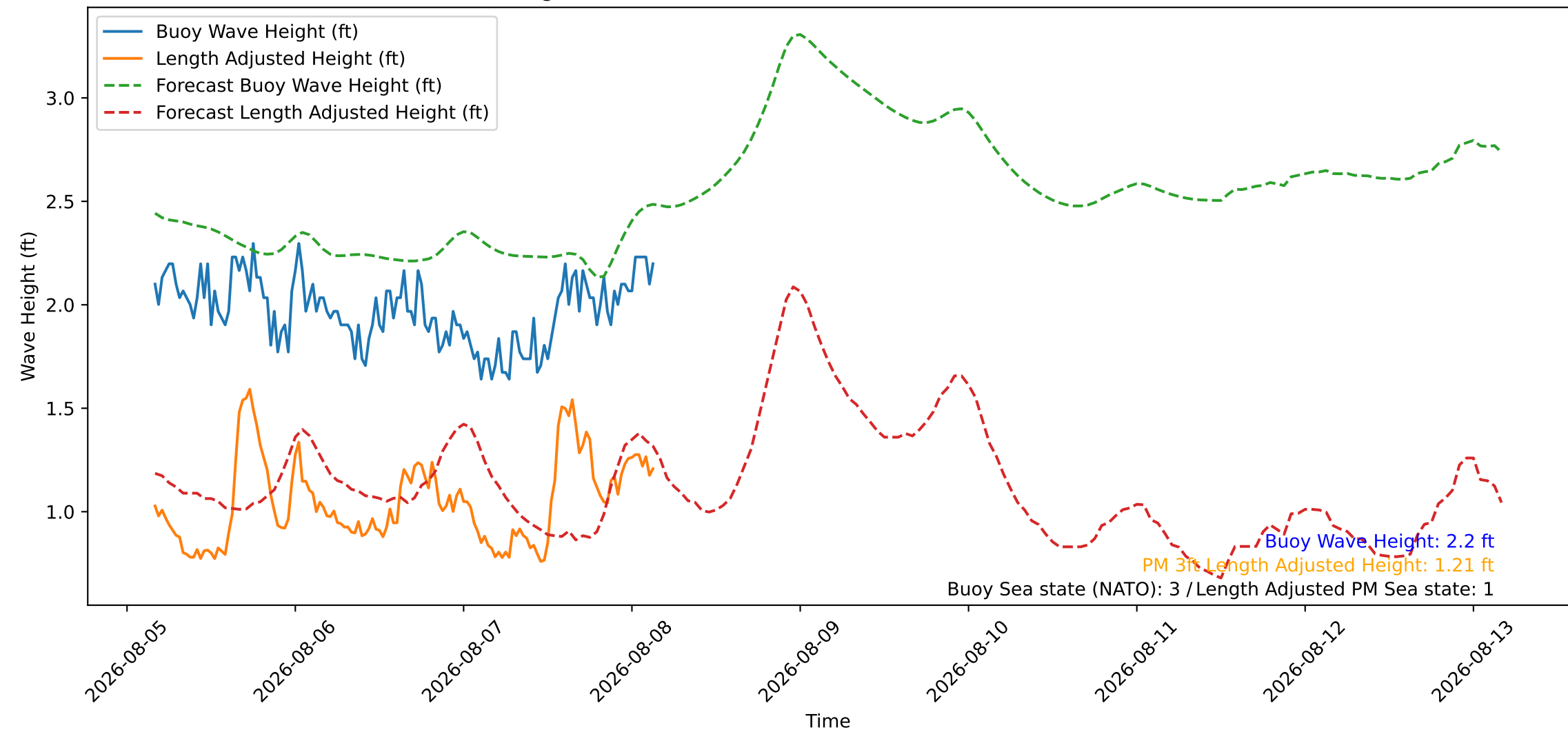
Wave Heights over Time for Oceanside Harbor at 2026-08-08 03:50:26
