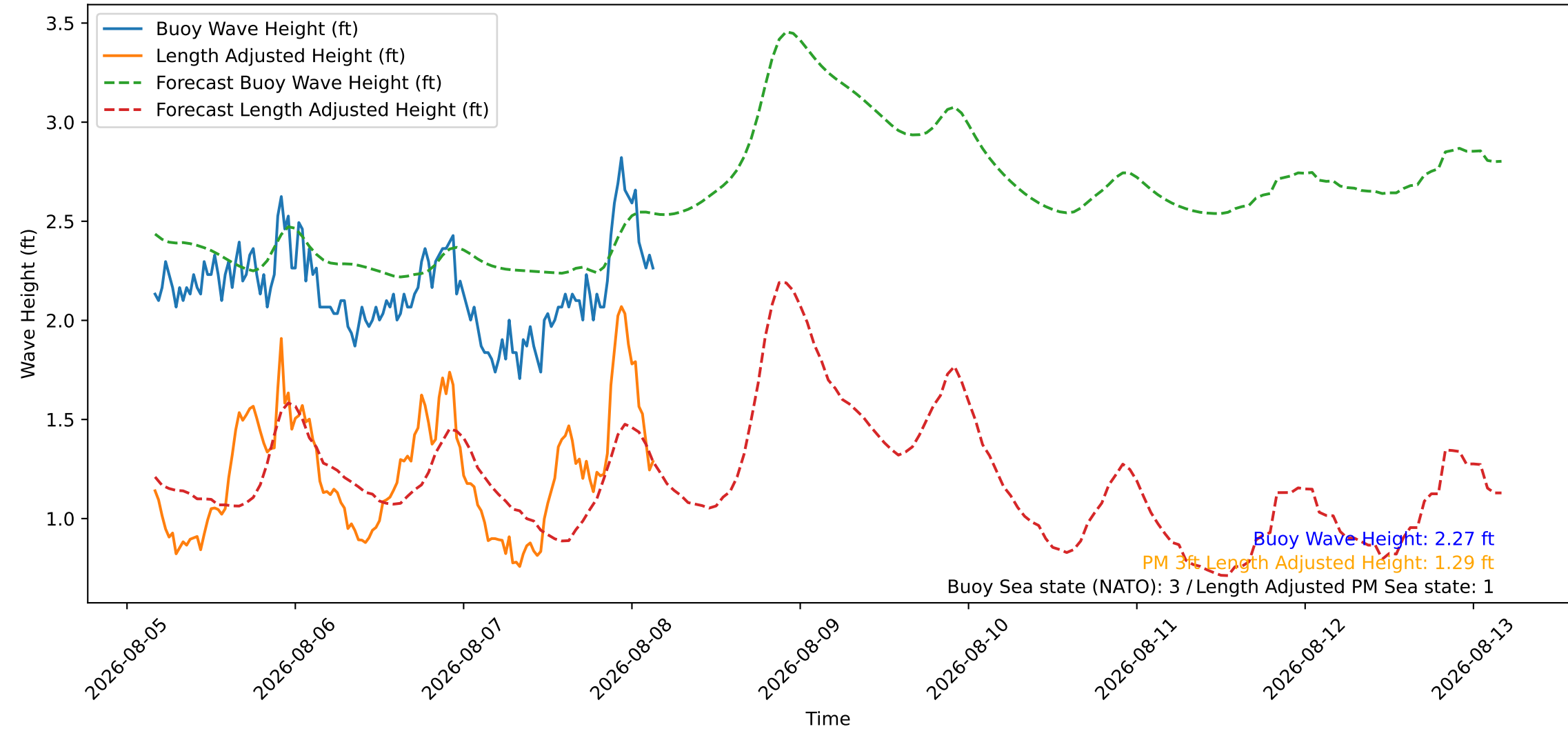
Wave Heights over Time for Green Beach at 2026-08-08 03:51:09
