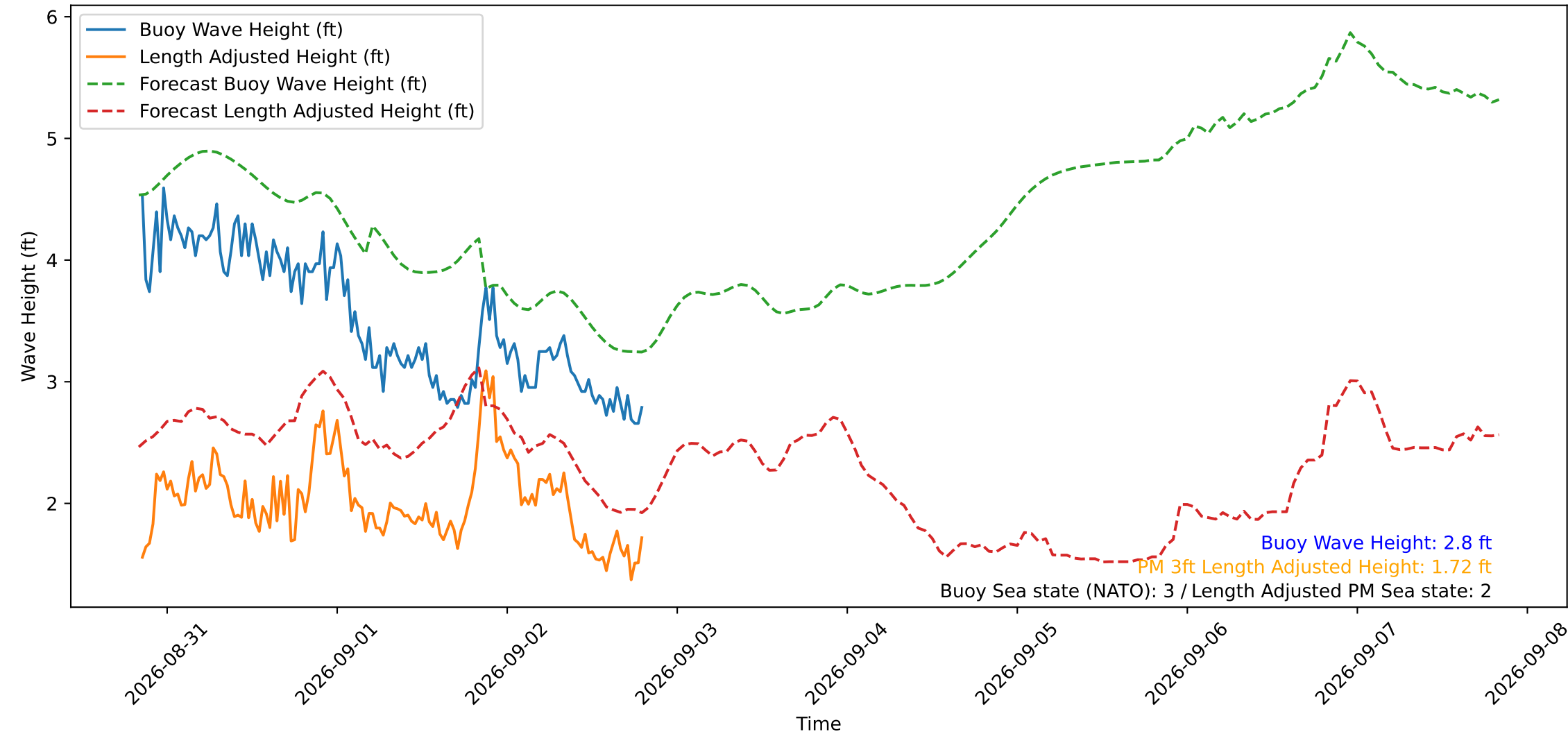
Wave Heights over Time for Green Beach at 2026-09-02 20:01:13
