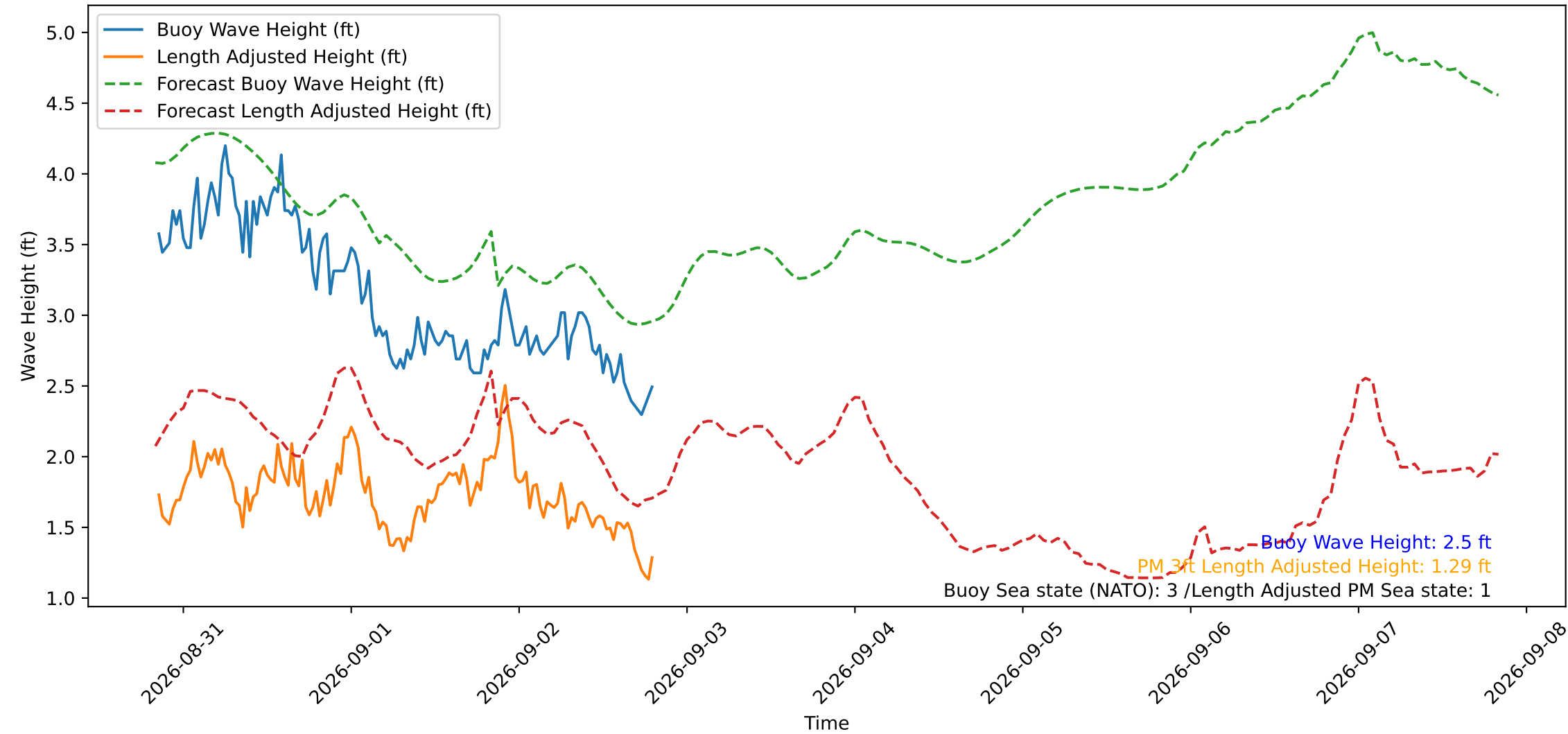
Wave Heights over Time for Red Beach at 2026-09-02 20:00:49
