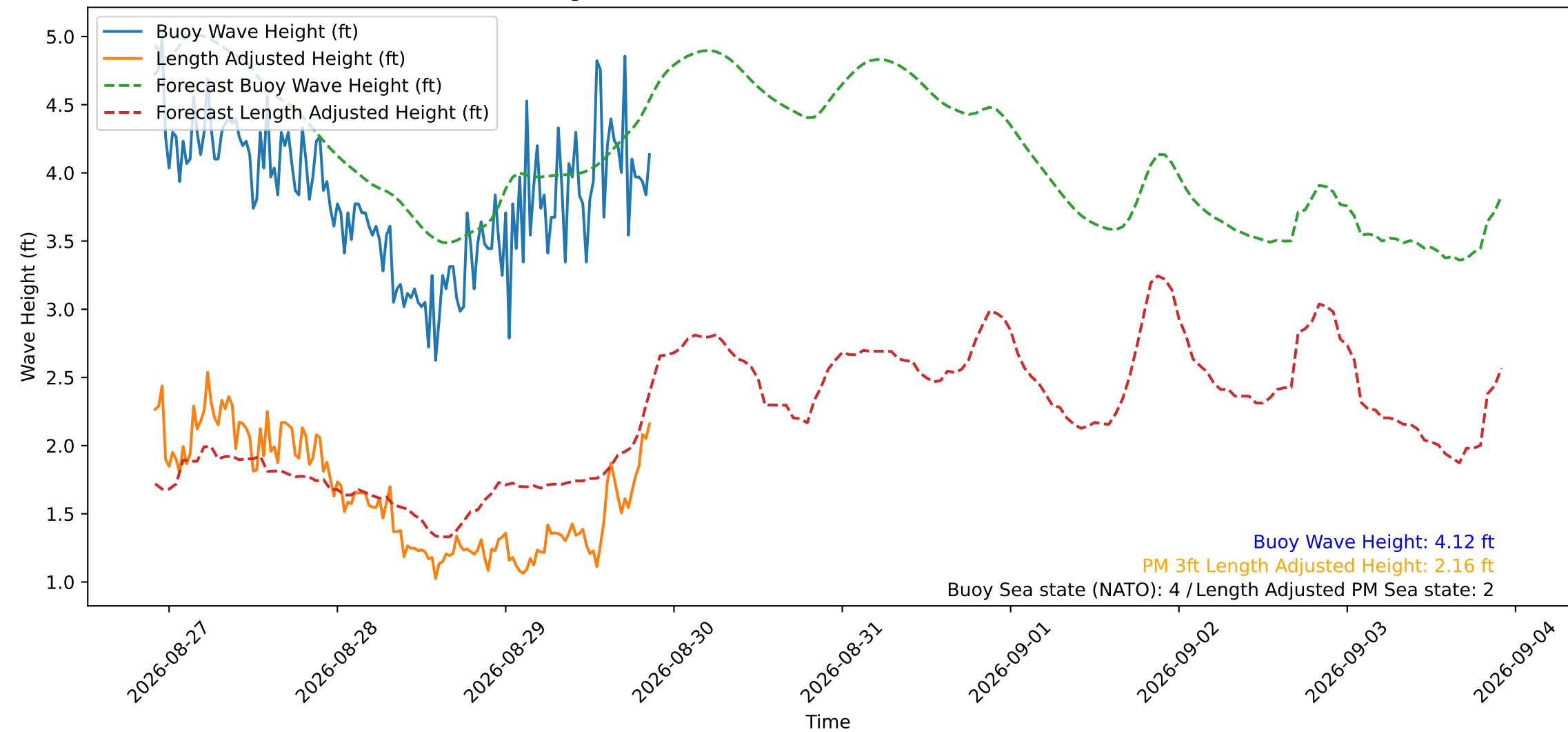
Wave Heights over Time for Green Beach at 2026-08-29 21:31:12
