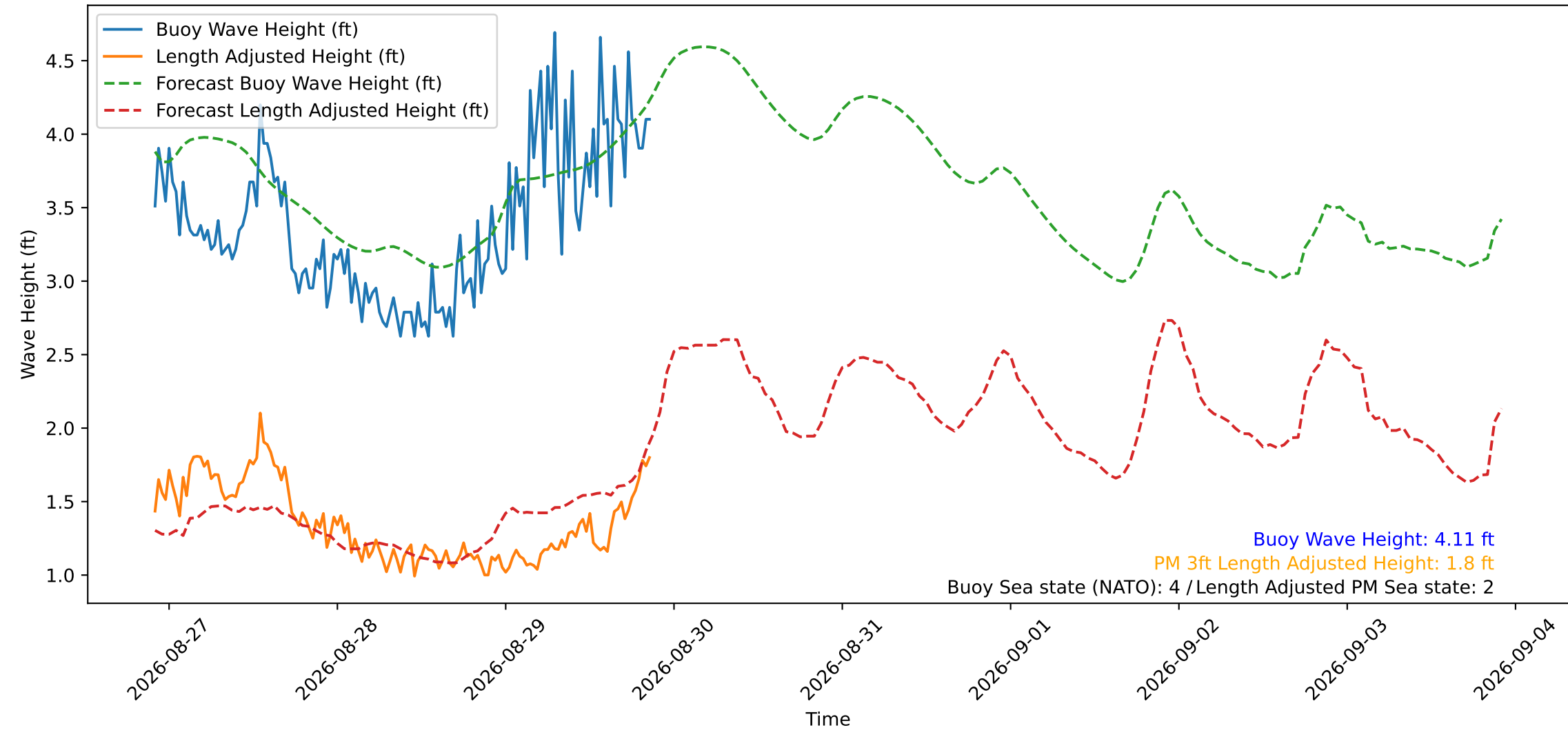
Wave Heights over Time for Red Beach at 2026-08-29 21:30:49
