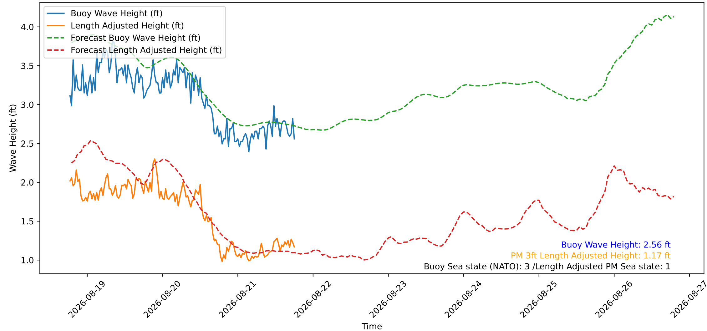
Wave Heights over Time for Oceanside Harbor at 2026-08-21 18:40:26
