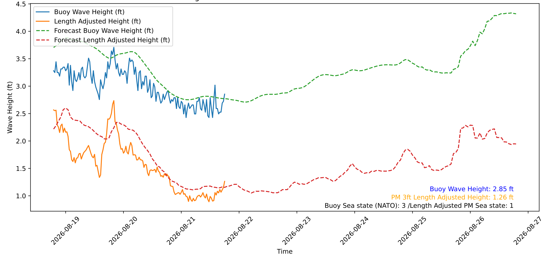
Wave Heights over Time for Green Beach at 2026-08-21 18:41:09
