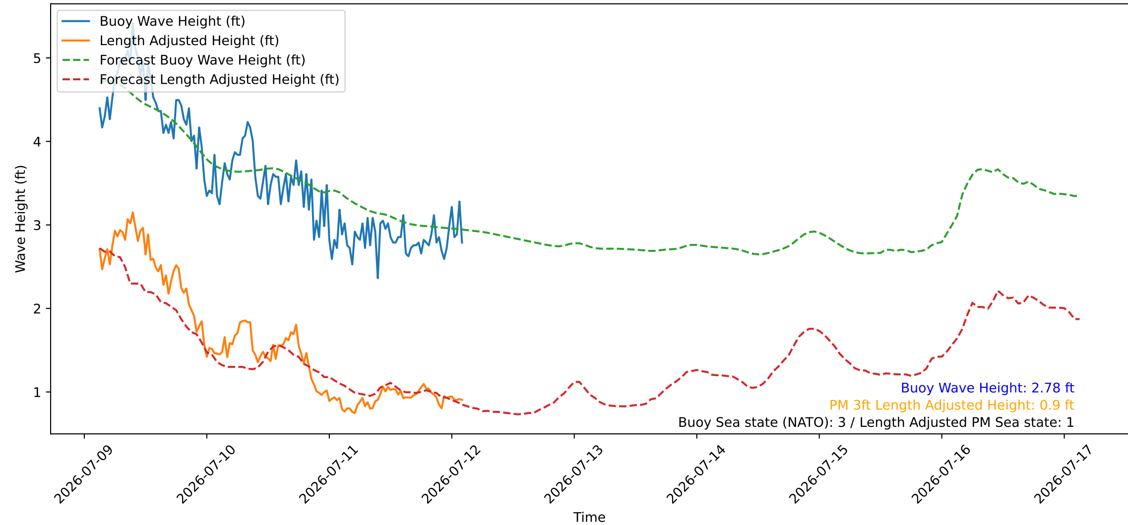
Wave Heights over Time for Oceanside Harbor at 2026-07-12 02:50:27
