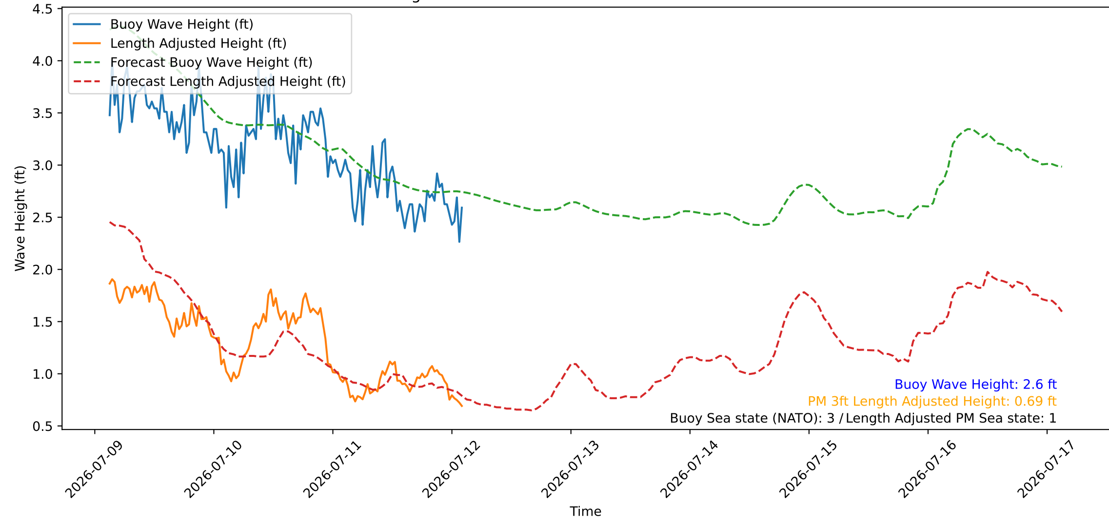
Wave Heights over Time for Red Beach at 2026-07-12 02:50:47
