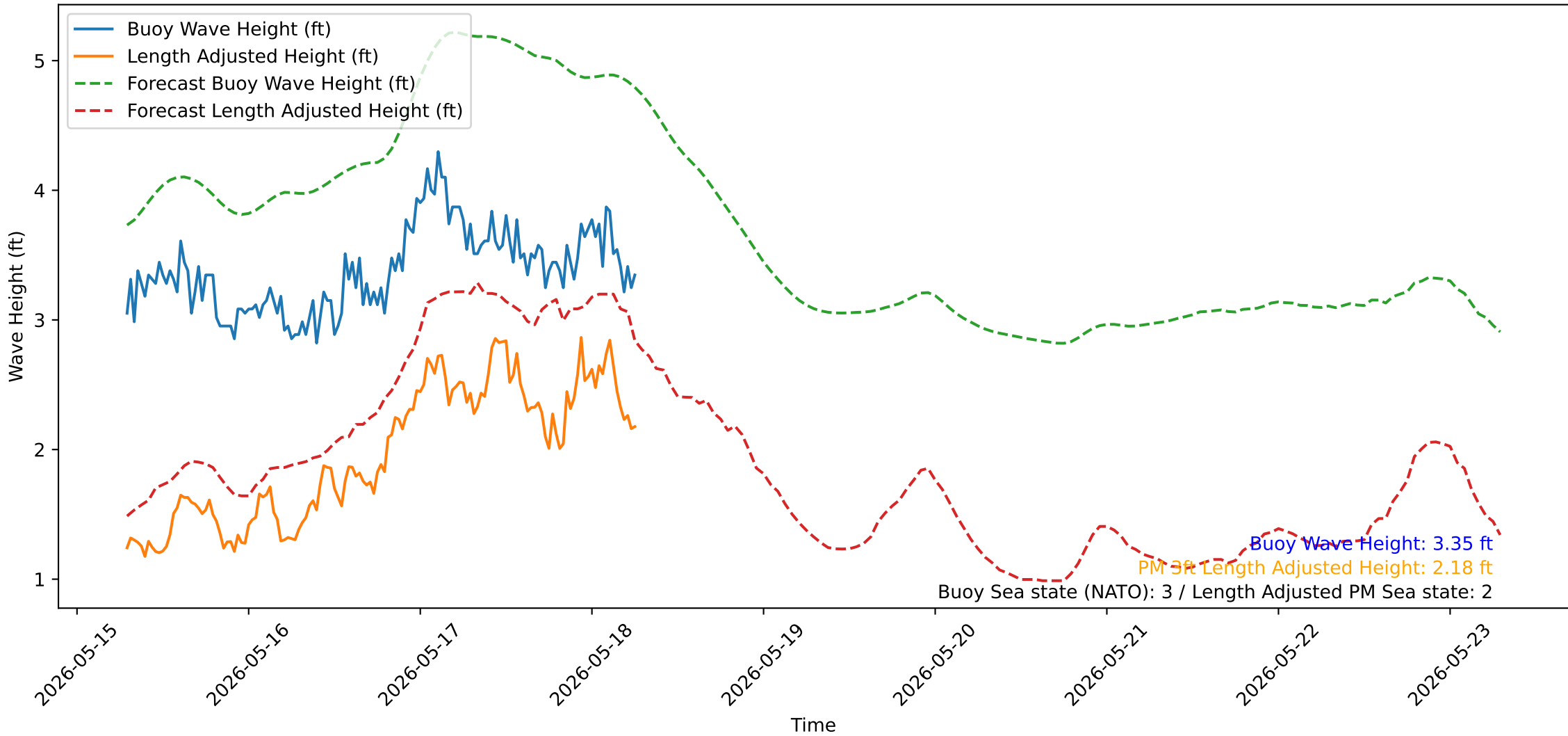
Wave Heights over Time for Oceanside Harbor at 2026-05-18 06:50:32
