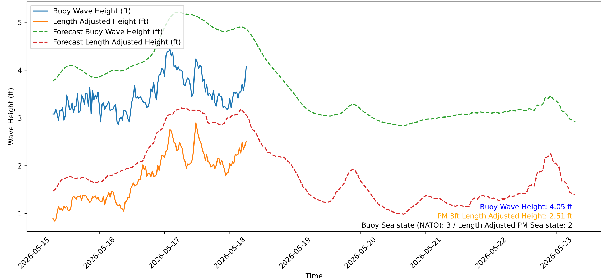
Wave Heights over Time for Green Beach at 2026-05-18 06:51:14
