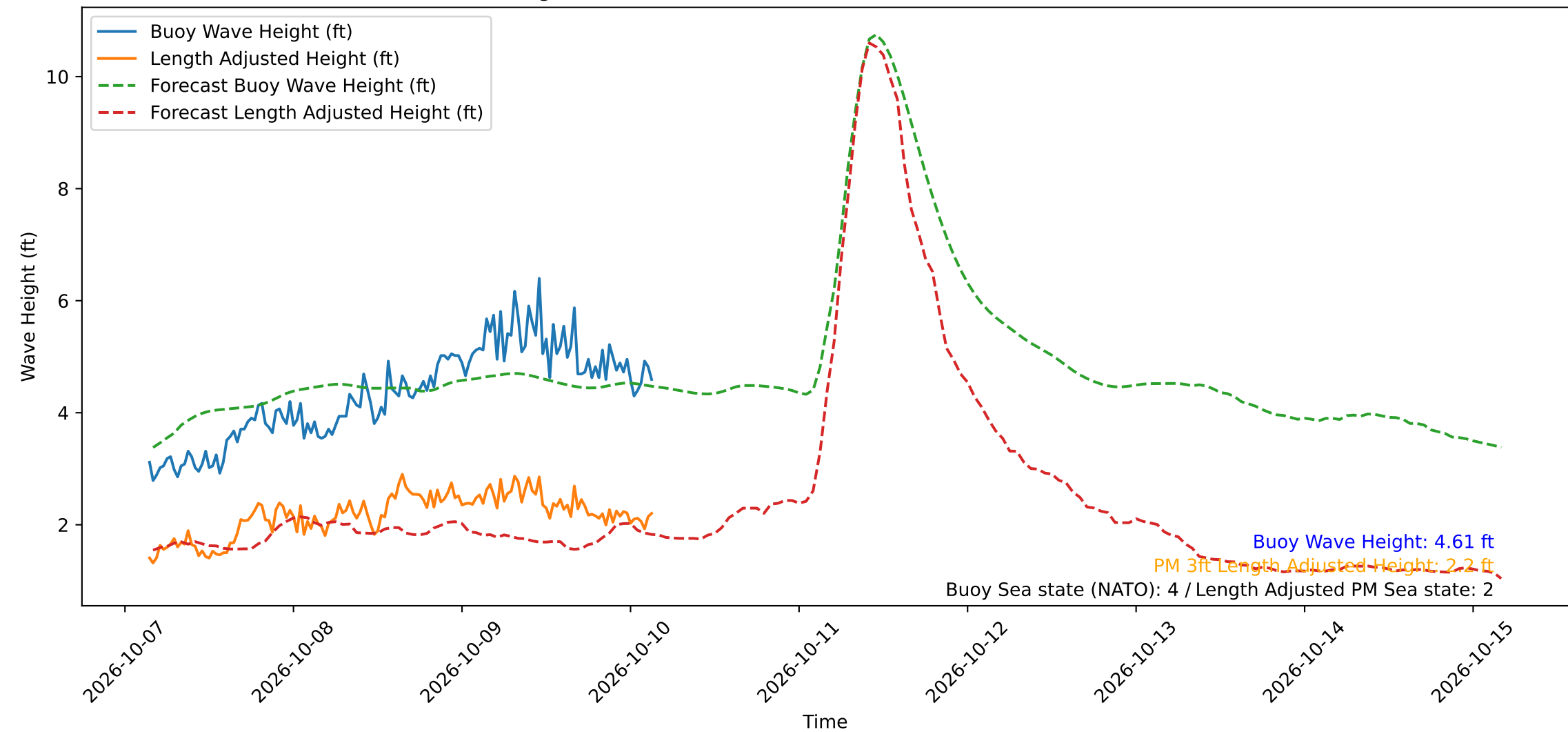
Wave Heights over Time for Oceanside Harbor at 2026-10-10 03:30:30
