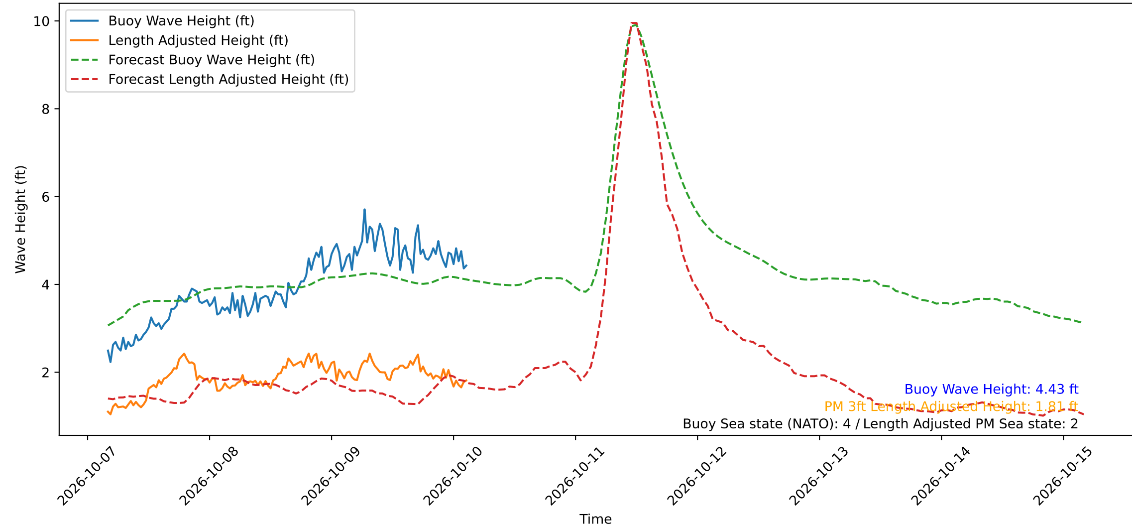
Wave Heights over Time for Red Beach at 2026-10-10 03:30:49
