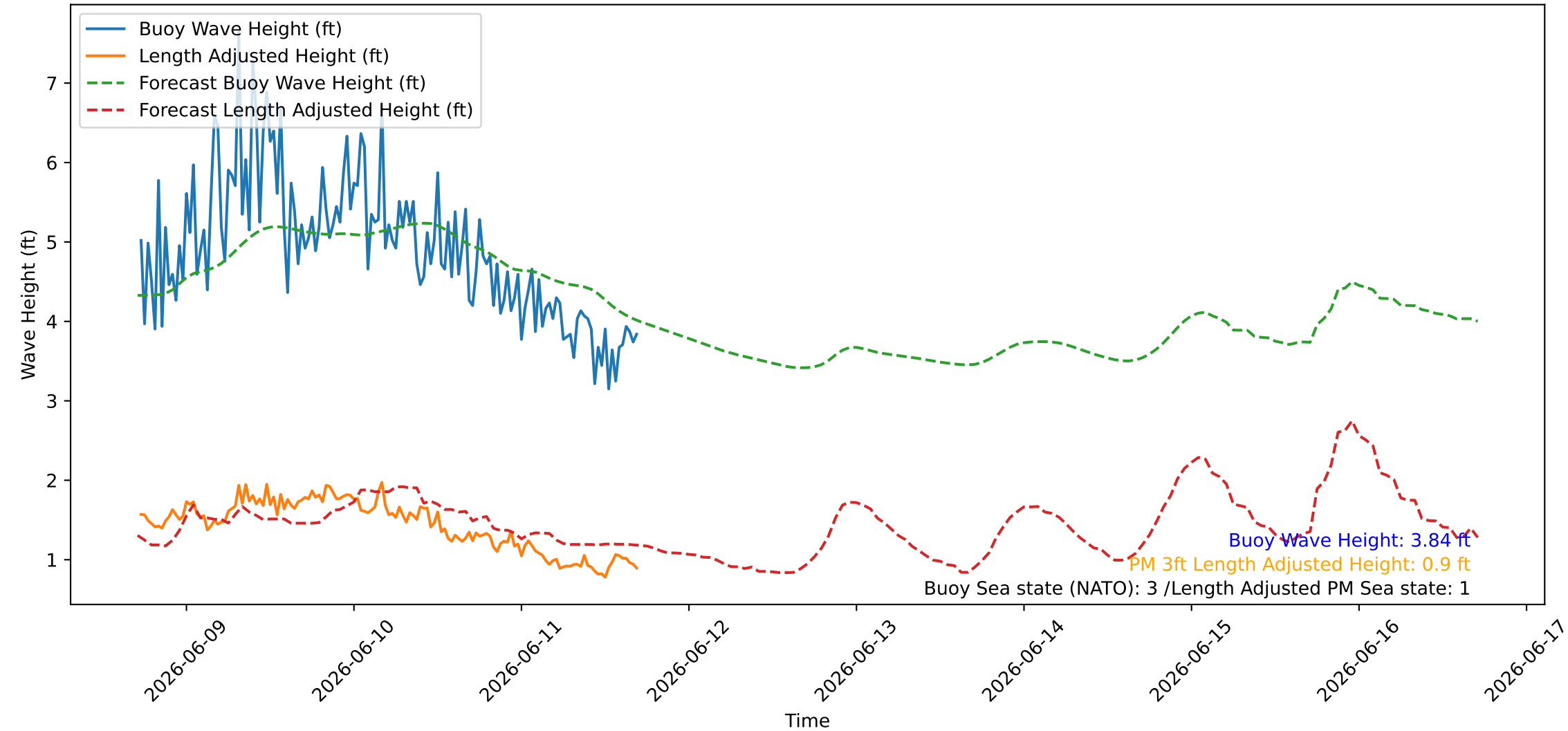
Wave Heights over Time for Red Beach at 2026-06-11 17:10:46
