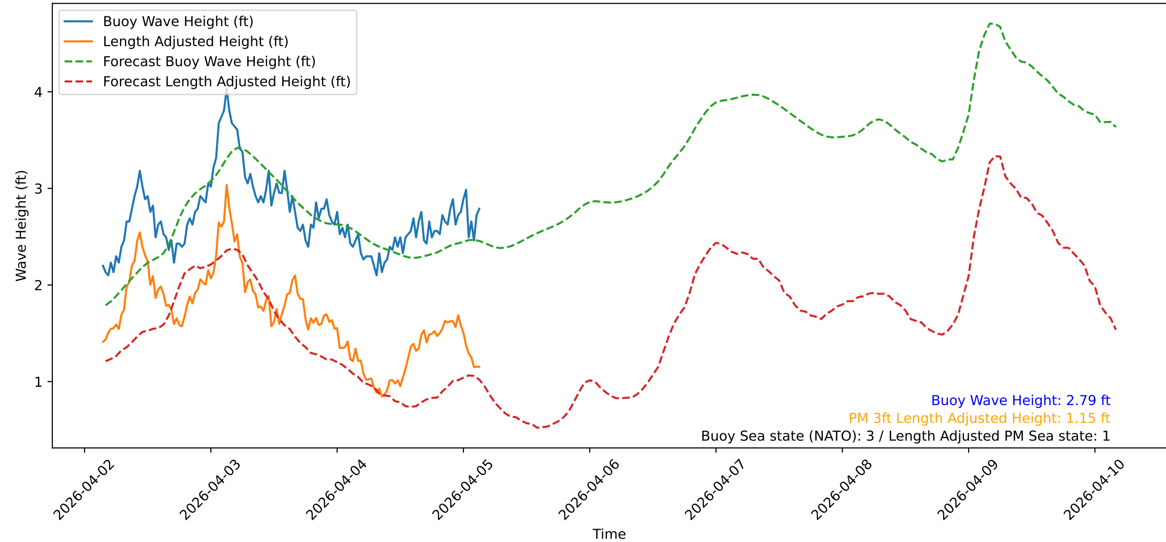
Wave Heights over Time for Oceanside Harbor at 2026-04-05 03:40:32
