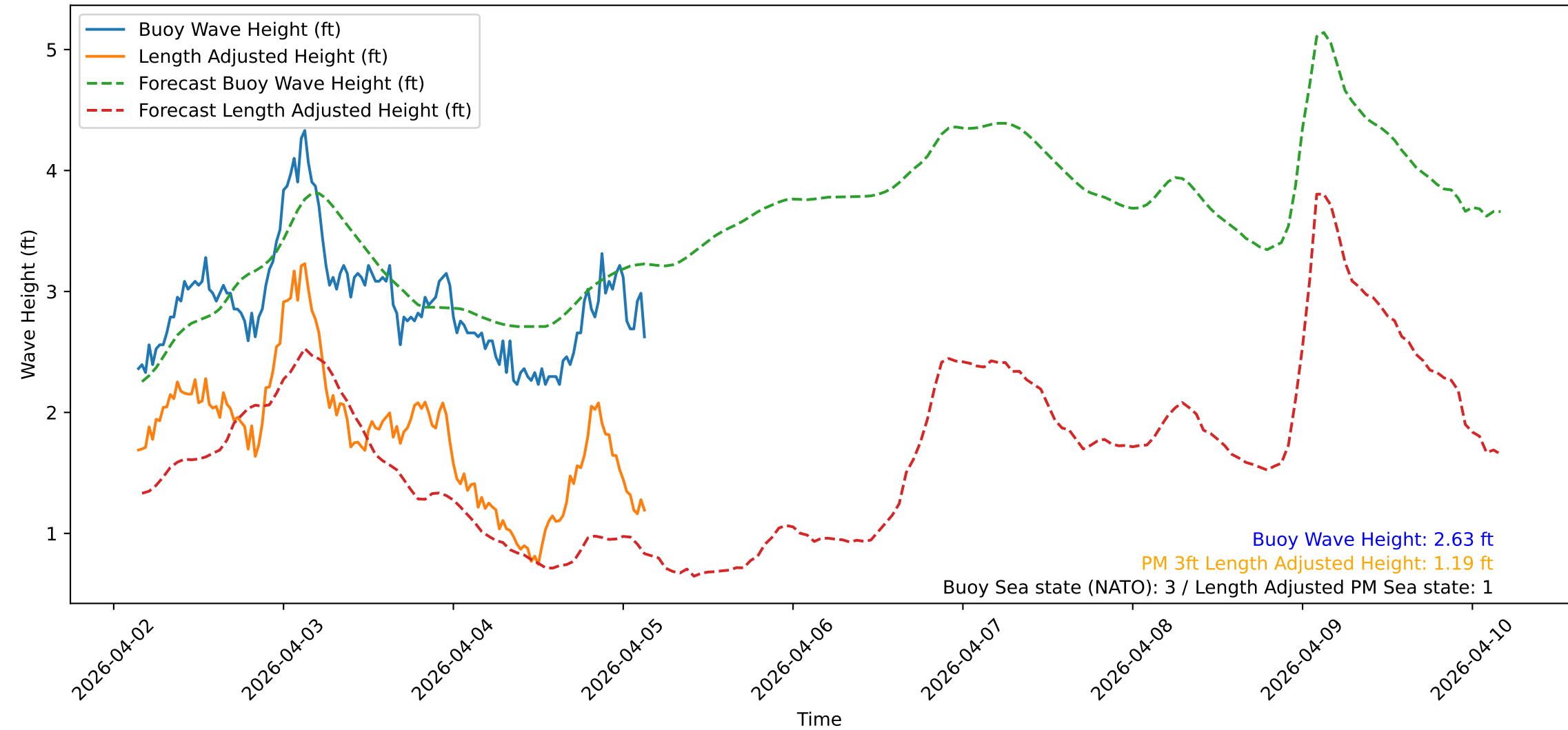
Wave Heights over Time for Green Beach at 2026-04-05 03:41:10
