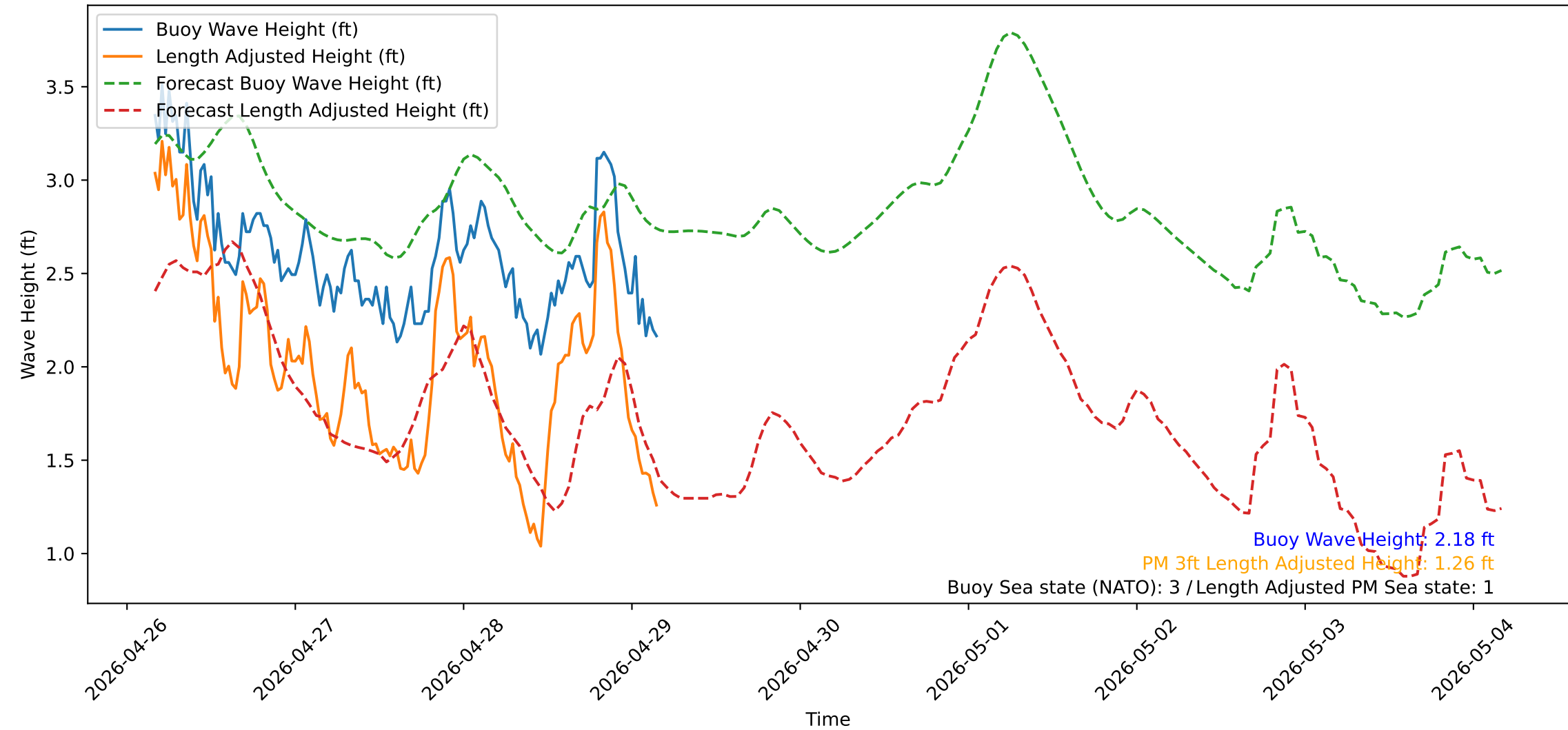
Wave Heights over Time for Green Beach at 2026-04-29 04:11:12
