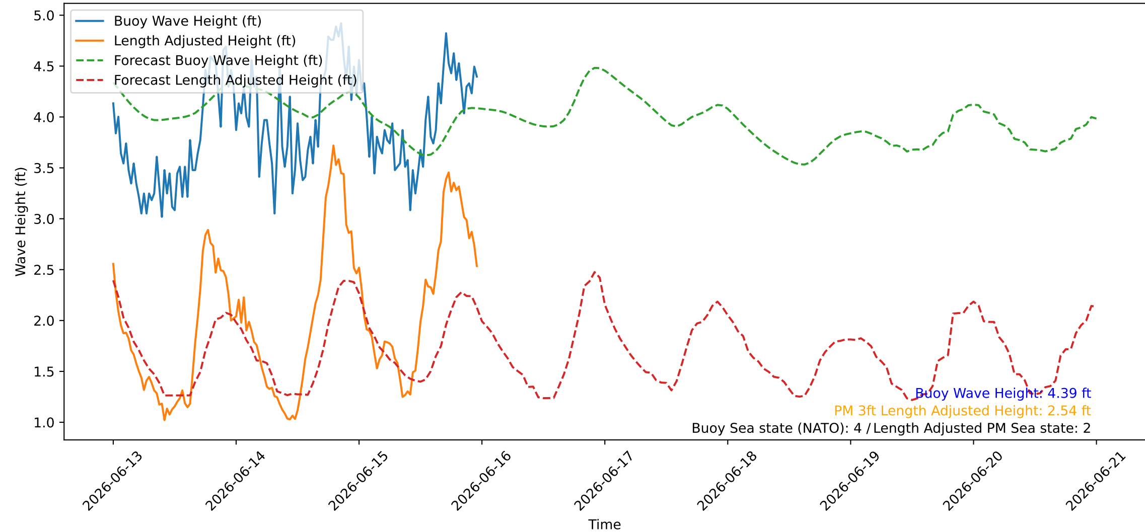
Wave Heights over Time for Green Beach at 2026-06-15 23:51:09
