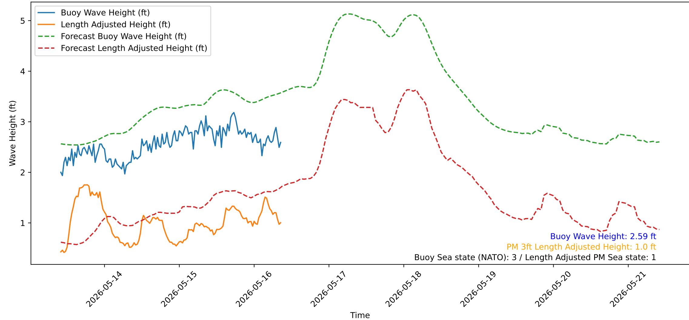
Wave Heights over Time for Red Beach at 2026-05-16 09:30:51
