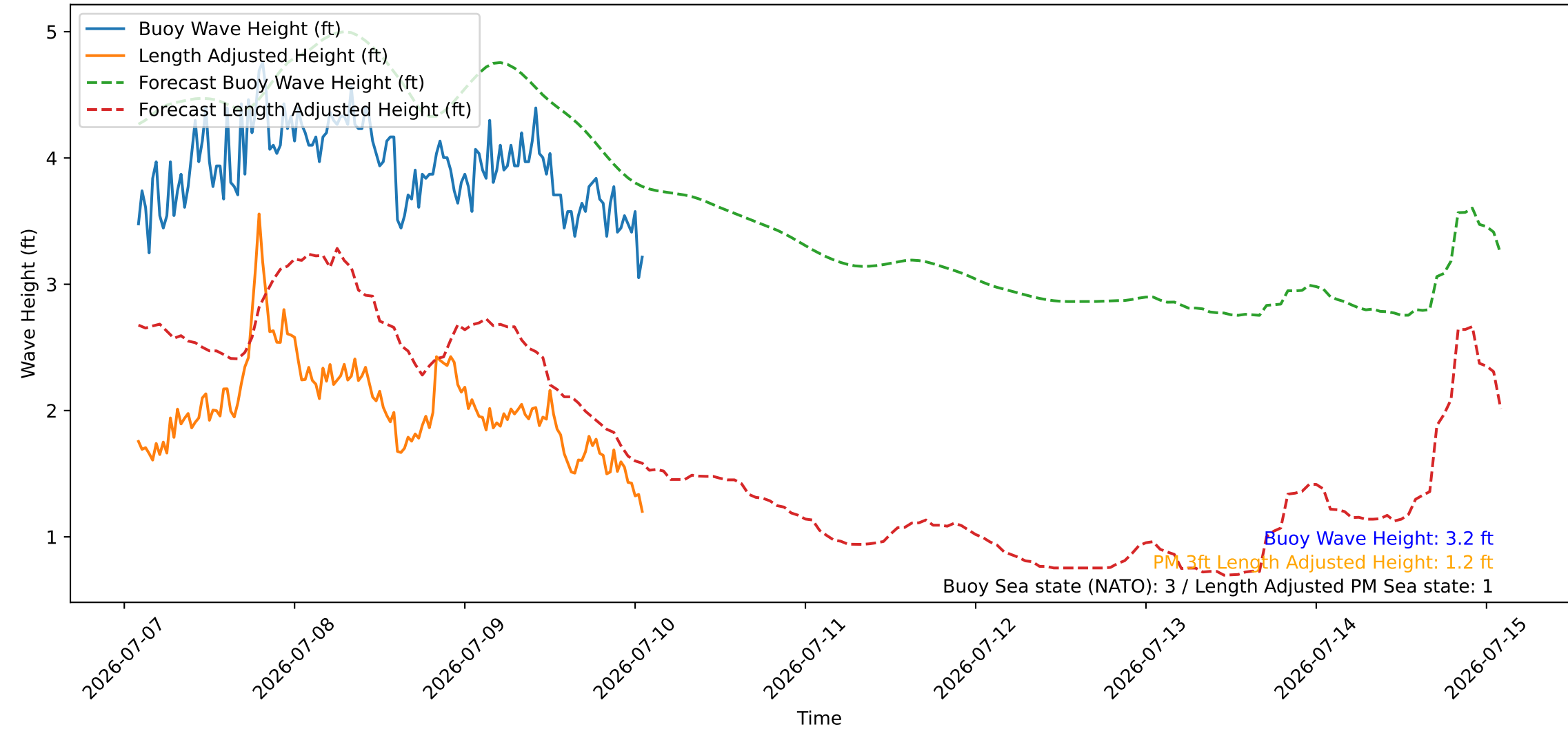
Wave Heights over Time for Green Beach at 2026-07-10 01:51:09
