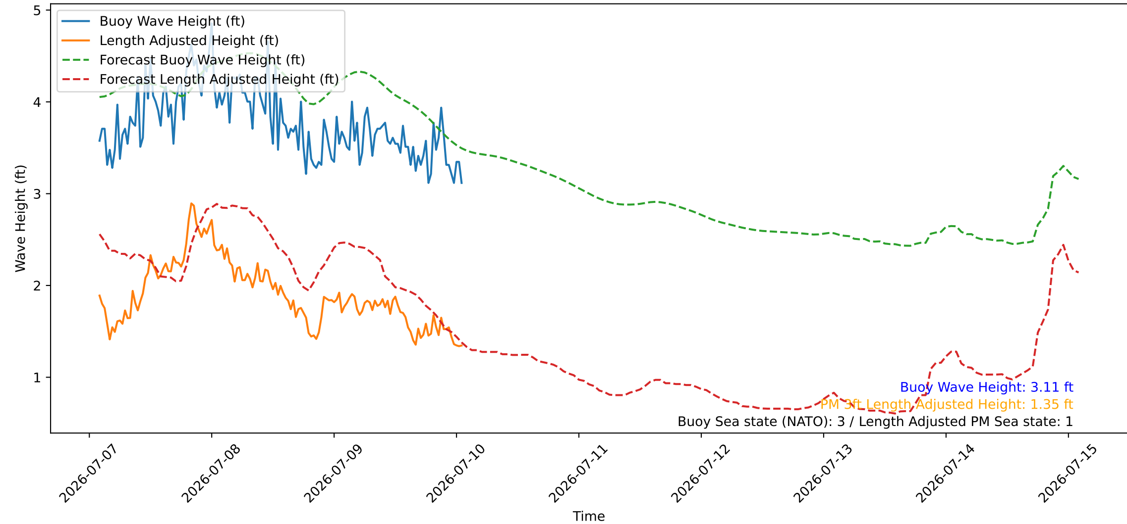
Wave Heights over Time for Red Beach at 2026-07-10 01:50:47
