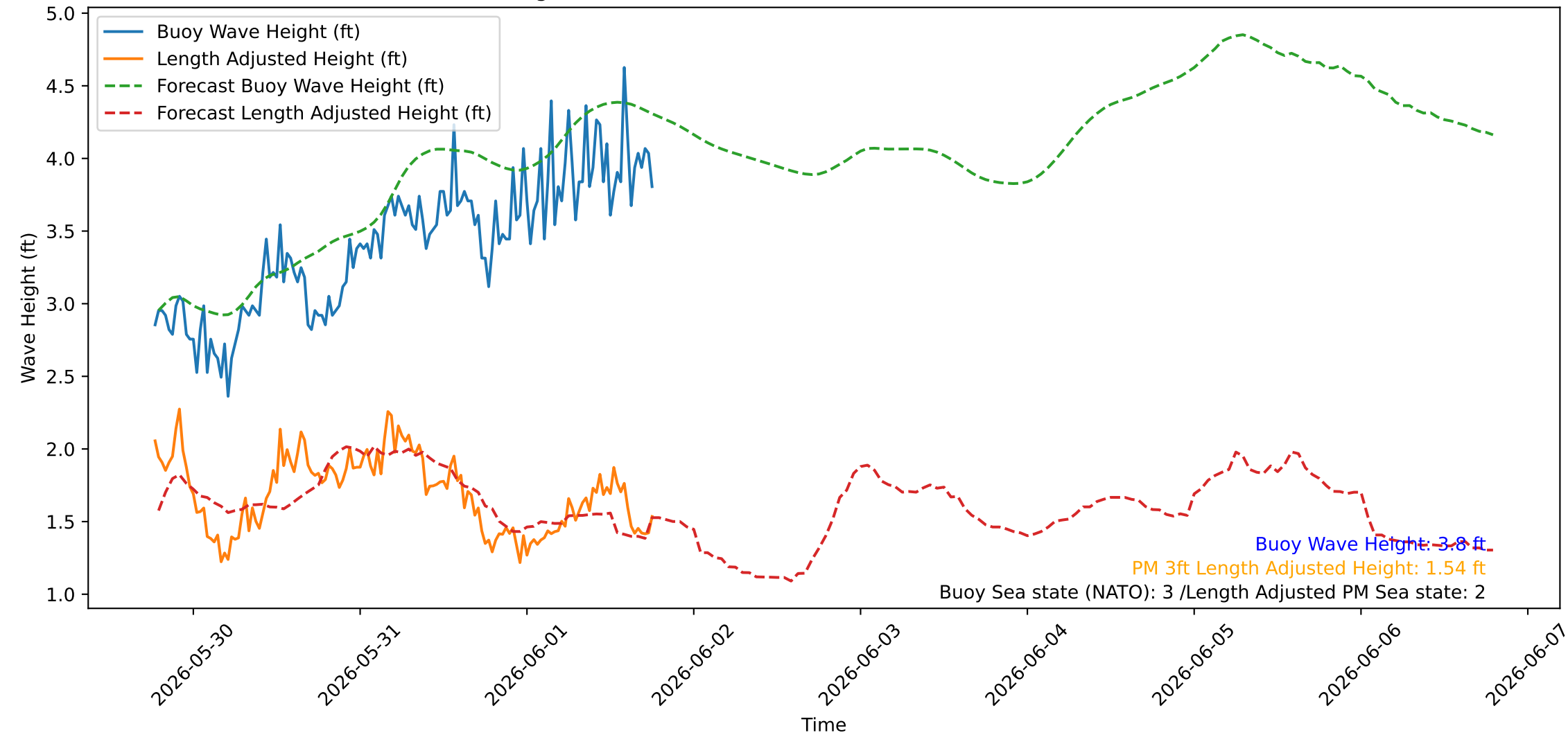
Wave Heights over Time for Oceanside Harbor at 2026-06-01 18:30:26
