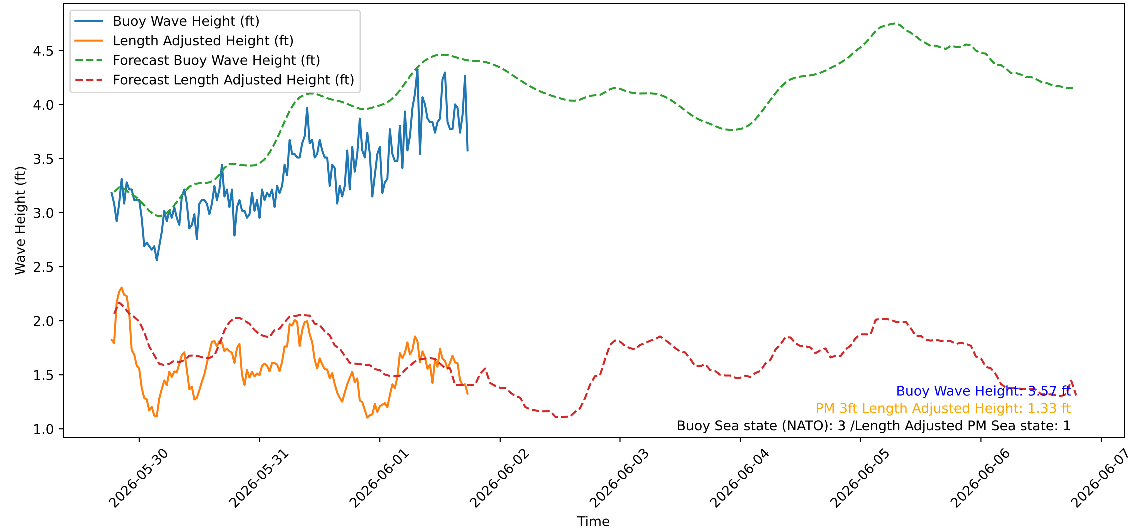
Wave Heights over Time for Green Beach at 2026-06-01 18:31:08
