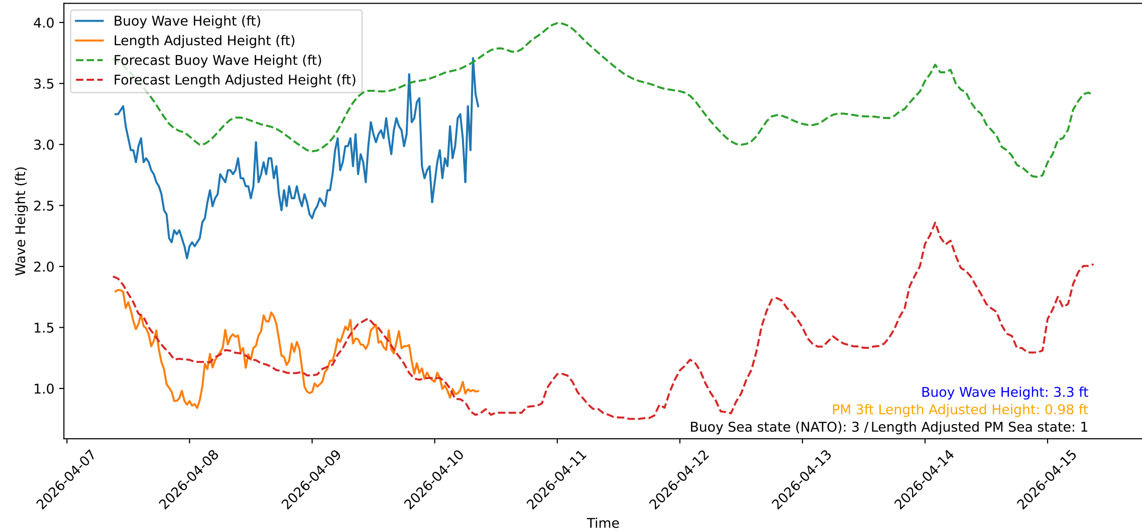
Wave Heights over Time for Red Beach at 2026-04-10 09:20:52
