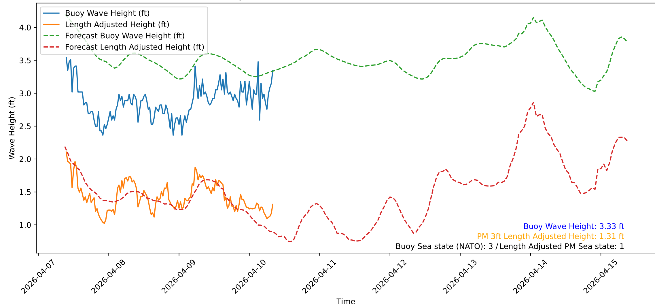
Wave Heights over Time for Green Beach at 2026-04-10 09:21:14
