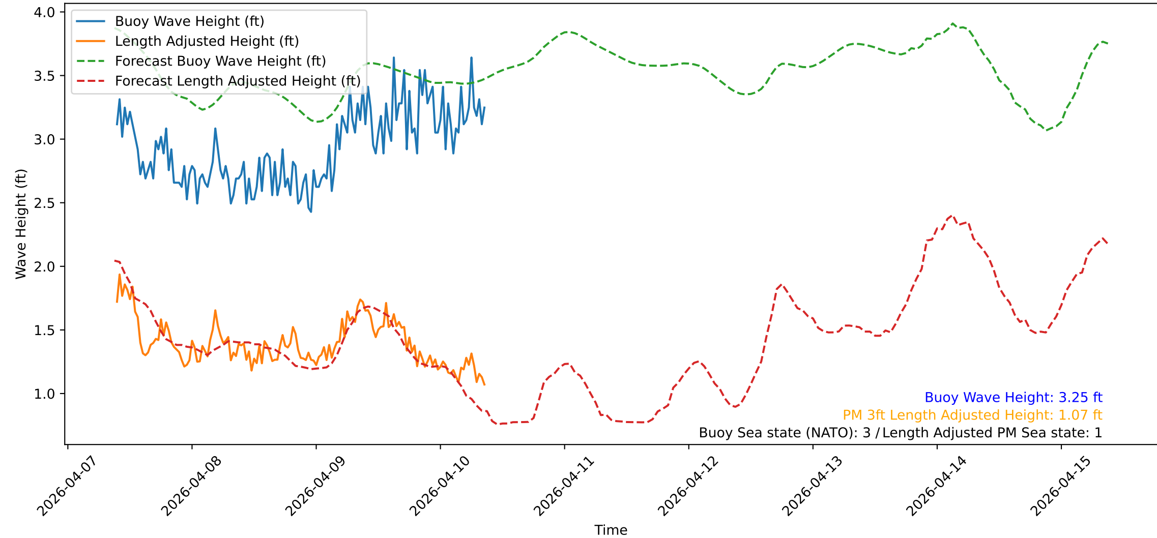
Wave Heights over Time for Oceanside Harbor at 2026-04-10 09:20:31
