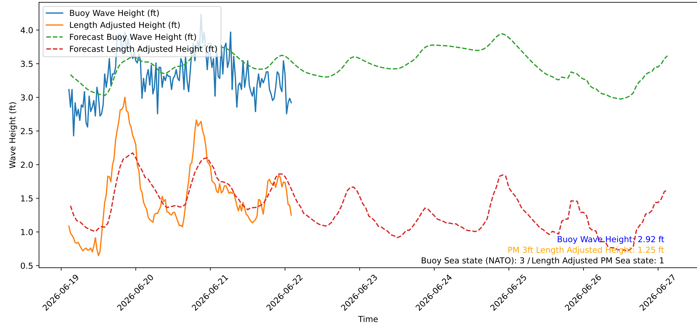
Wave Heights over Time for Green Beach at 2026-06-22 02:41:08
