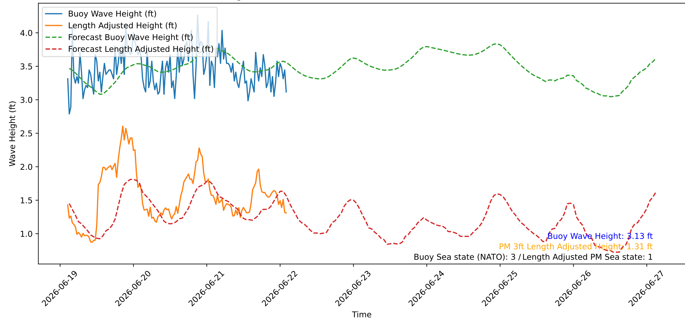
Wave Heights over Time for Oceanside Harbor at 2026-06-22 02:40:26
