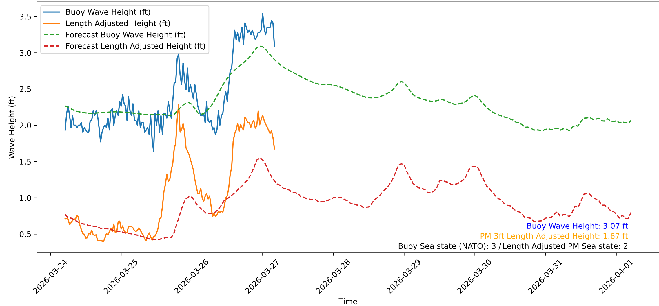
Wave Heights over Time for Green Beach at 2026-03-27 04:51:09
