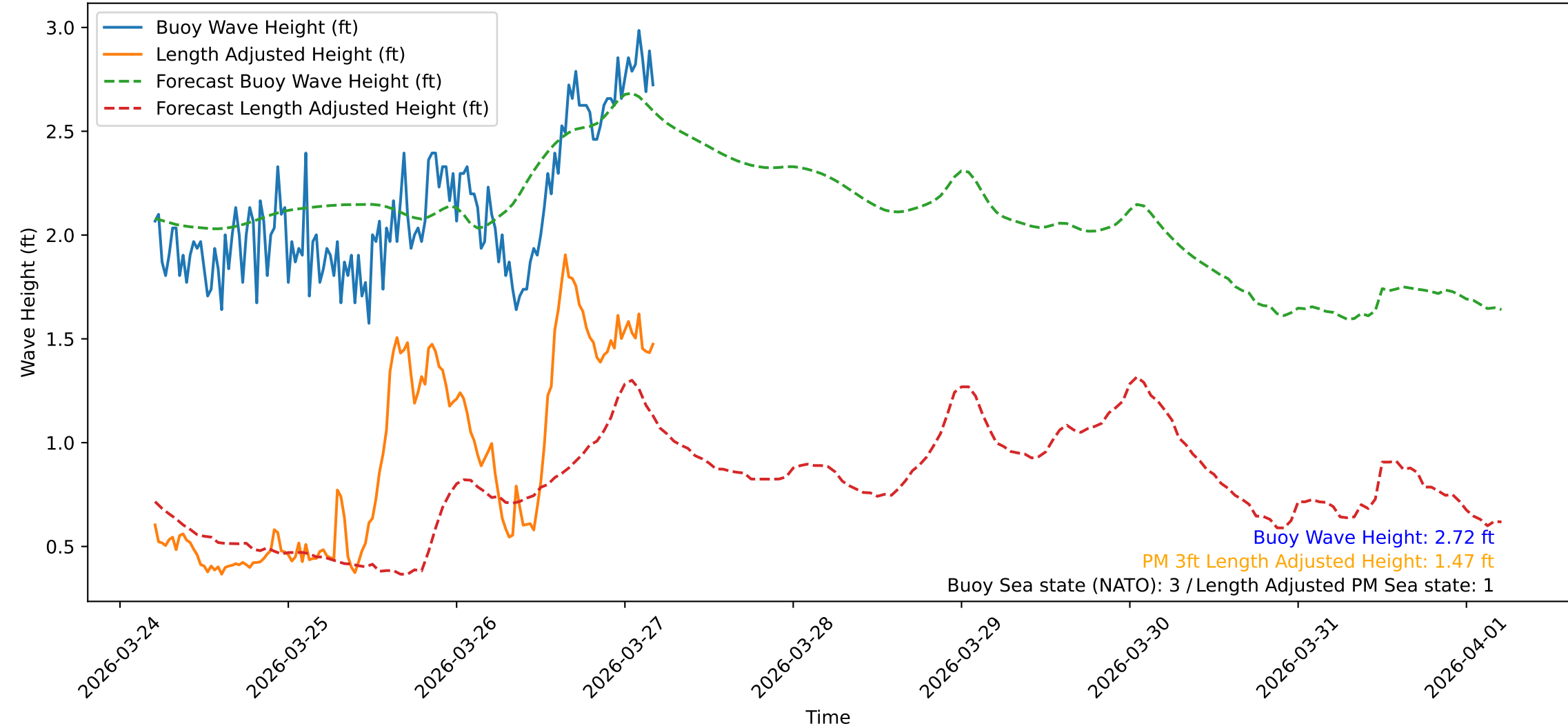
Wave Heights over Time for Red Beach at 2026-03-27 04:50:47
