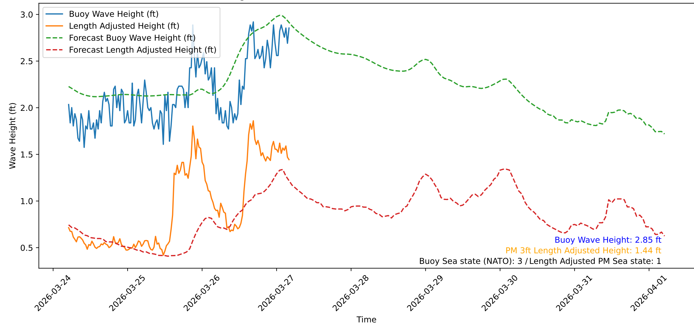
Wave Heights over Time for Oceanside Harbor at 2026-03-27 04:50:31
