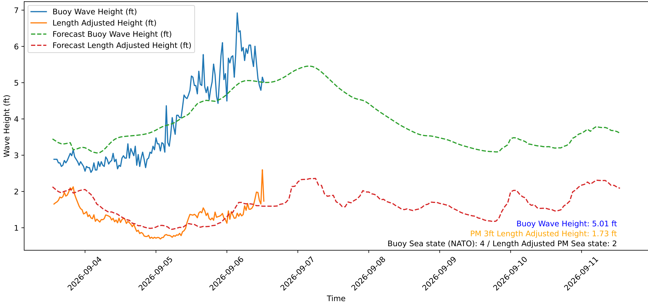
Wave Heights over Time for Red Beach at 2026-09-06 13:20:50
