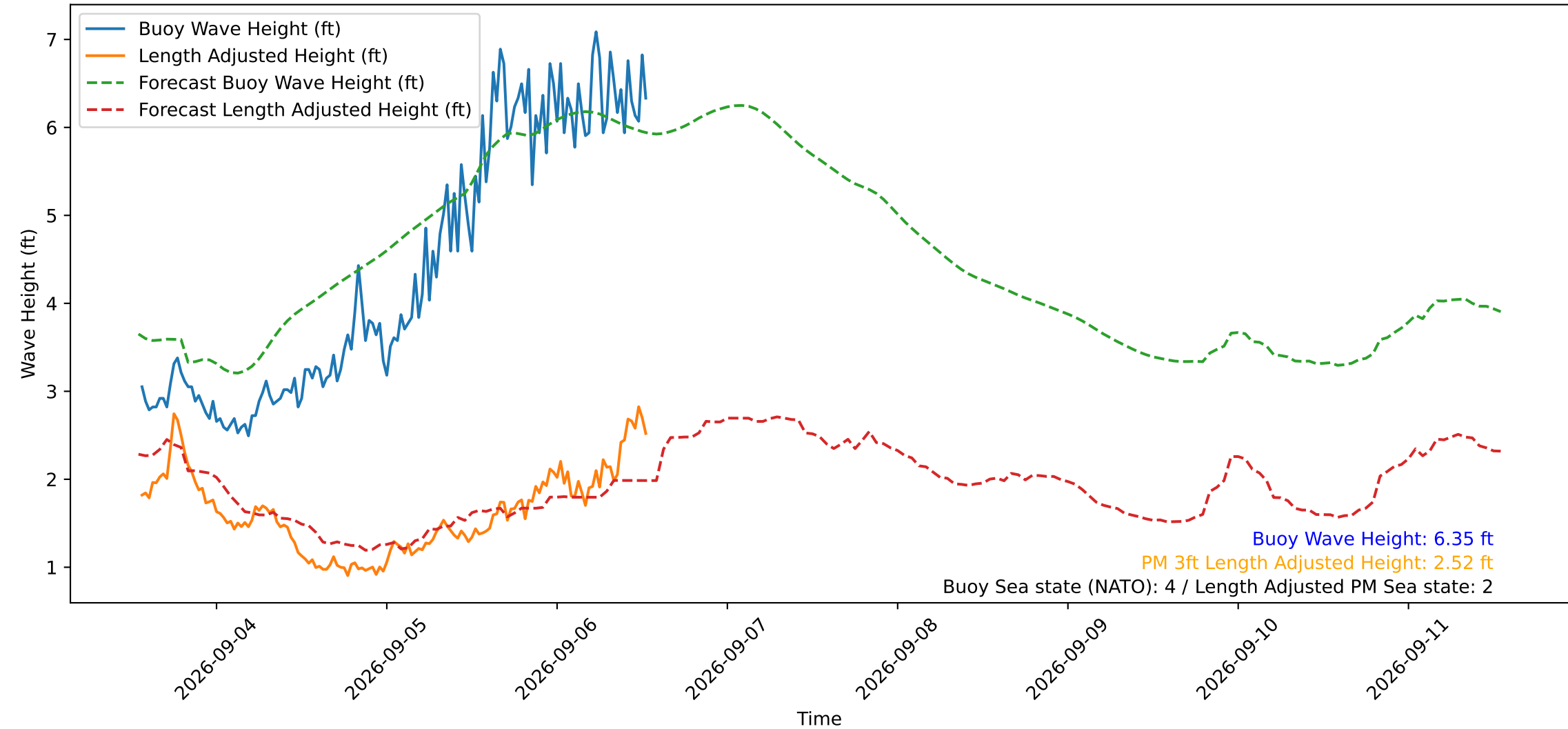
Wave Heights over Time for Green Beach at 2026-09-06 13:21:15
