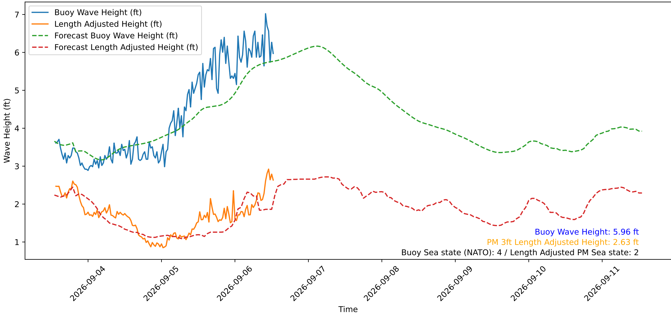
Wave Heights over Time for Oceanside Harbor at 2026-09-06 13:20:29
