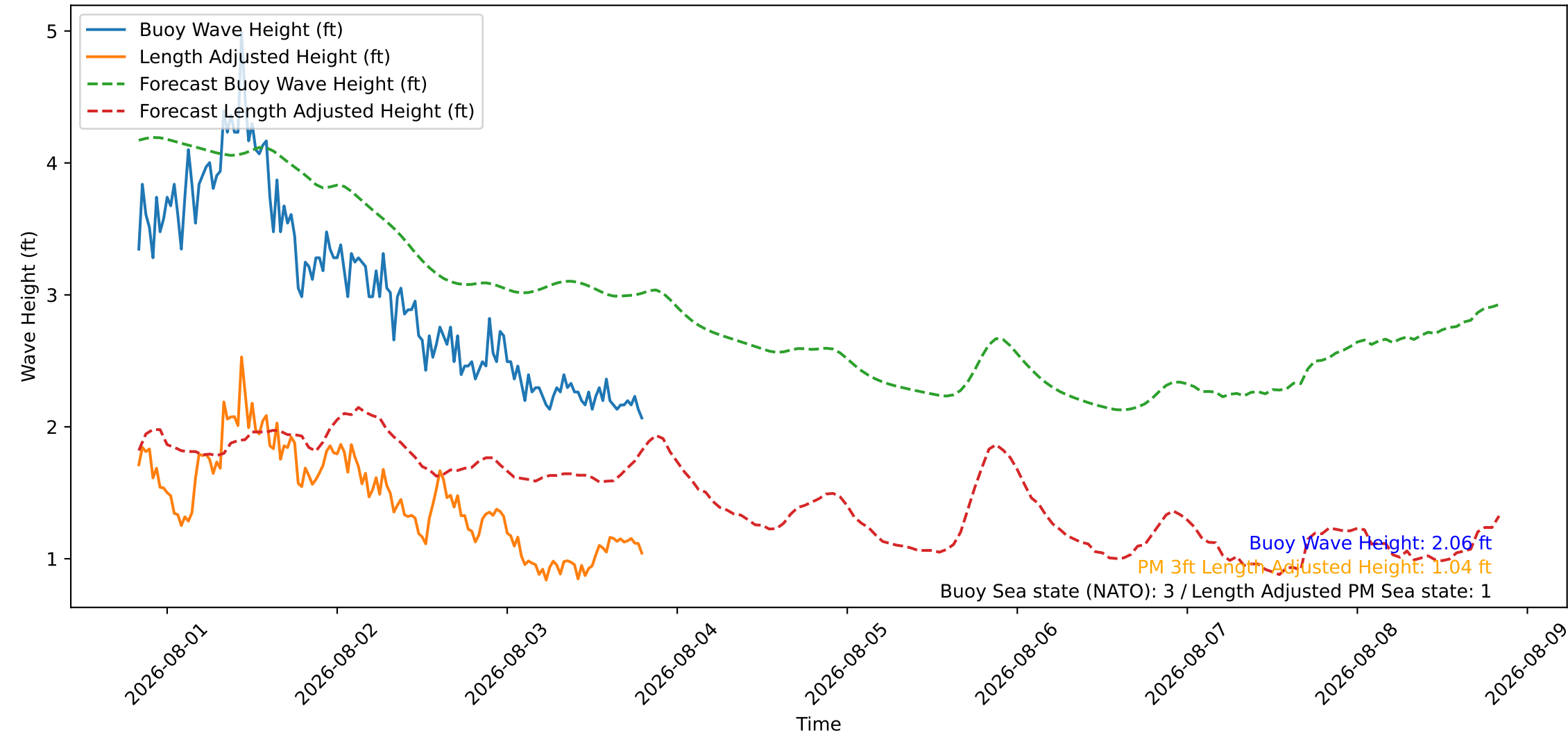
Wave Heights over Time for Green Beach at 2026-08-03 20:01:08
