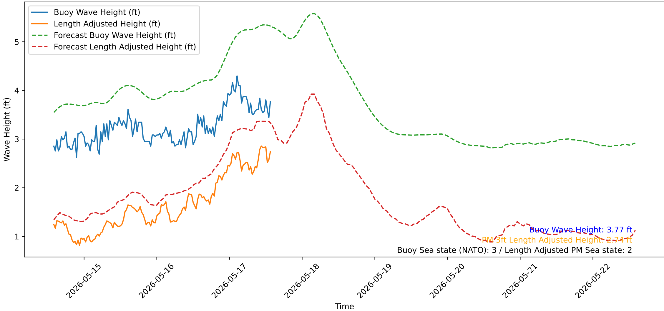
Wave Heights over Time for Oceanside Harbor at 2026-05-17 14:10:32
