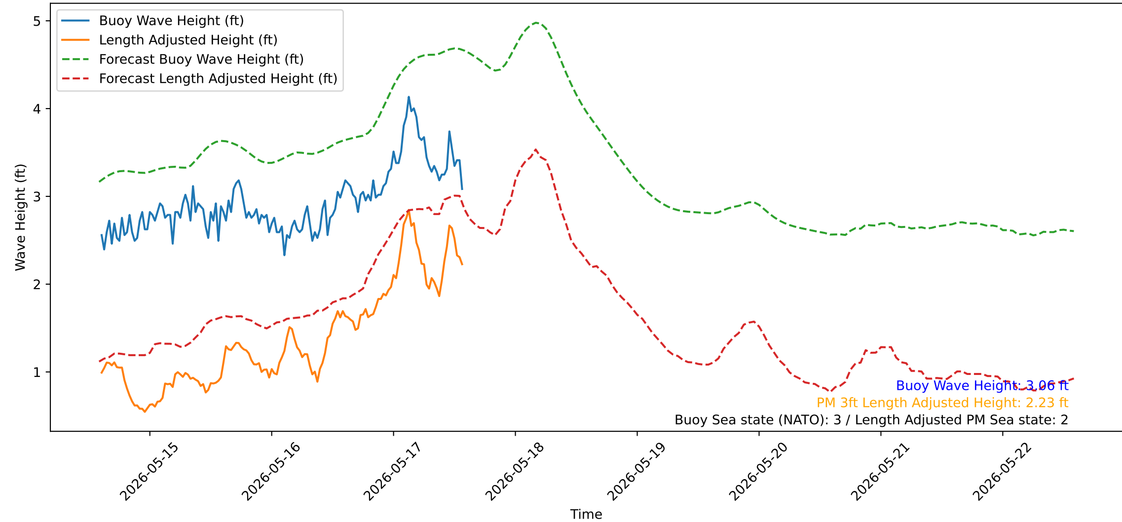
Wave Heights over Time for Red Beach at 2026-05-17 14:10:52
