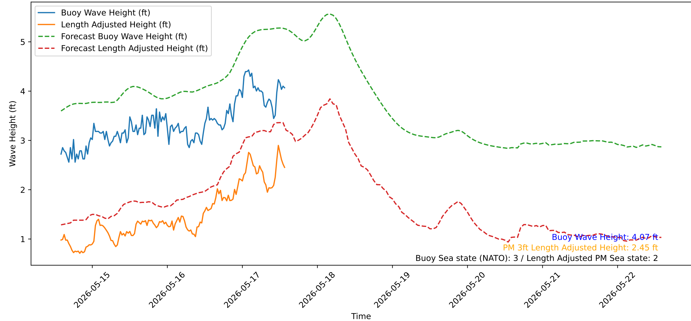
Wave Heights over Time for Green Beach at 2026-05-17 14:11:14
