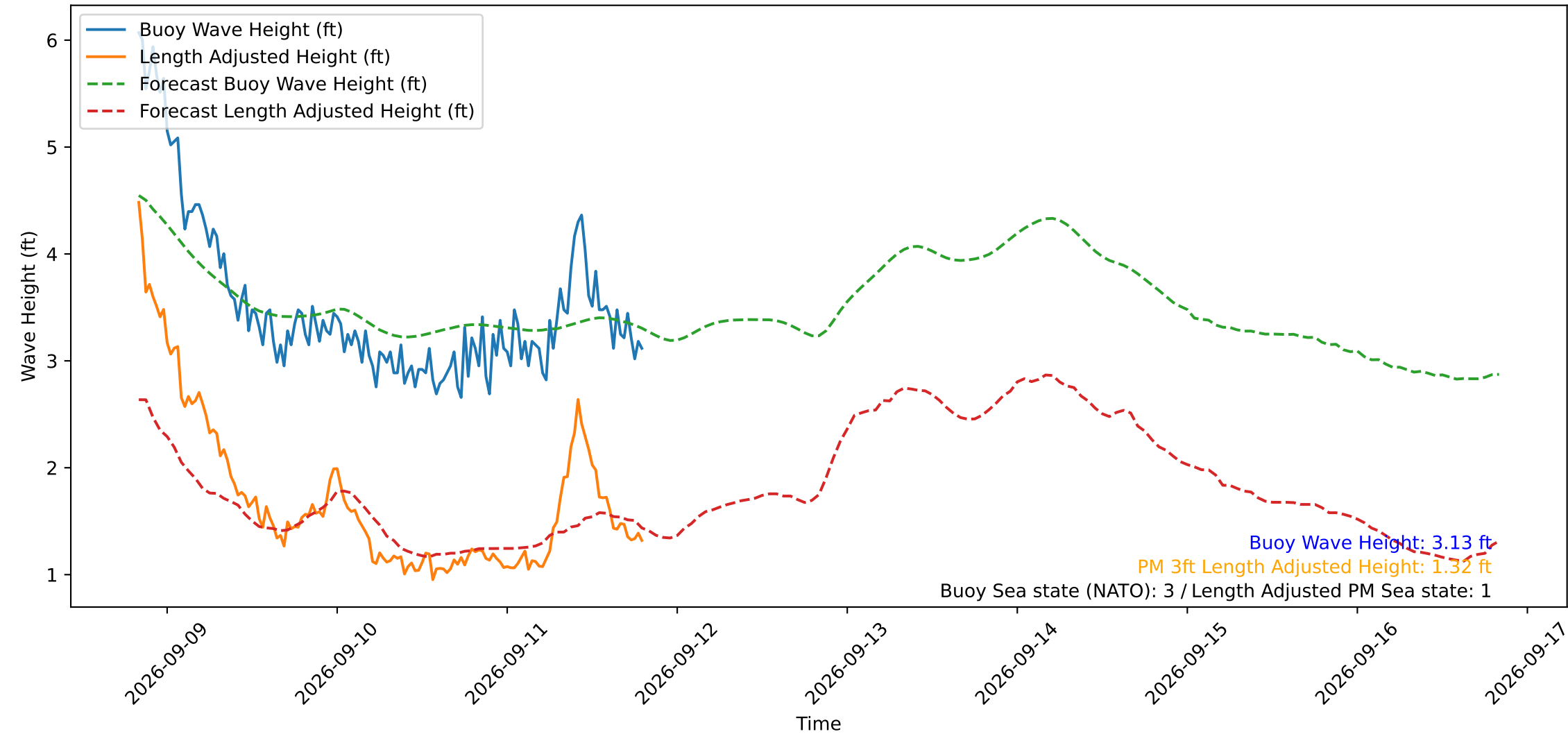
Wave Heights over Time for Oceanside Harbor at 2026-09-11 19:50:29
