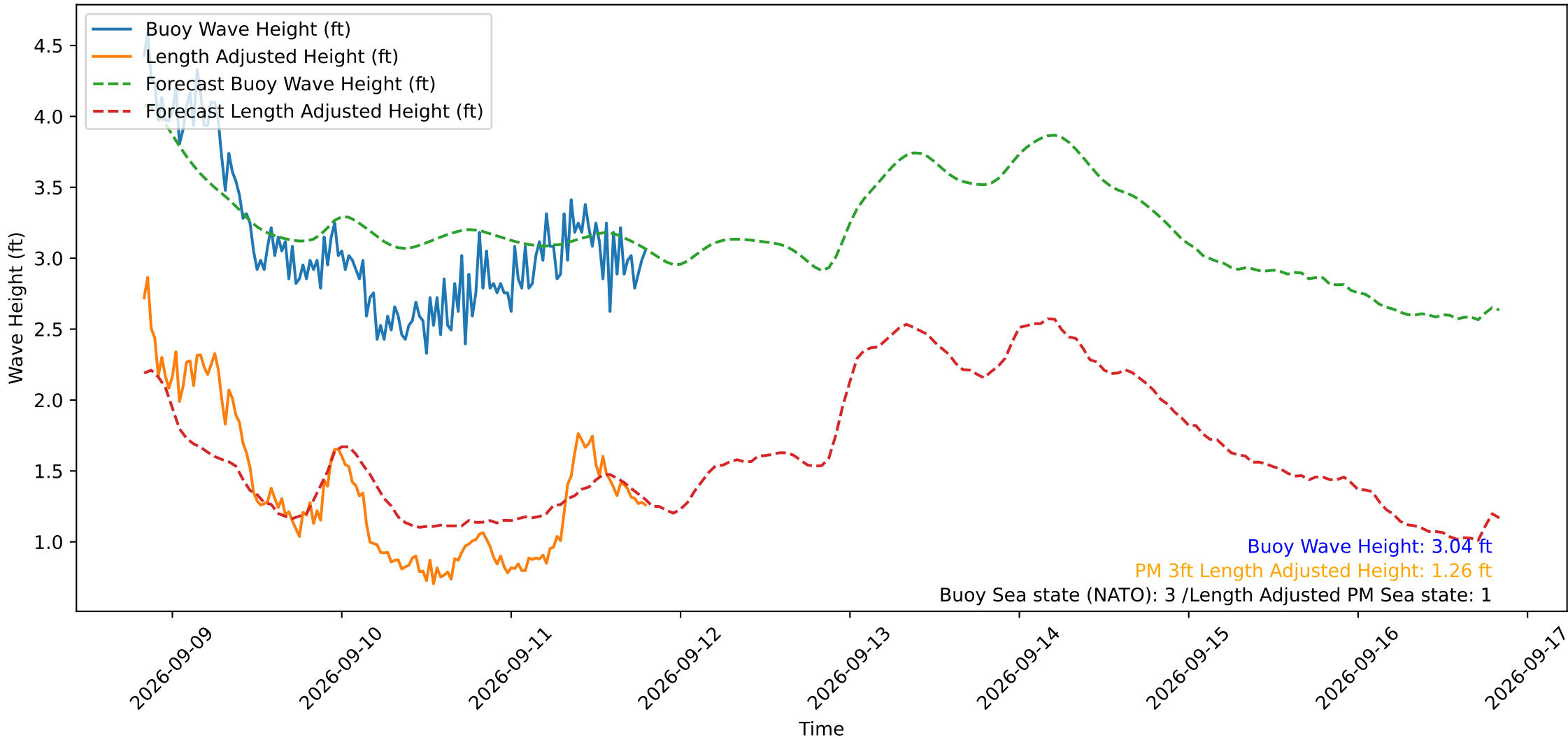
Wave Heights over Time for Red Beach at 2026-09-11 19:50:51
