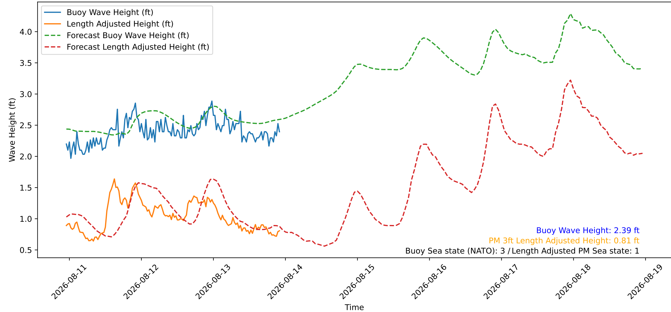
Wave Heights over Time for Red Beach at 2026-08-13 22:50:47
