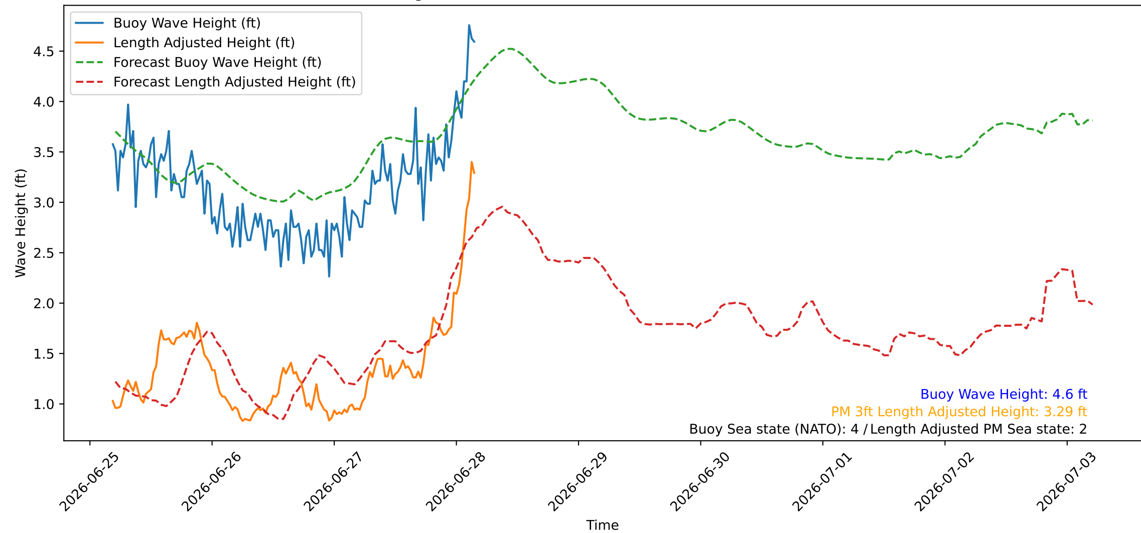
Wave Heights over Time for Green Beach at 2026-06-28 04:31:07
