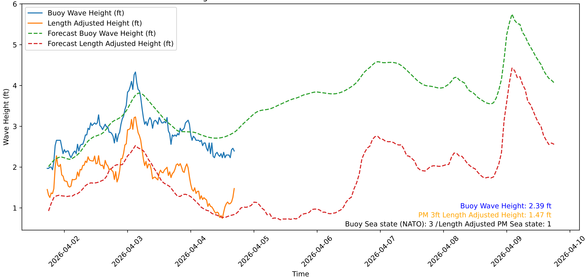
Wave Heights over Time for Green Beach at 2026-04-04 17:31:11
