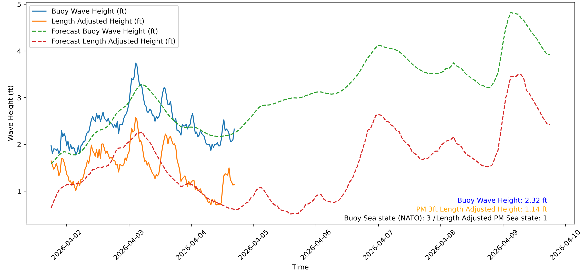
Wave Heights over Time for Red Beach at 2026-04-04 17:30:48
