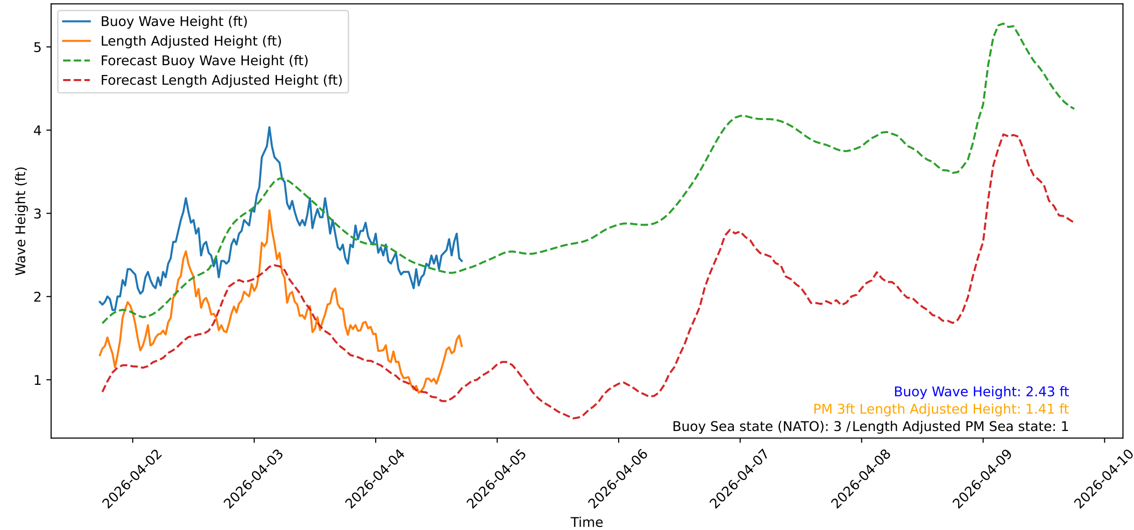
Wave Heights over Time for Oceanside Harbor at 2026-04-04 17:30:32
