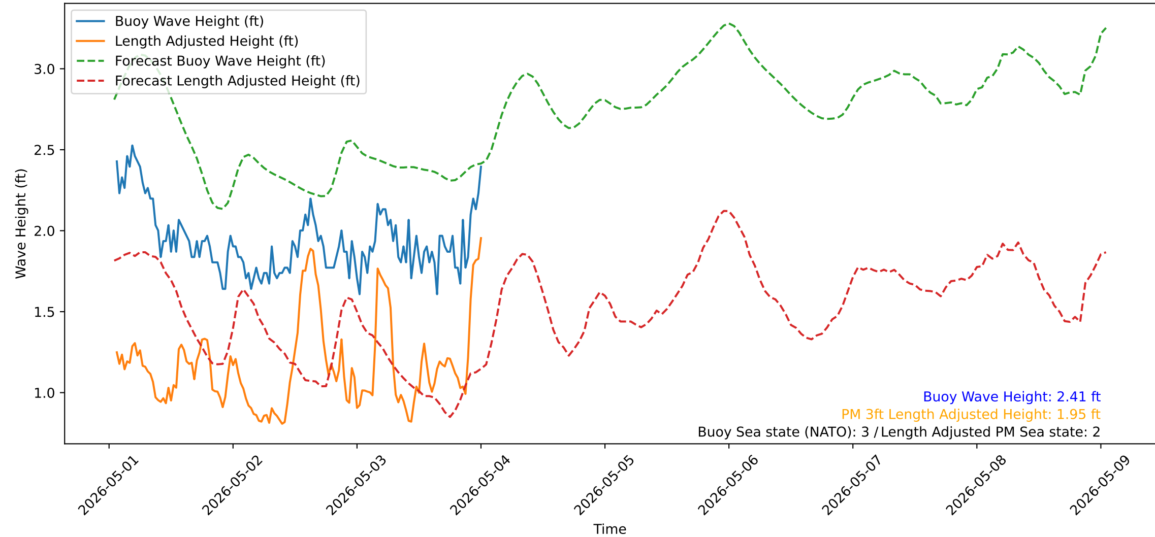
Wave Heights over Time for Red Beach at 2026-05-04 01:00:51
