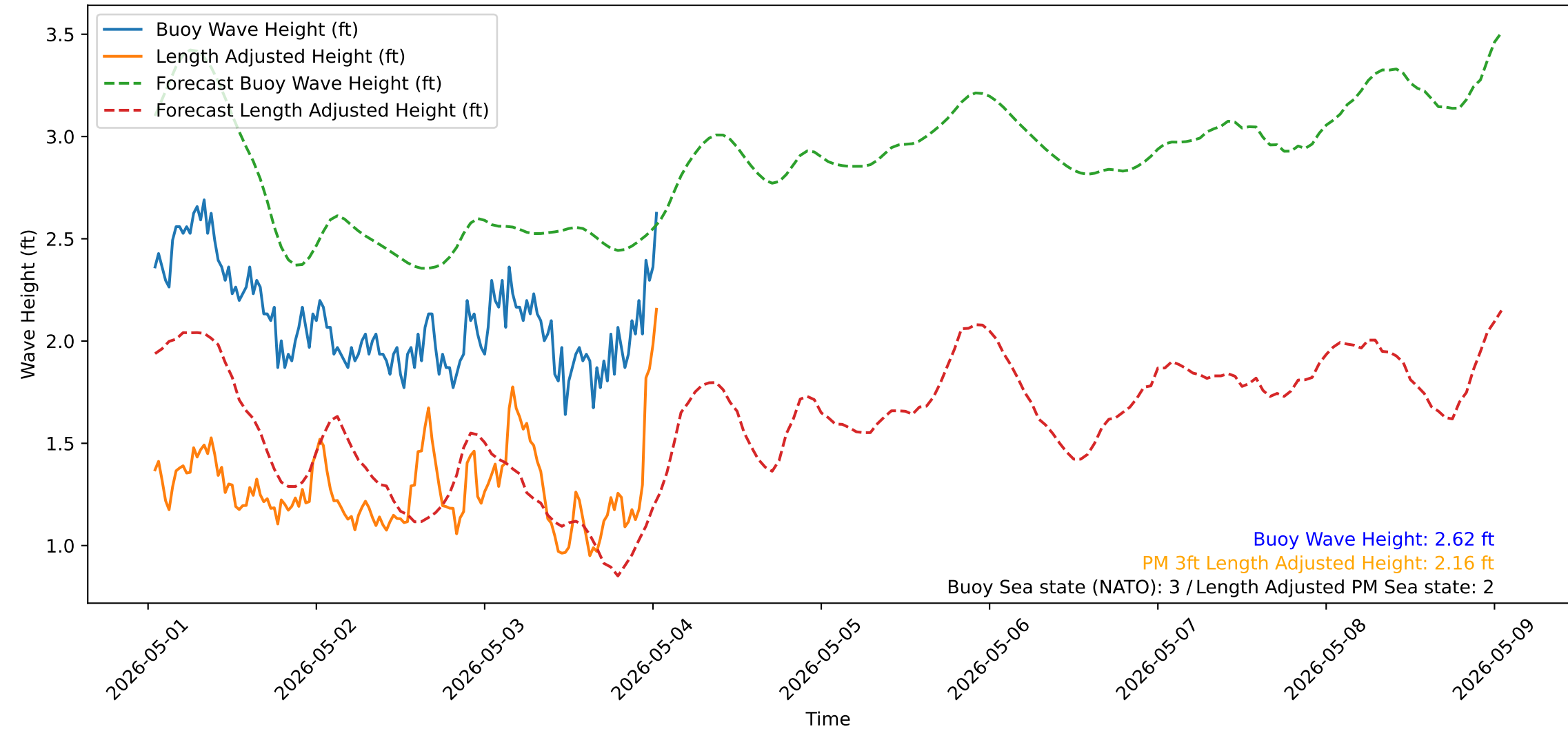
Wave Heights over Time for Oceanside Harbor at 2026-05-04 01:00:32
