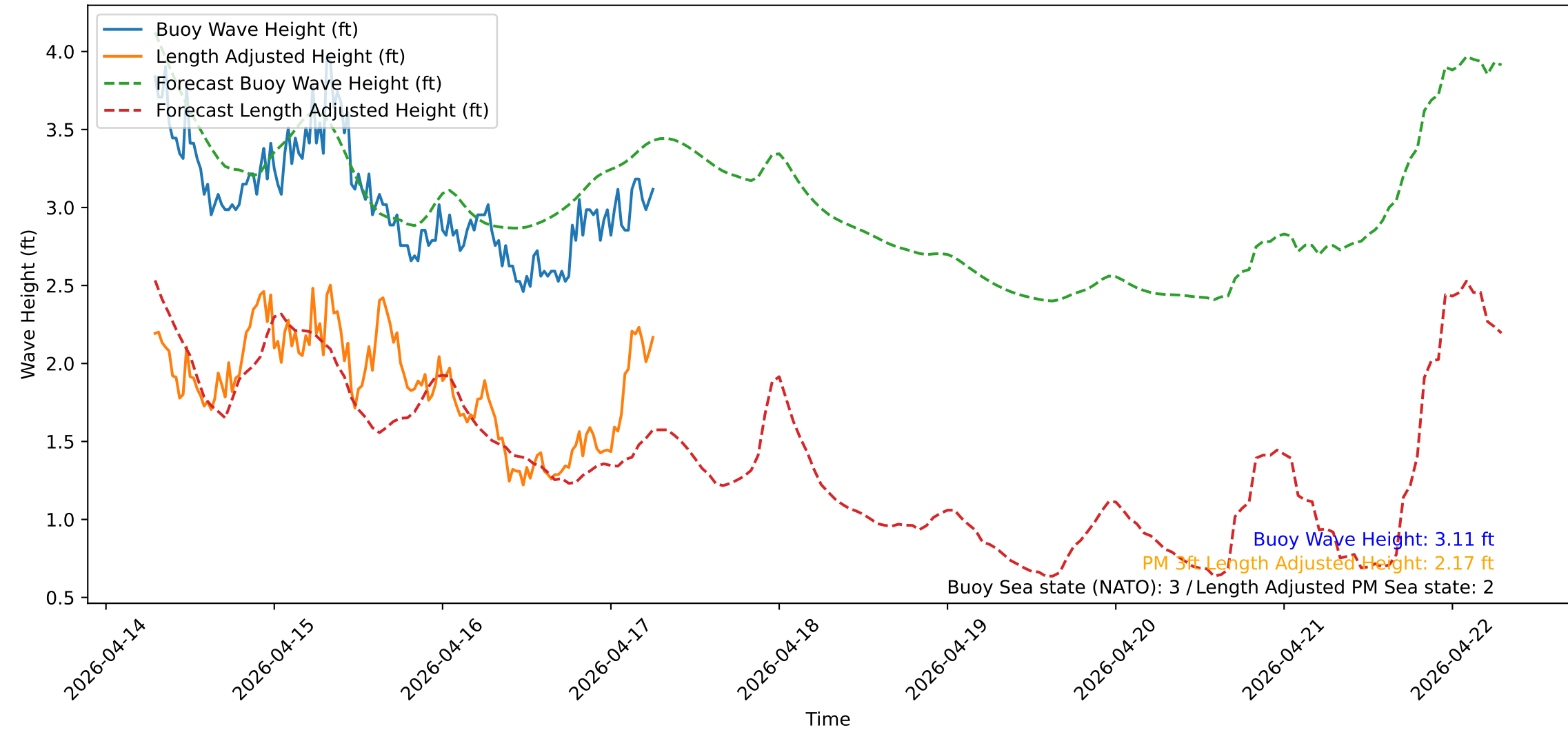
Wave Heights over Time for Green Beach at 2026-04-17 06:51:15
