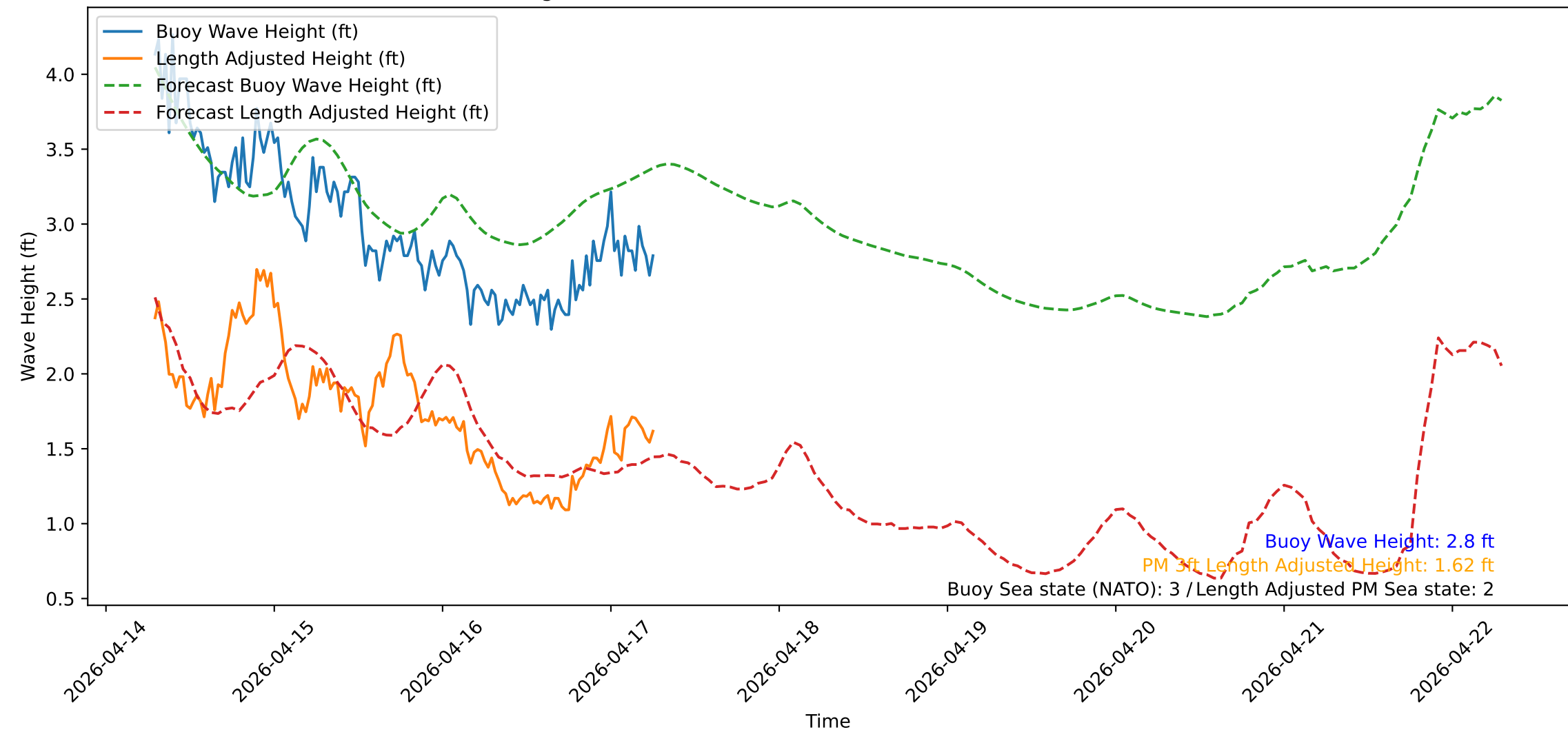
Wave Heights over Time for Oceanside Harbor at 2026-04-17 06:50:32
