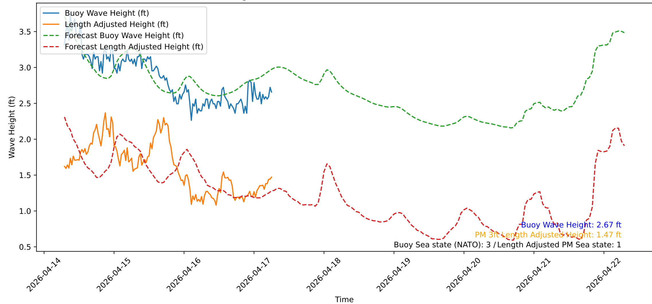
Wave Heights over Time for Red Beach at 2026-04-17 06:50:53
