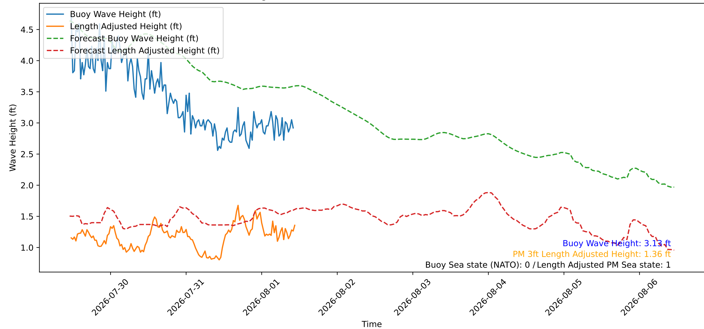
Wave Heights over Time for Red Beach at 2026-08-01 11:10:46
