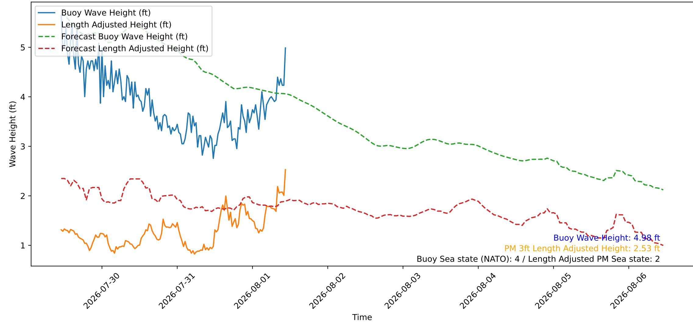
Wave Heights over Time for Green Beach at 2026-08-01 11:11:09
