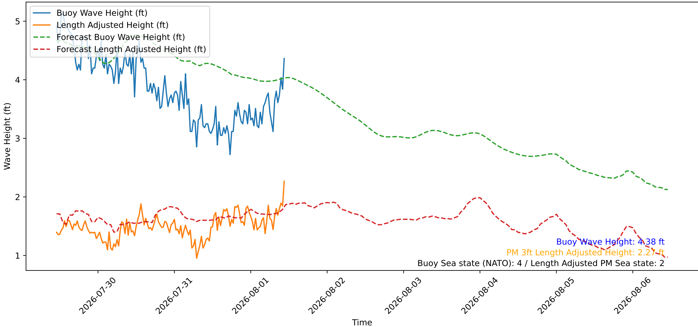
Wave Heights over Time for Oceanside Harbor at 2026-08-01 11:10:26
