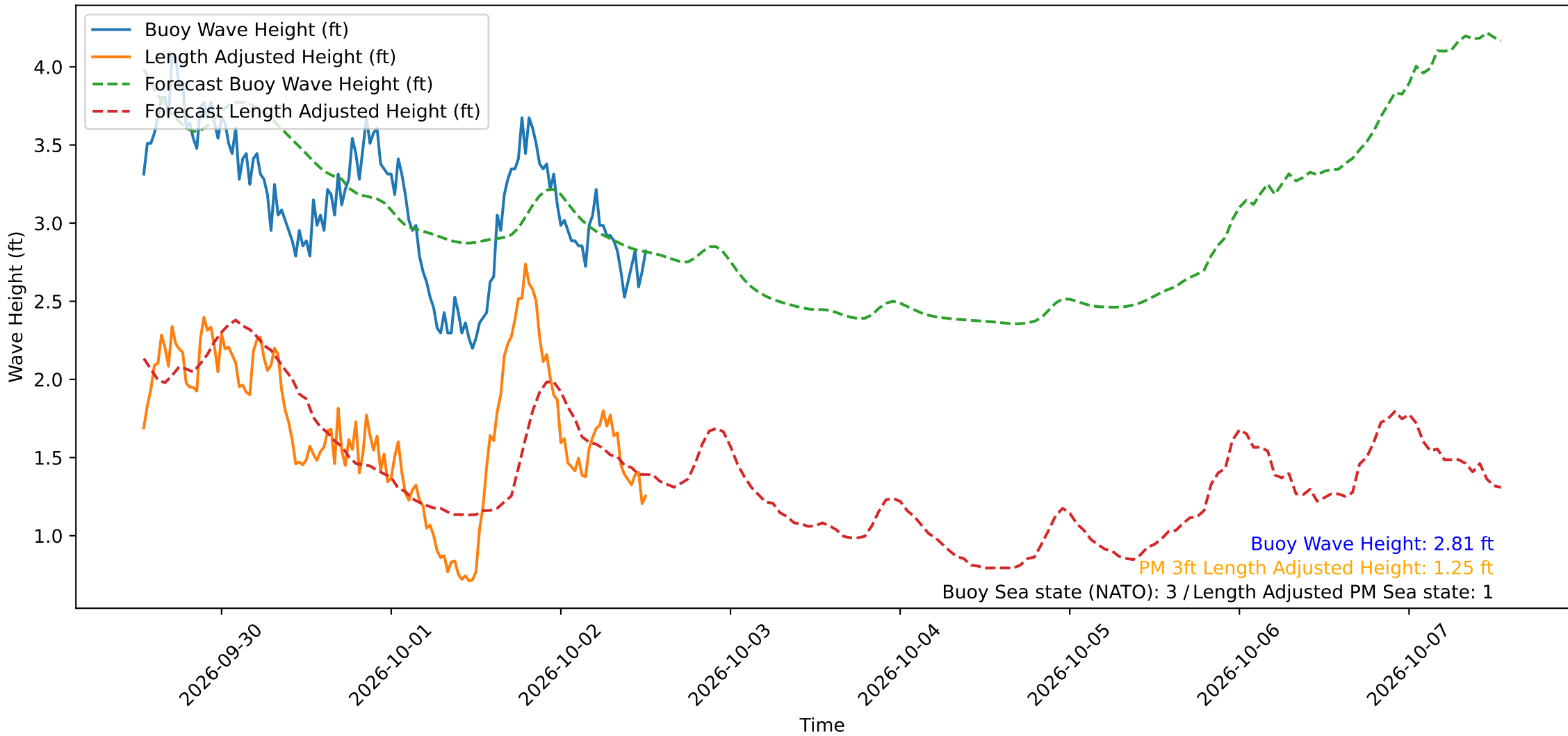
Wave Heights over Time for Green Beach at 2026-10-02 12:51:15
