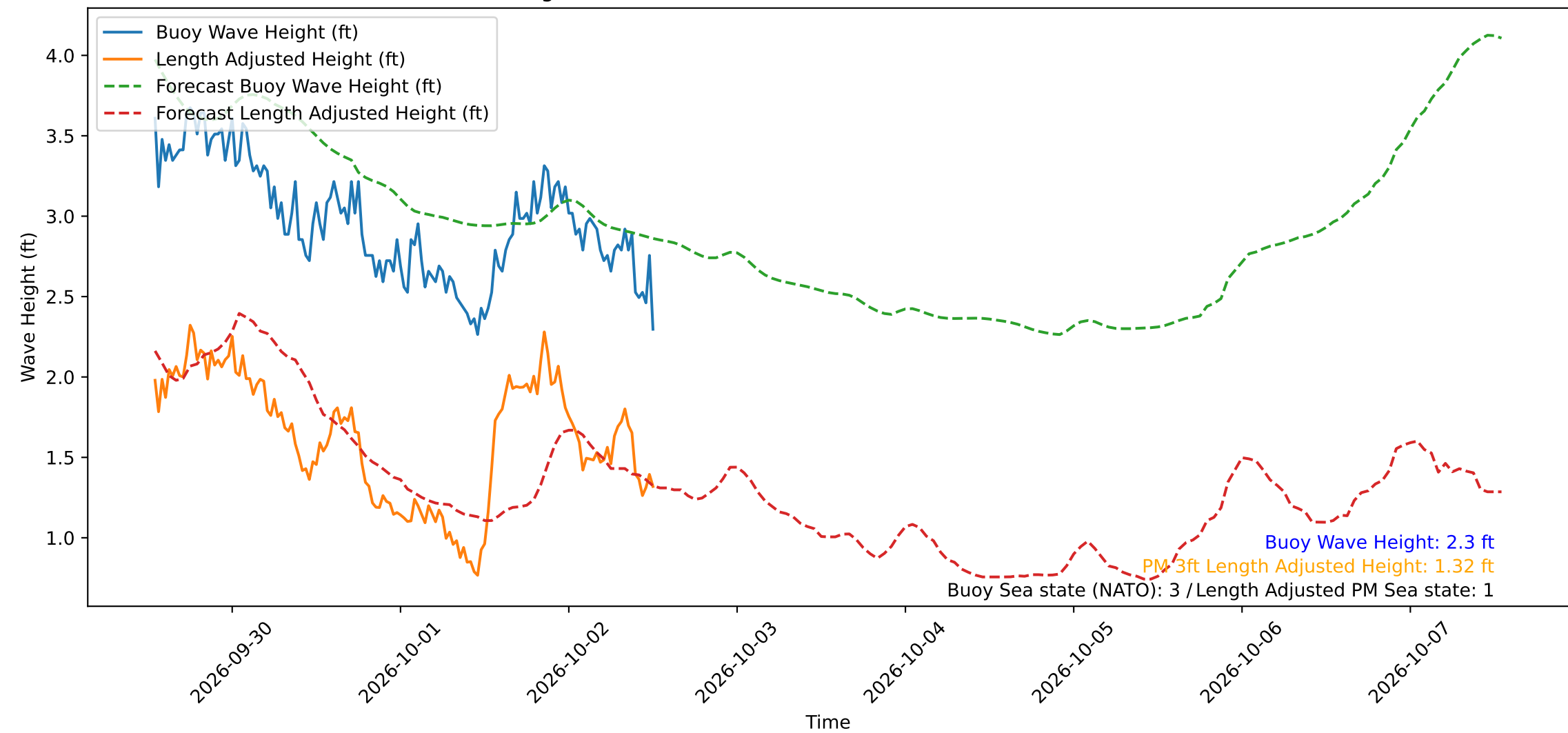
Wave Heights over Time for Oceanside Harbor at 2026-10-02 12:50:30
