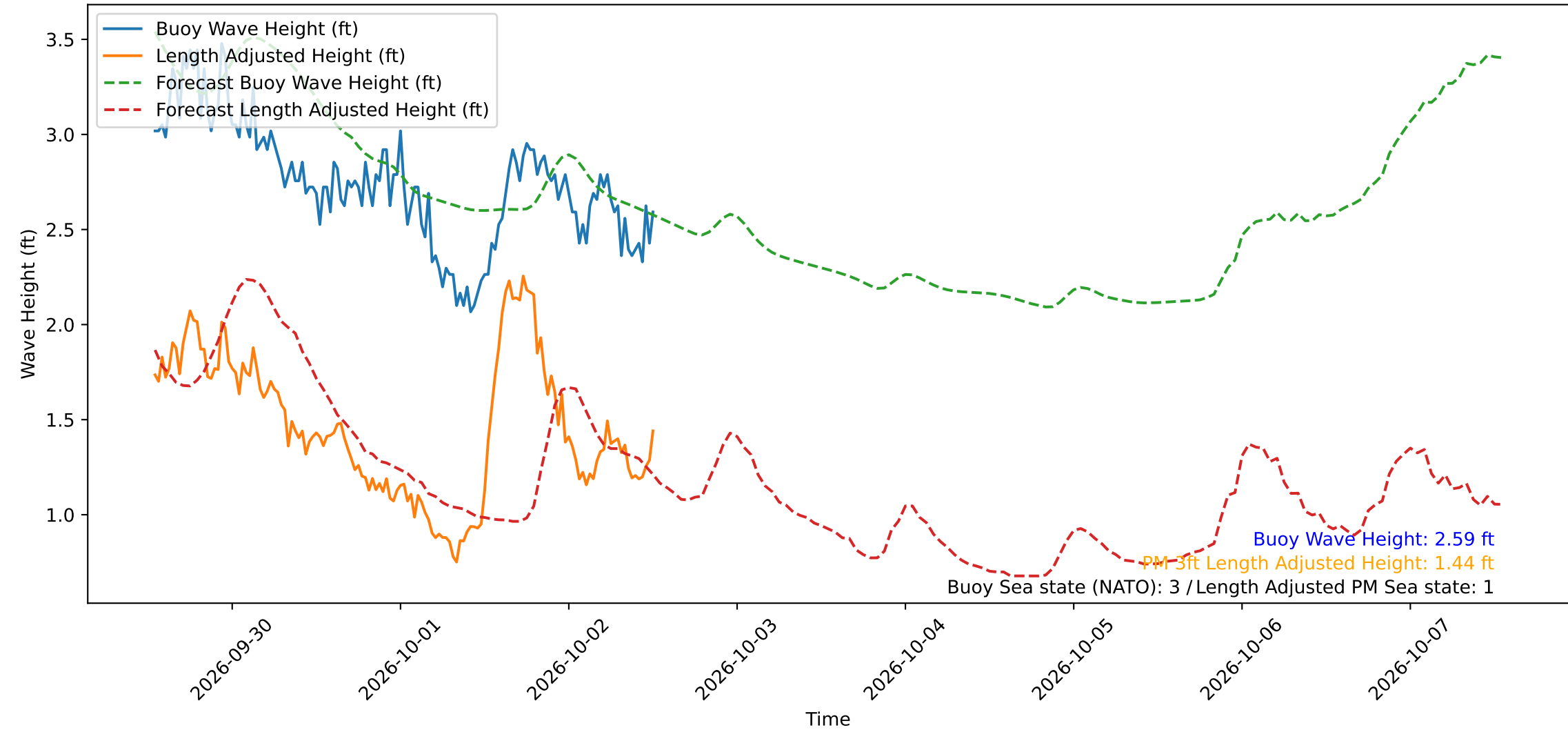
Wave Heights over Time for Red Beach at 2026-10-02 12:50:51
