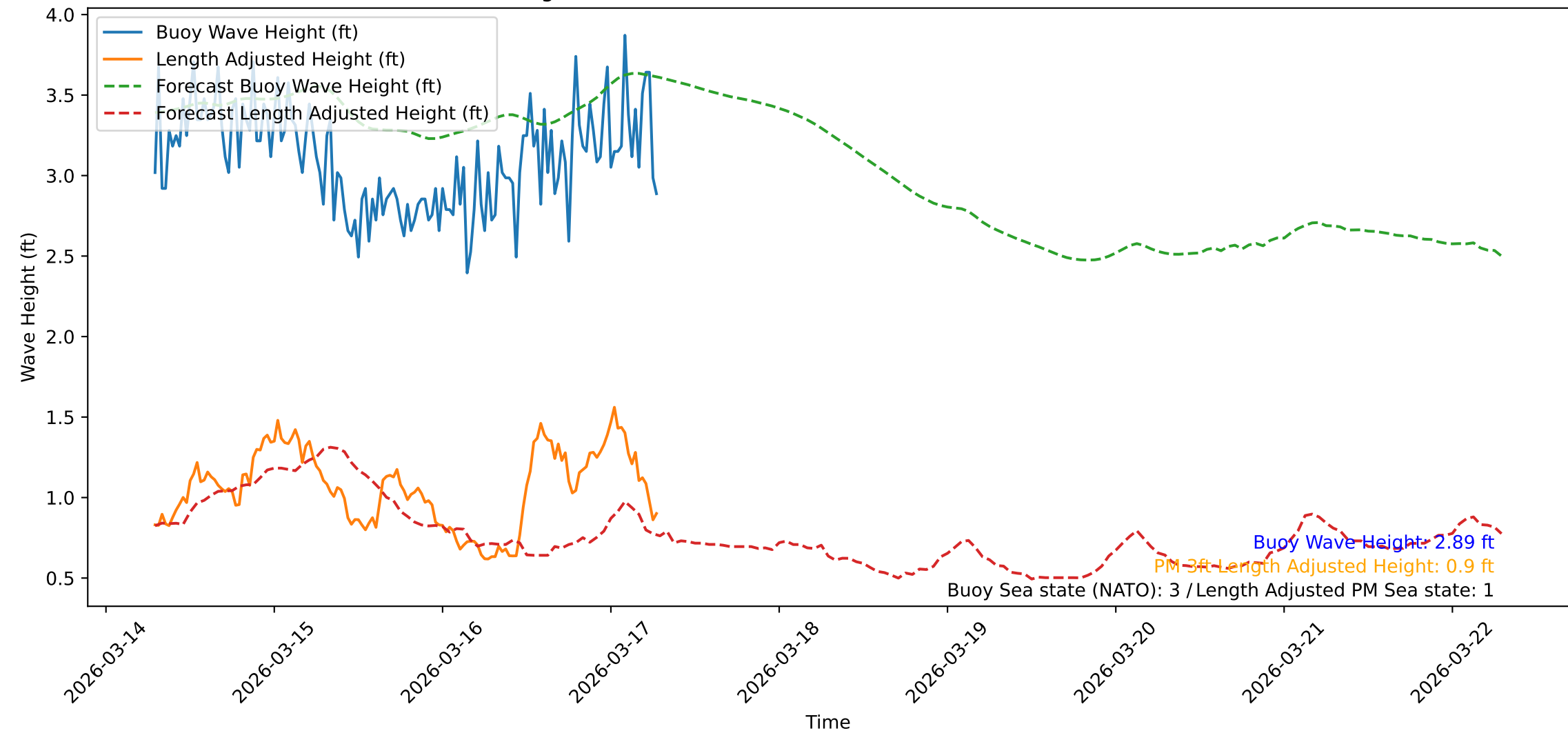
Wave Heights over Time for Oceanside Harbor at 2026-03-17 07:10:49
