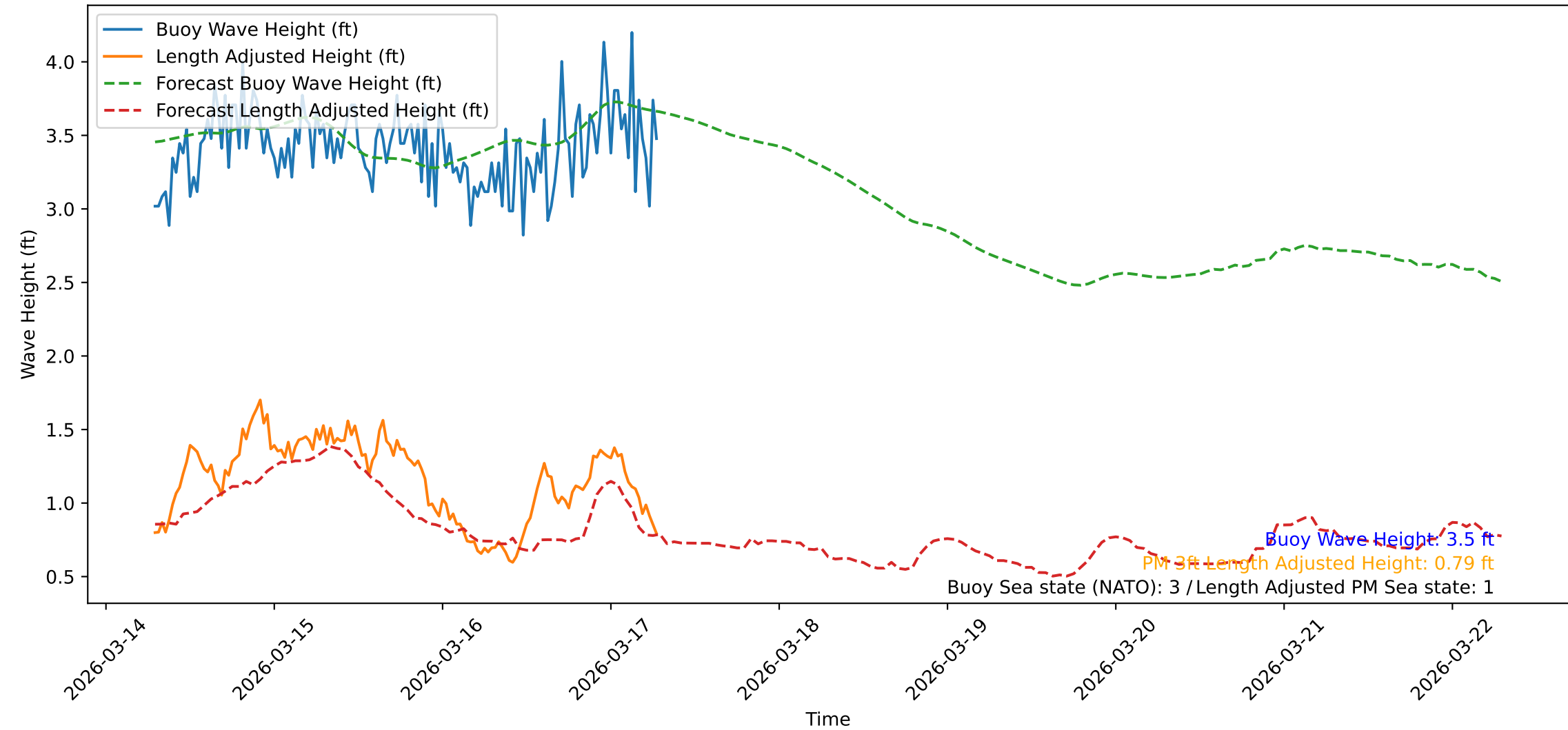
Wave Heights over Time for Green Beach at 2026-03-17 07:11:53
