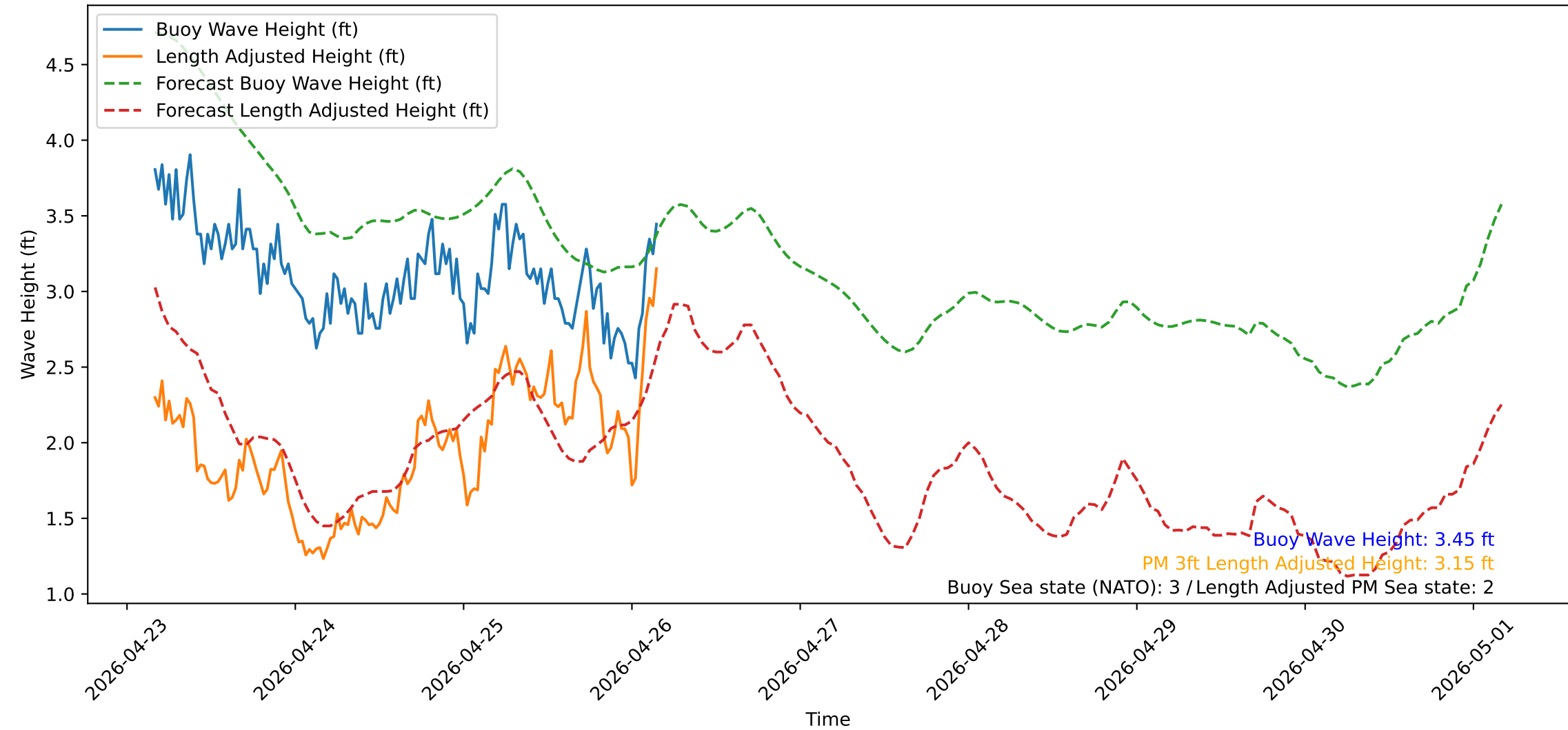
Wave Heights over Time for Green Beach at 2026-04-26 04:11:12
