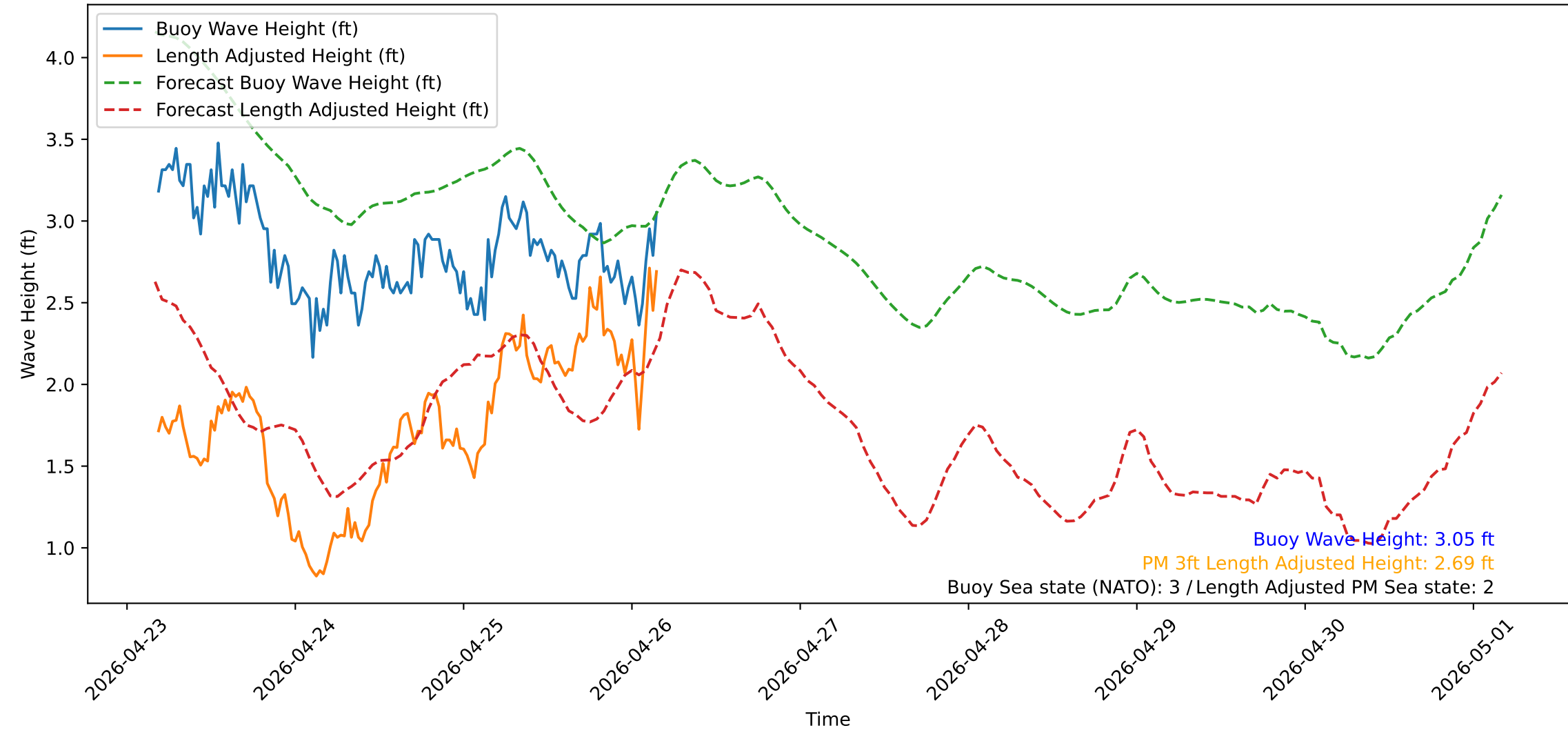
Wave Heights over Time for Red Beach at 2026-04-26 04:10:50
