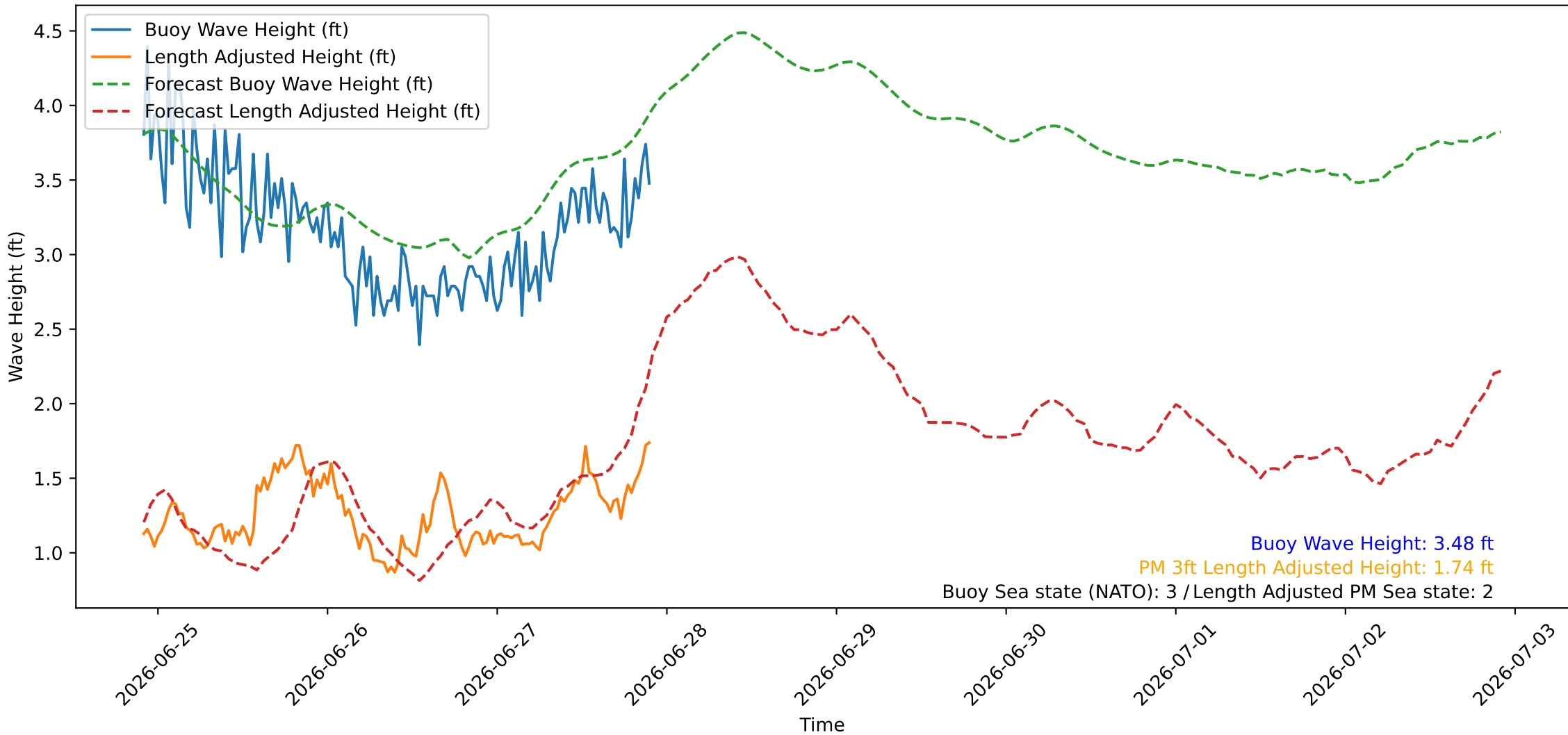
Wave Heights over Time for Oceanside Harbor at 2026-06-27 22:10:27
