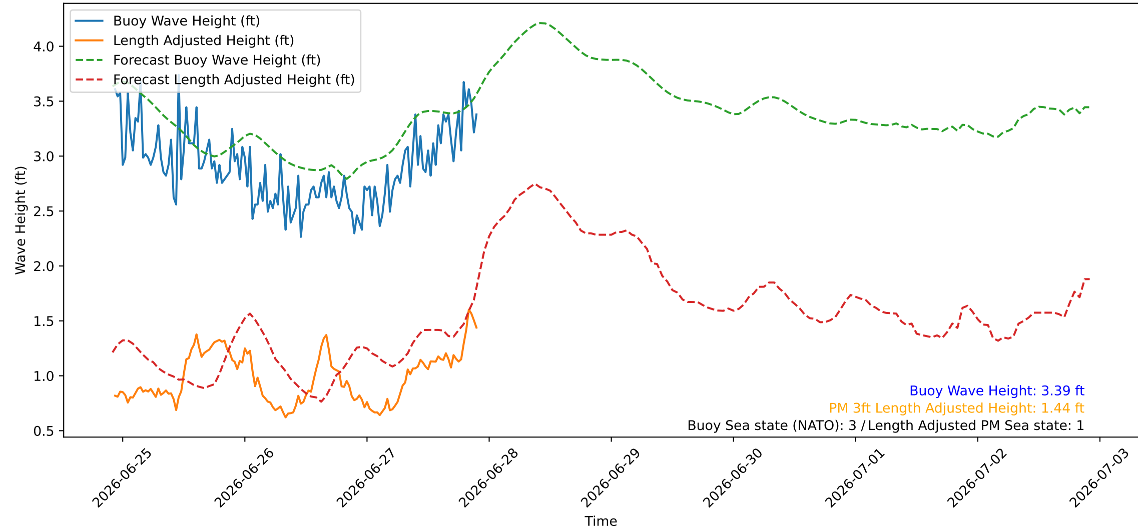
Wave Heights over Time for Red Beach at 2026-06-27 22:10:46
