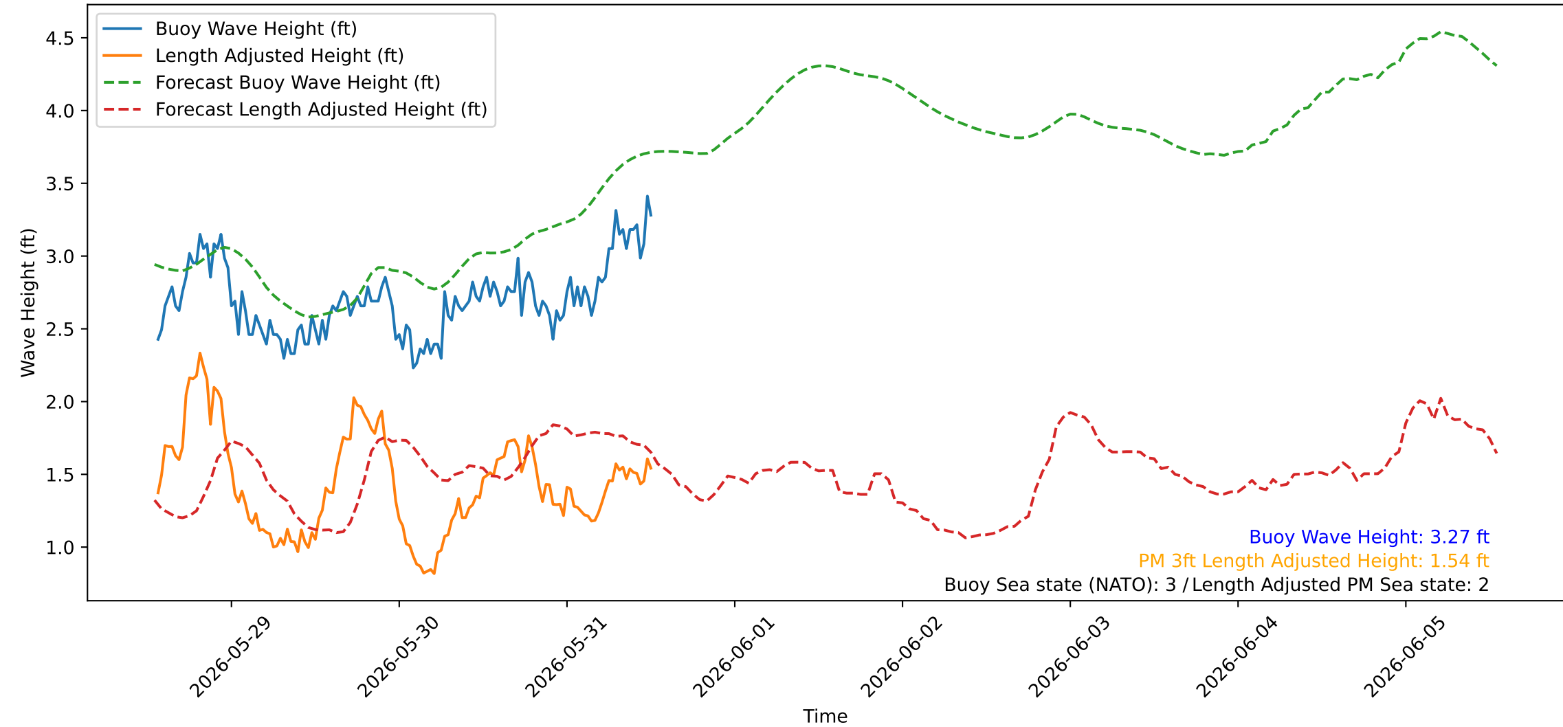
Wave Heights over Time for Red Beach at 2026-05-31 13:10:45
