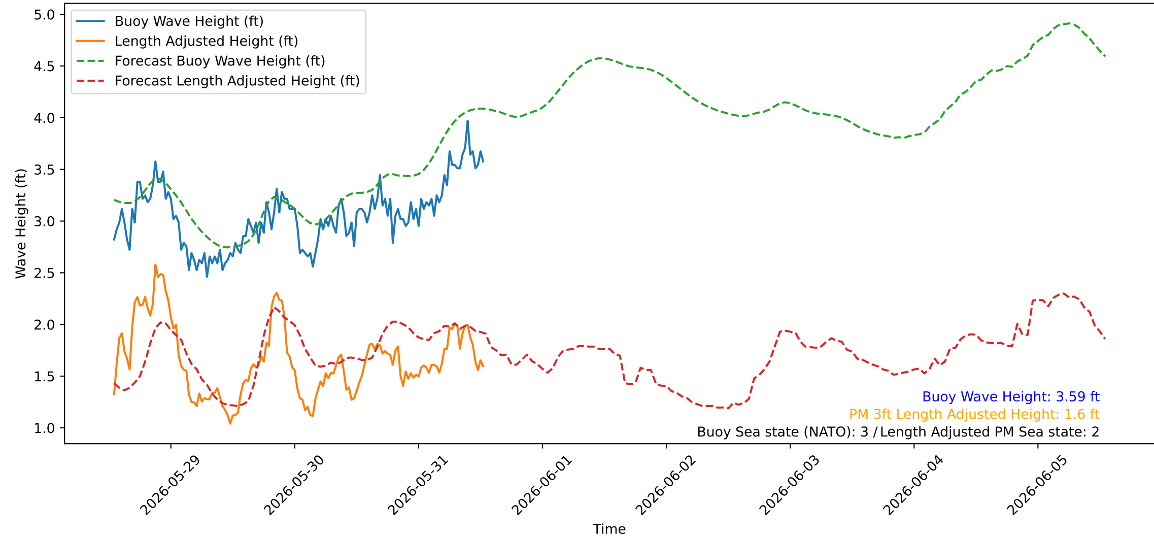
Wave Heights over Time for Green Beach at 2026-05-31 13:11:07
