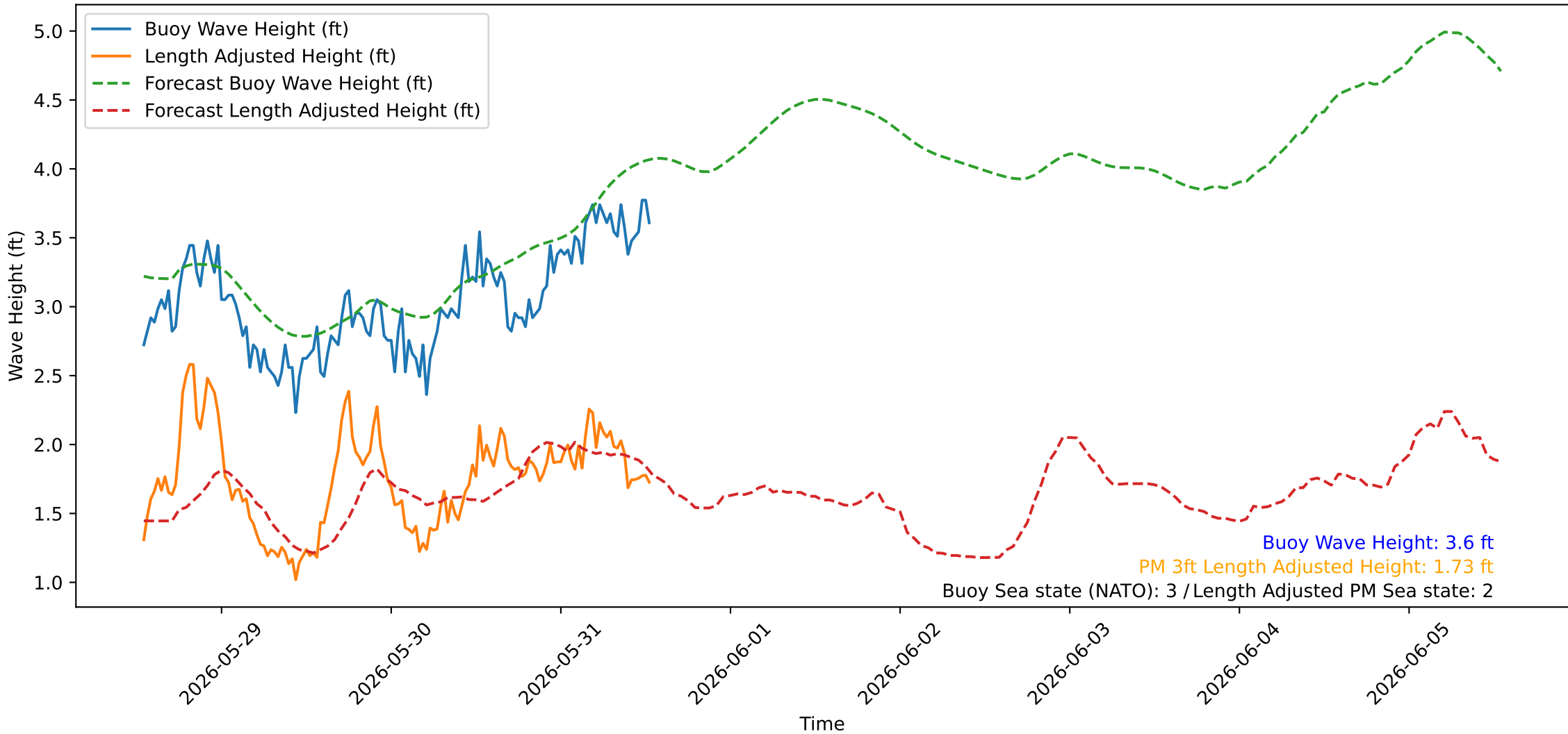
Wave Heights over Time for Oceanside Harbor at 2026-05-31 13:10:26
