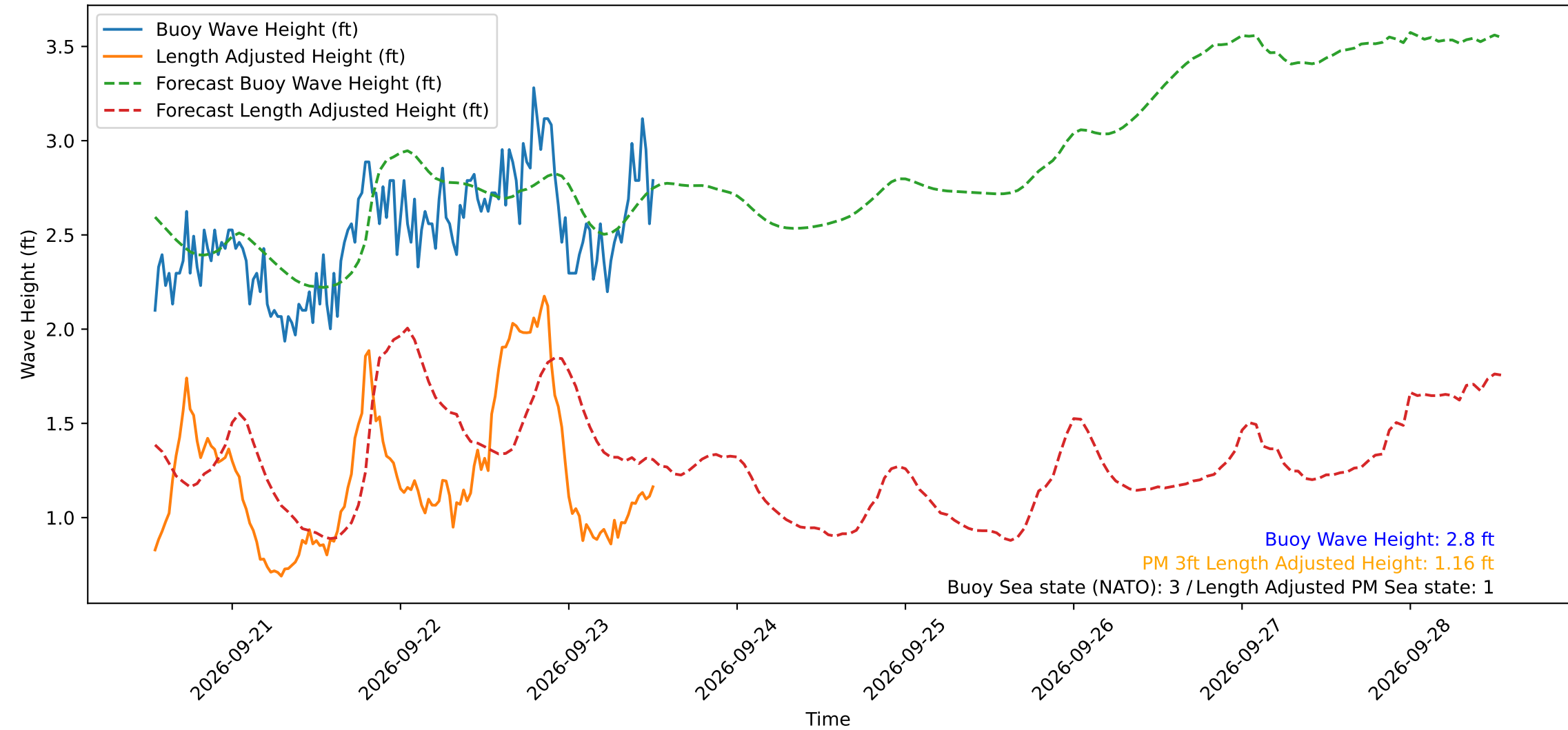
Wave Heights over Time for Red Beach at 2026-09-23 12:50:50
