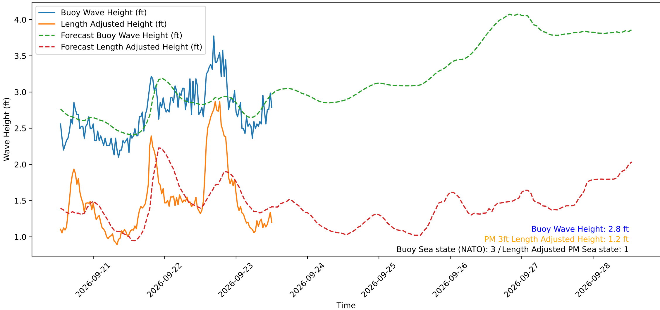
Wave Heights over Time for Oceanside Harbor at 2026-09-23 12:50:29
