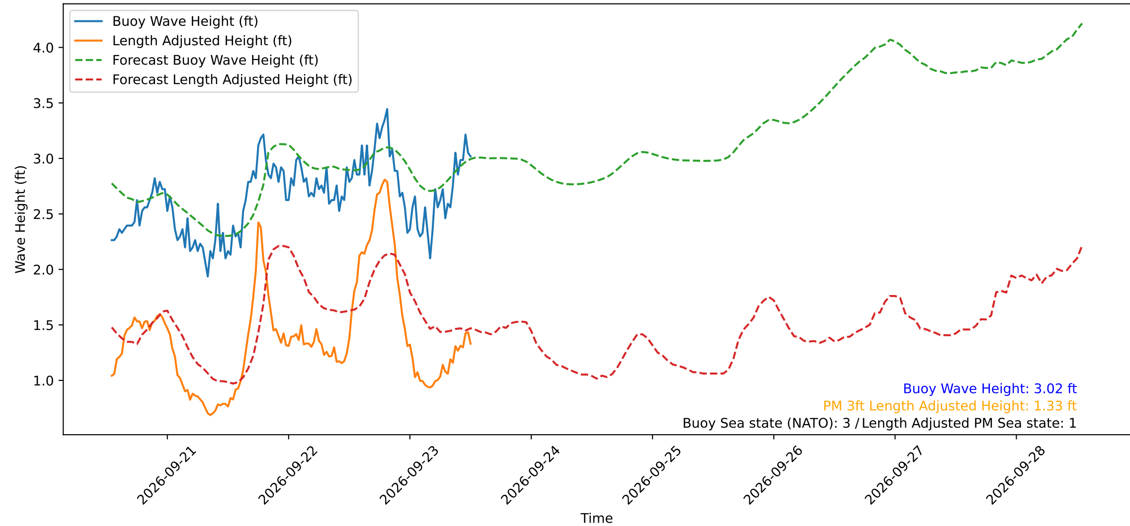
Wave Heights over Time for Green Beach at 2026-09-23 12:51:14
