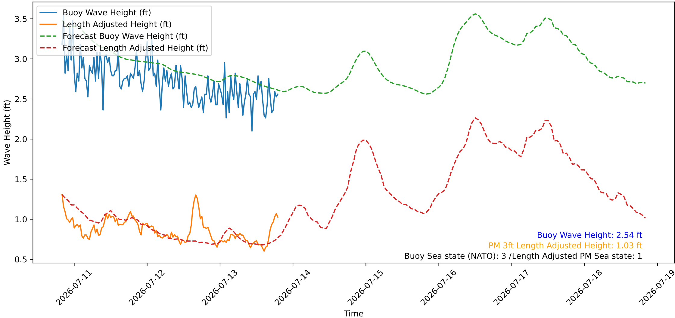
Wave Heights over Time for Oceanside Harbor at 2026-07-13 20:00:26
