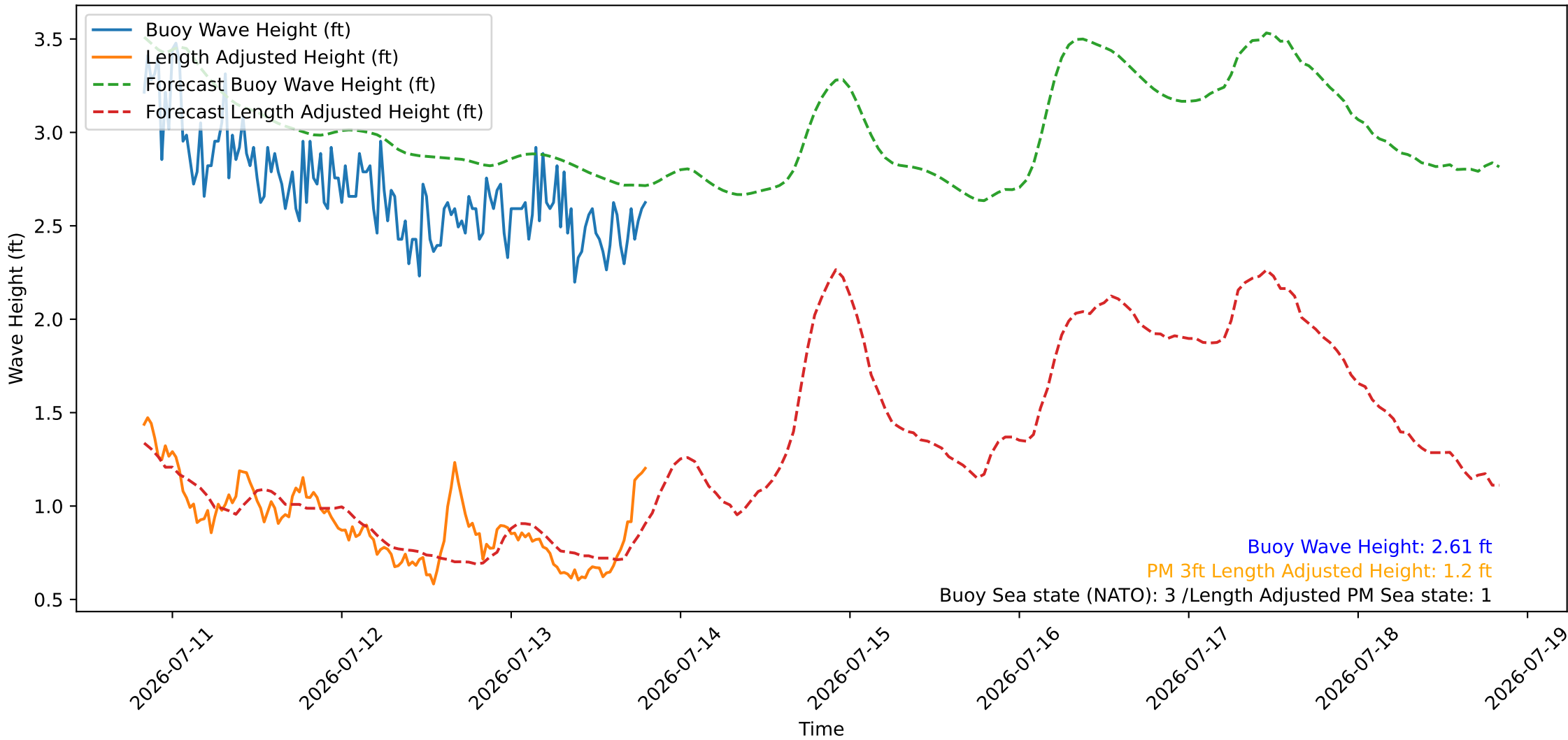
Wave Heights over Time for Green Beach at 2026-07-13 20:01:07
