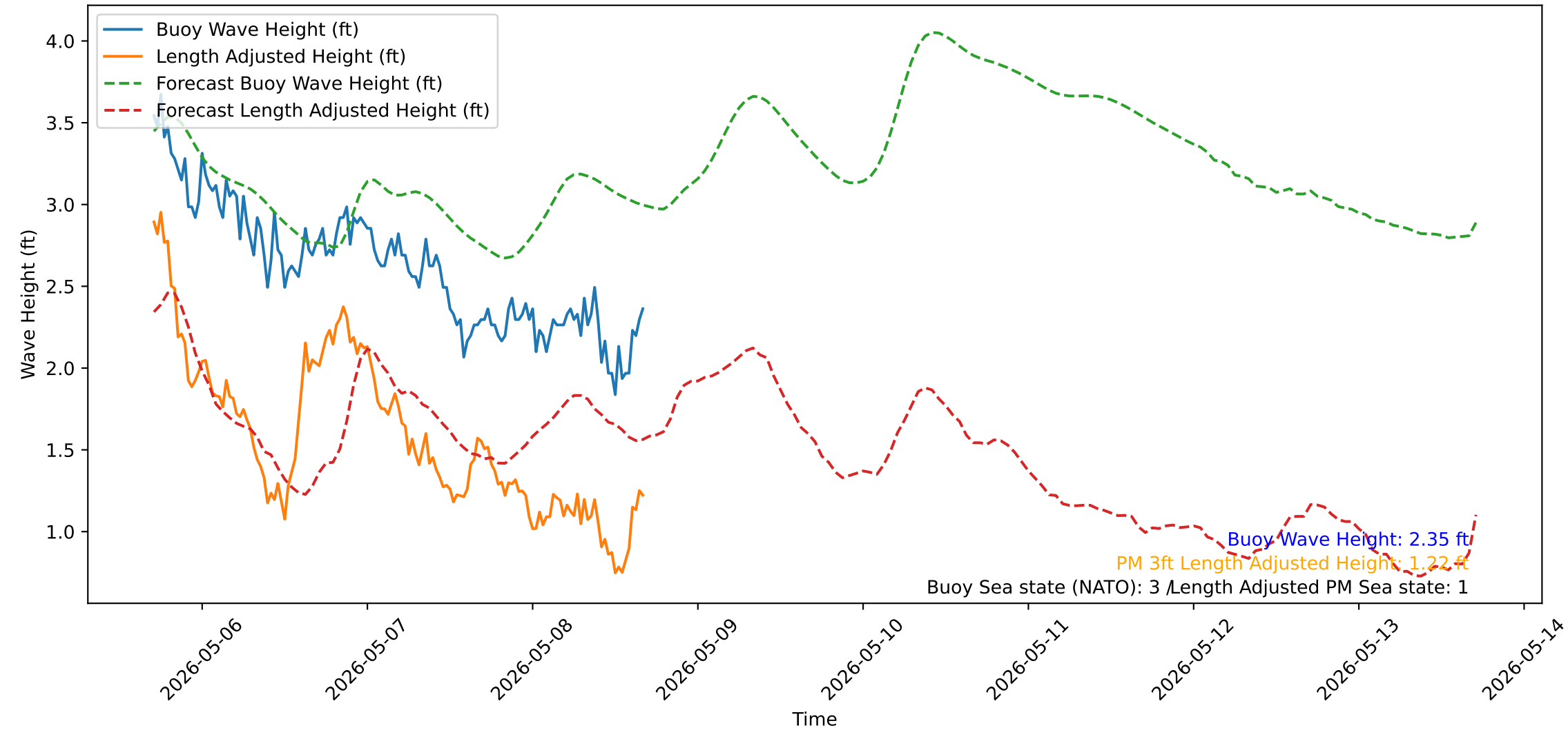
Wave Heights over Time for Green Beach at 2026-05-08 16:51:14
