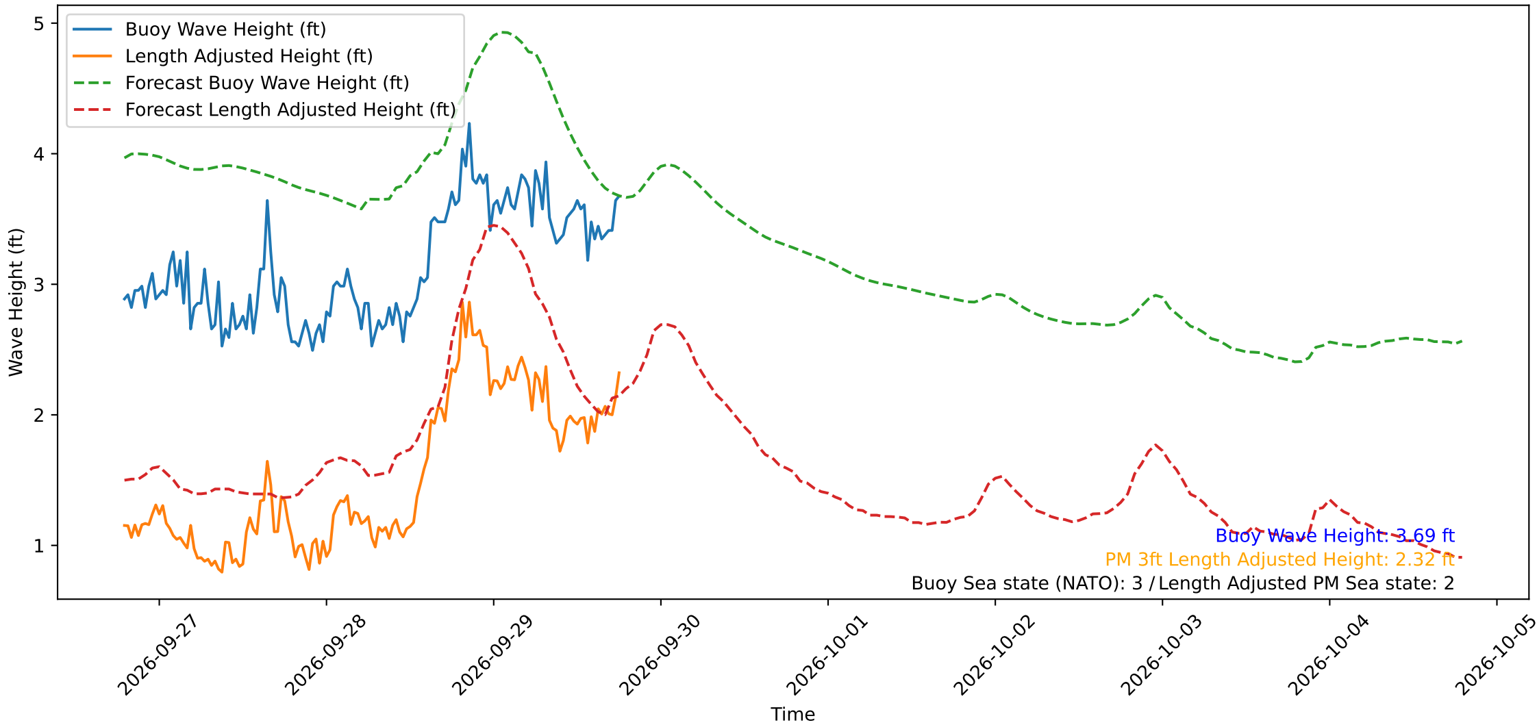
Wave Heights over Time for Oceanside Harbor at 2026-09-29 18:50:29
