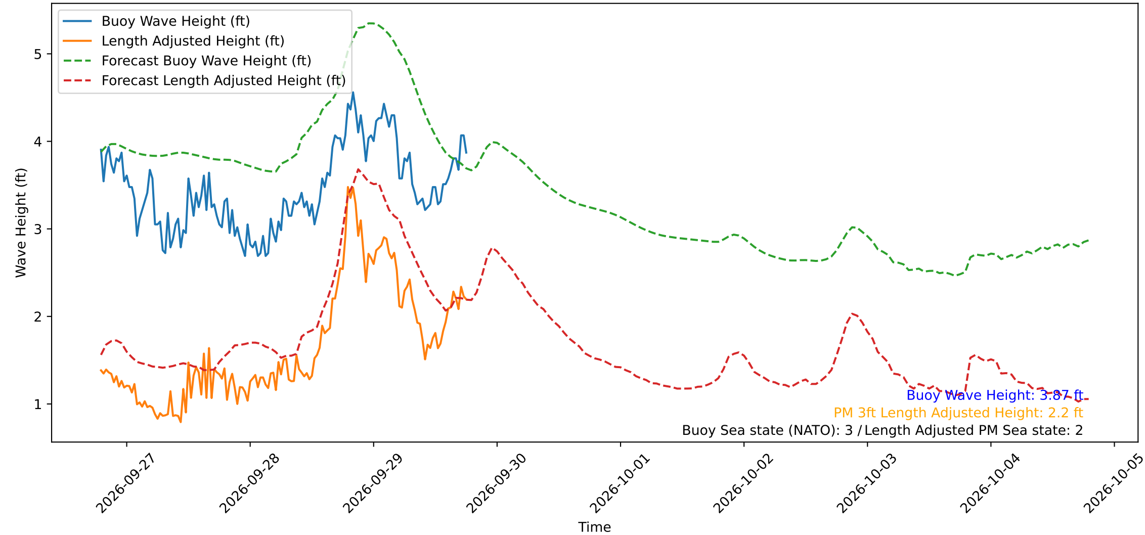
Wave Heights over Time for Green Beach at 2026-09-29 18:51:15
