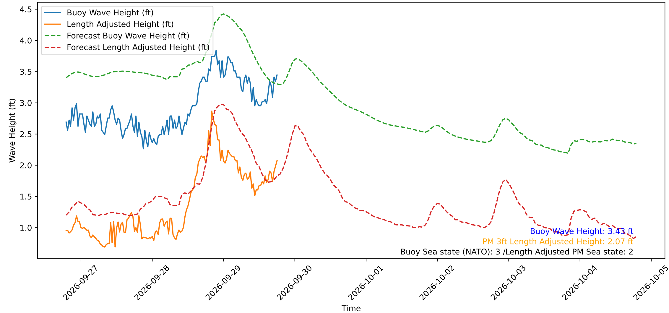
Wave Heights over Time for Red Beach at 2026-09-29 18:50:51
