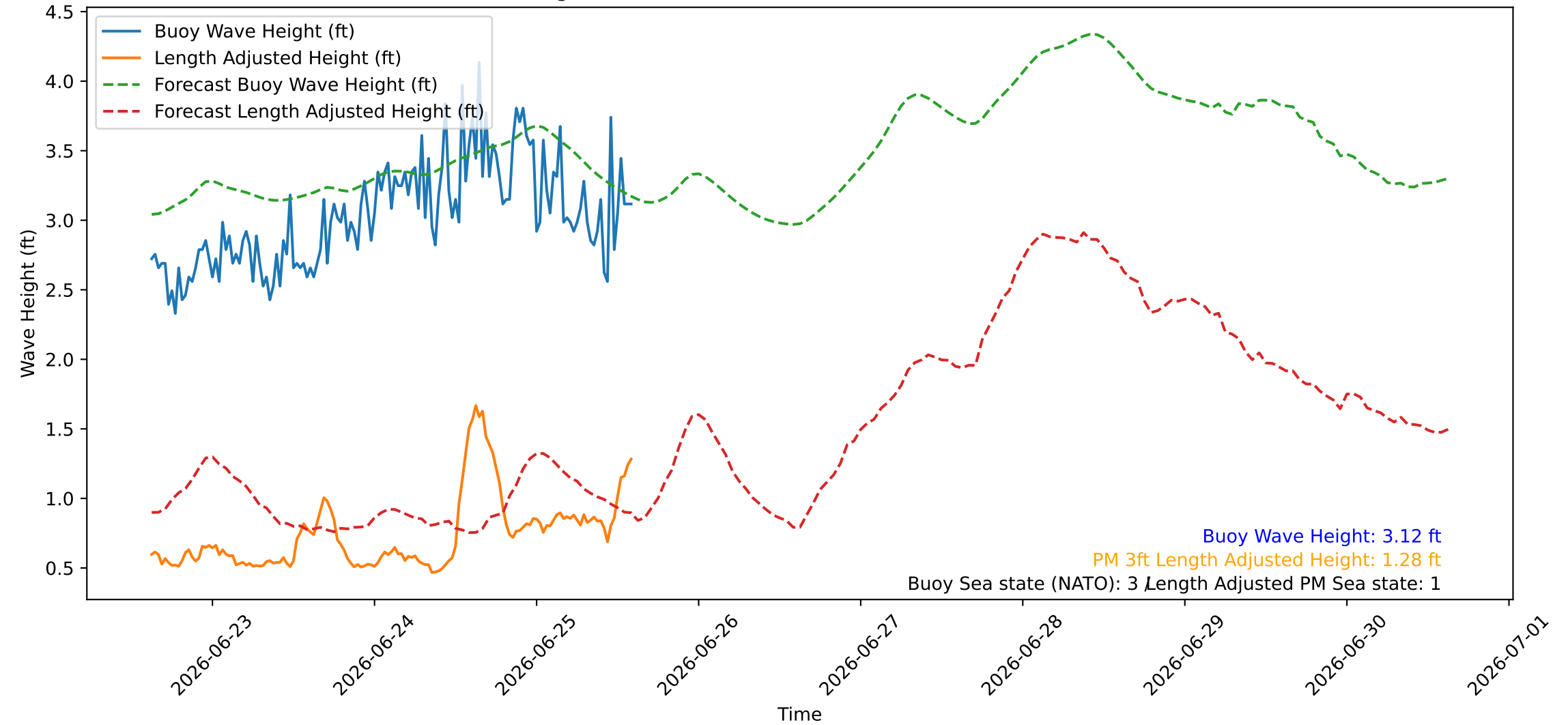
Wave Heights over Time for Red Beach at 2026-06-25 14:40:45
