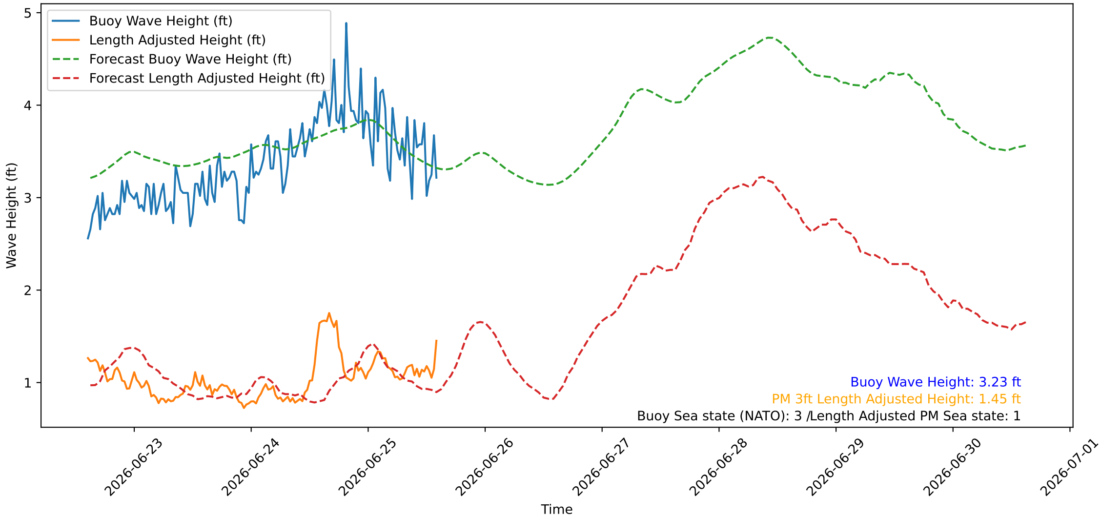
Wave Heights over Time for Oceanside Harbor at 2026-06-25 14:40:26
