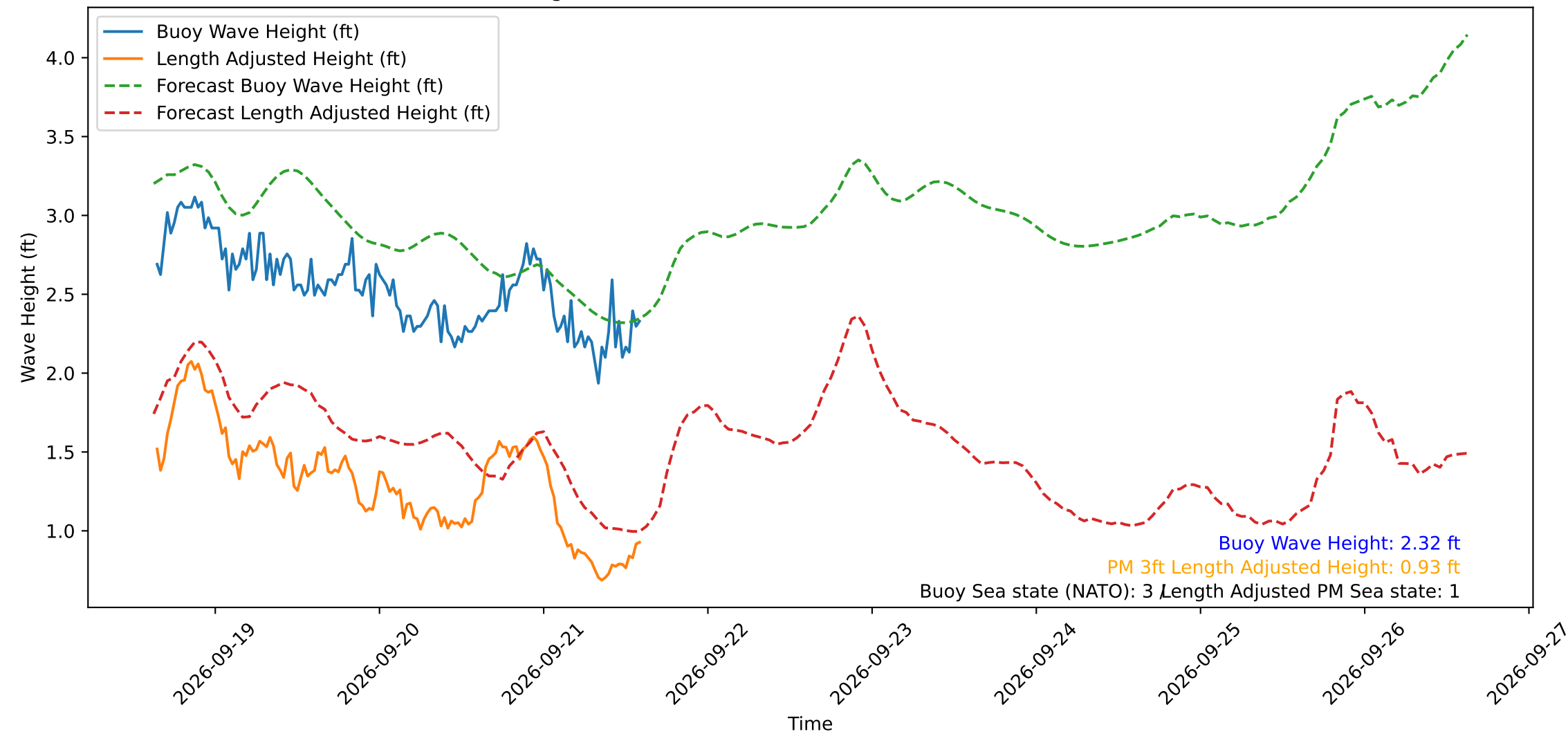
Wave Heights over Time for Green Beach at 2026-09-21 15:01:11
