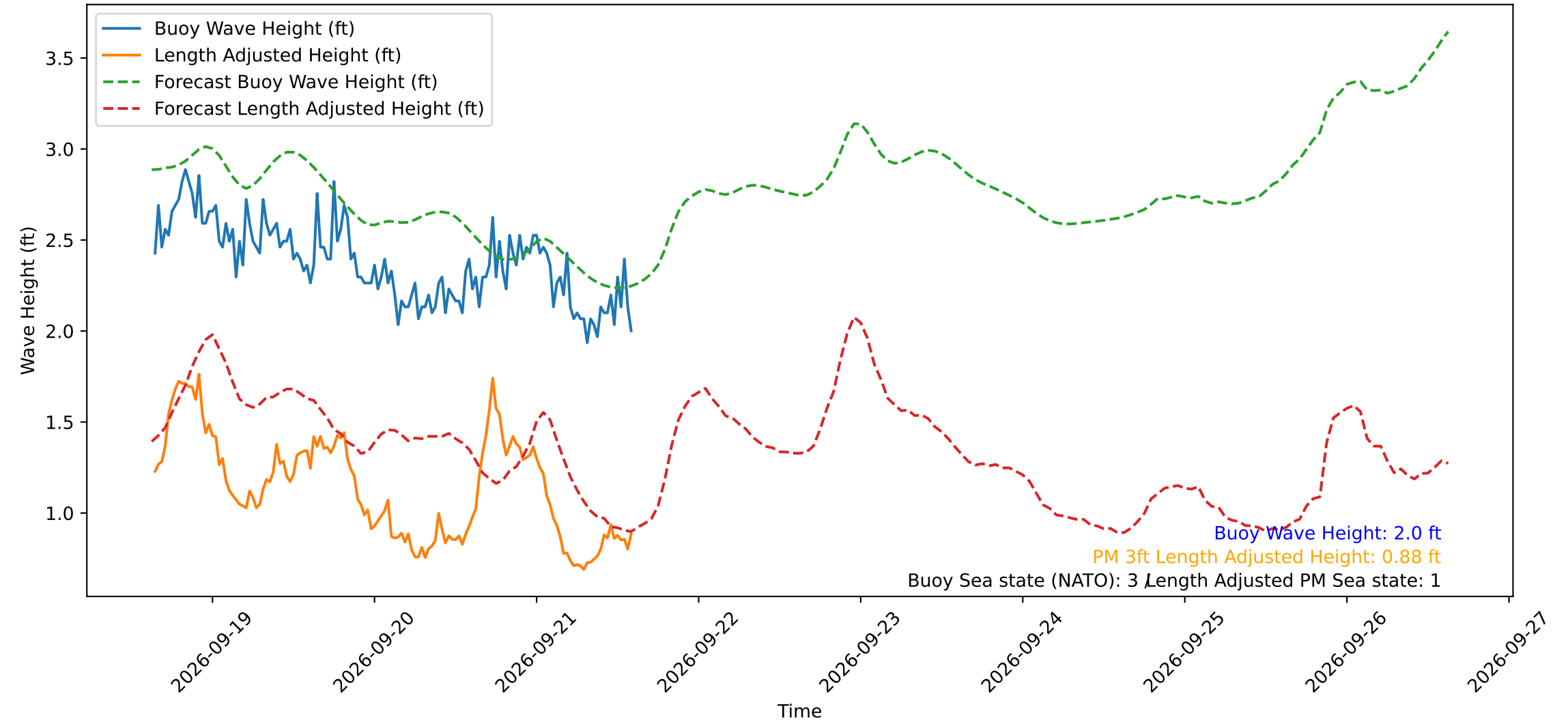
Wave Heights over Time for Red Beach at 2026-09-21 15:00:49
