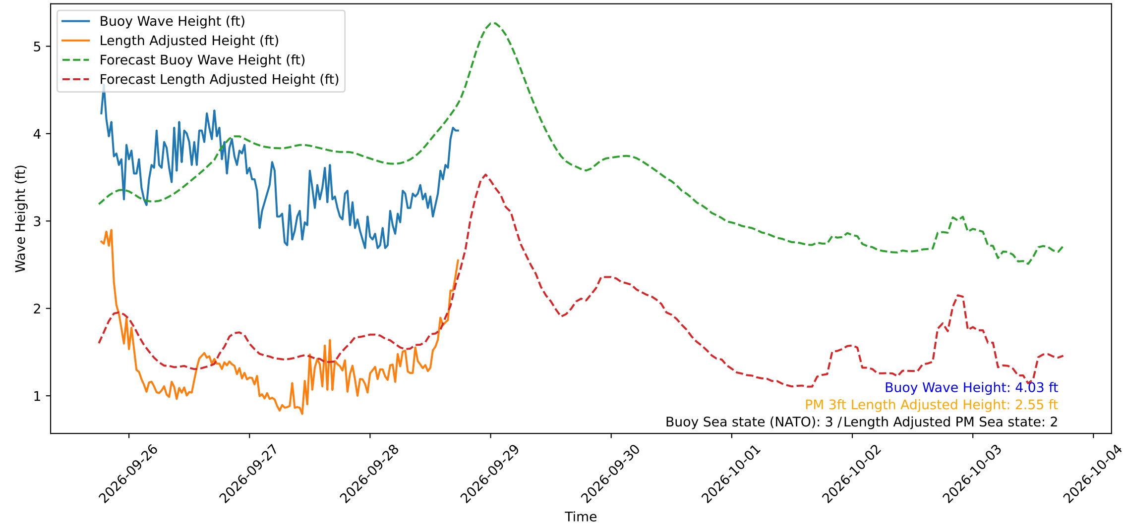
Wave Heights over Time for Green Beach at 2026-09-28 18:21:15
