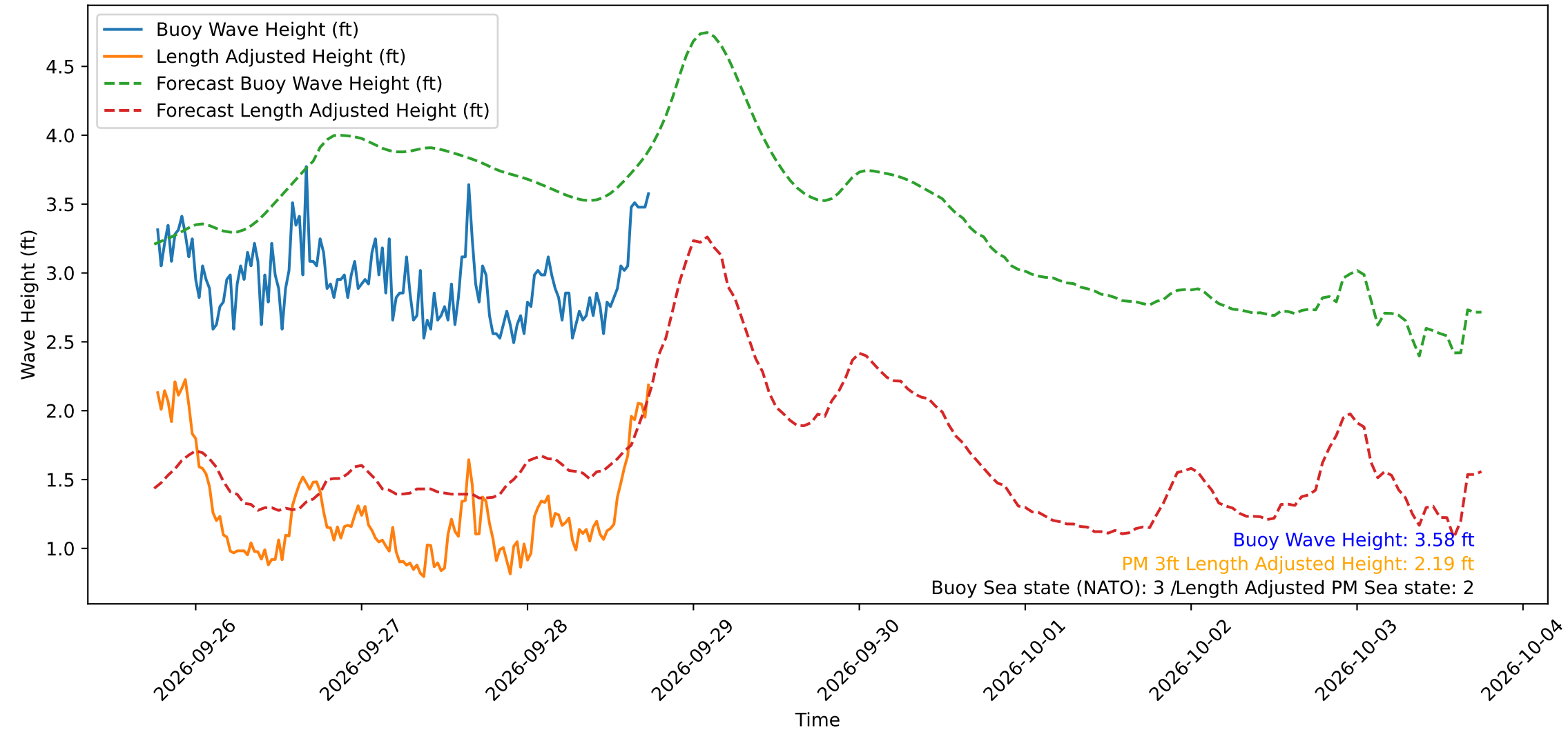
Wave Heights over Time for Oceanside Harbor at 2026-09-28 18:20:29
