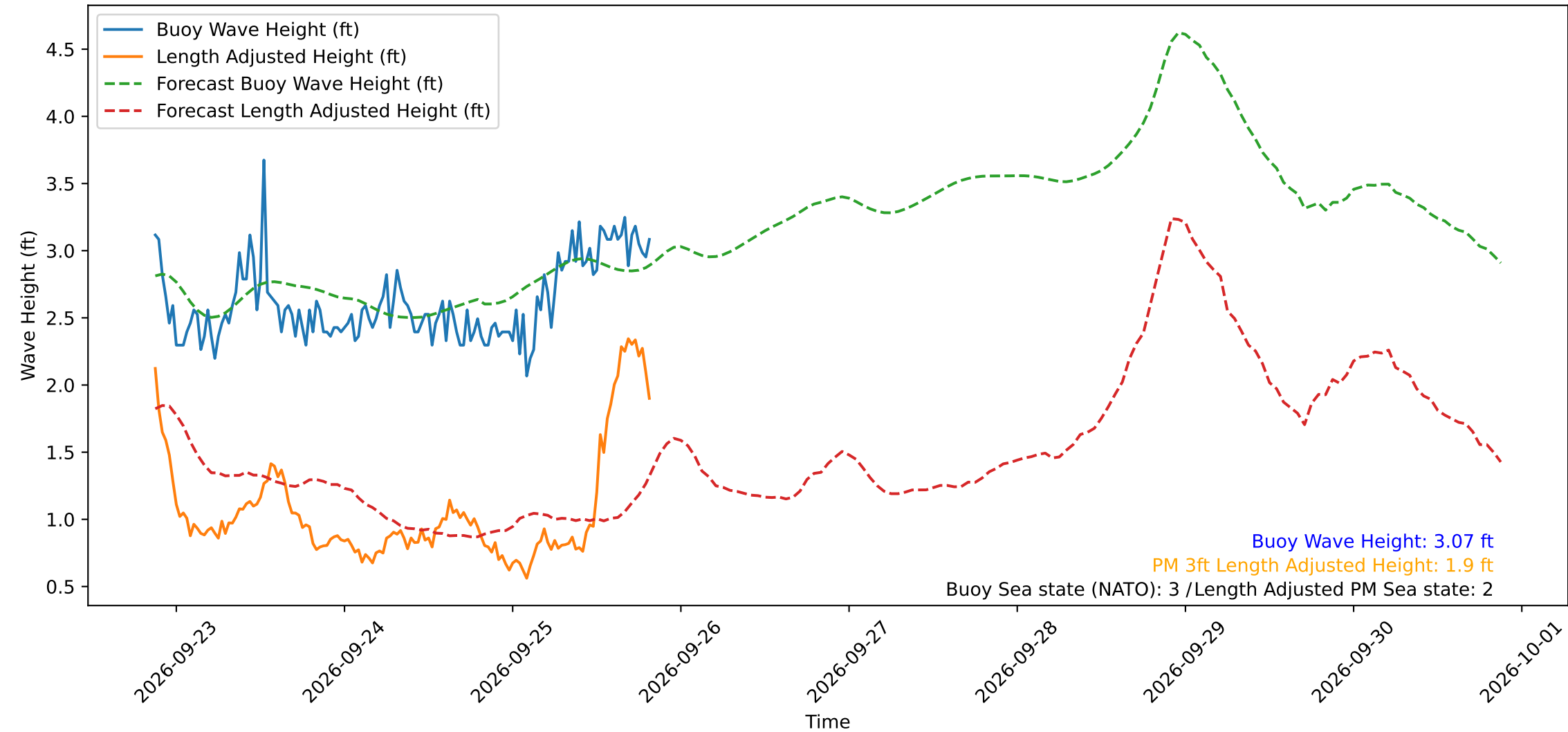
Wave Heights over Time for Red Beach at 2026-09-25 20:30:49
