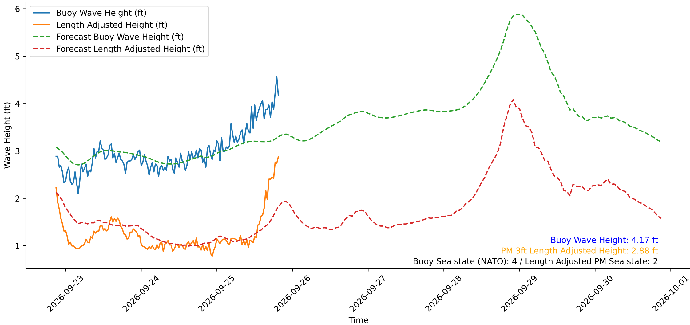
Wave Heights over Time for Green Beach at 2026-09-25 20:31:11
