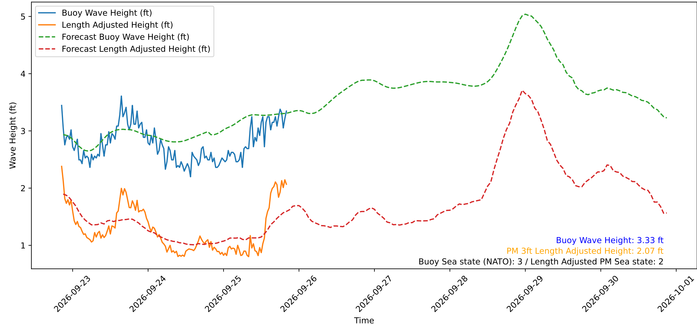
Wave Heights over Time for Oceanside Harbor at 2026-09-25 20:30:30
