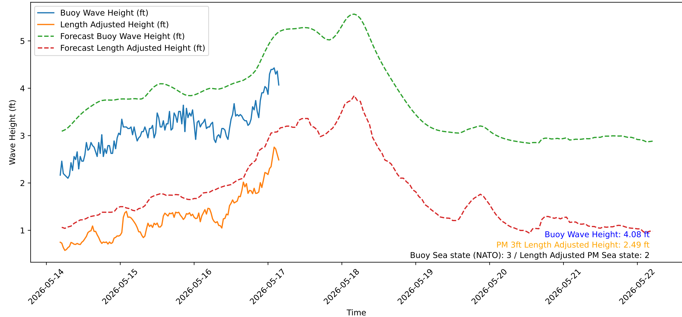
Wave Heights over Time for Green Beach at 2026-05-17 04:31:12
