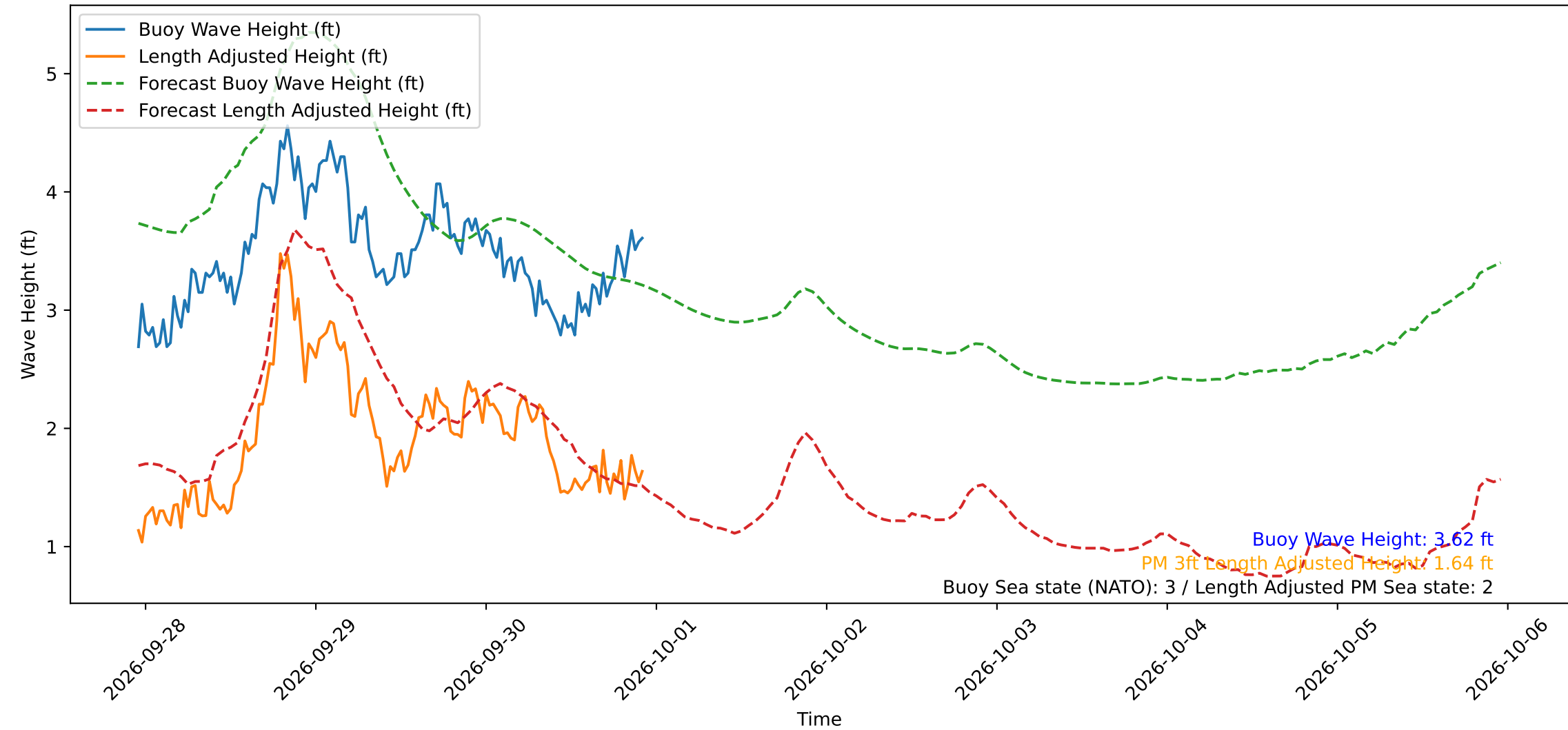
Wave Heights over Time for Green Beach at 2026-09-30 22:51:15
