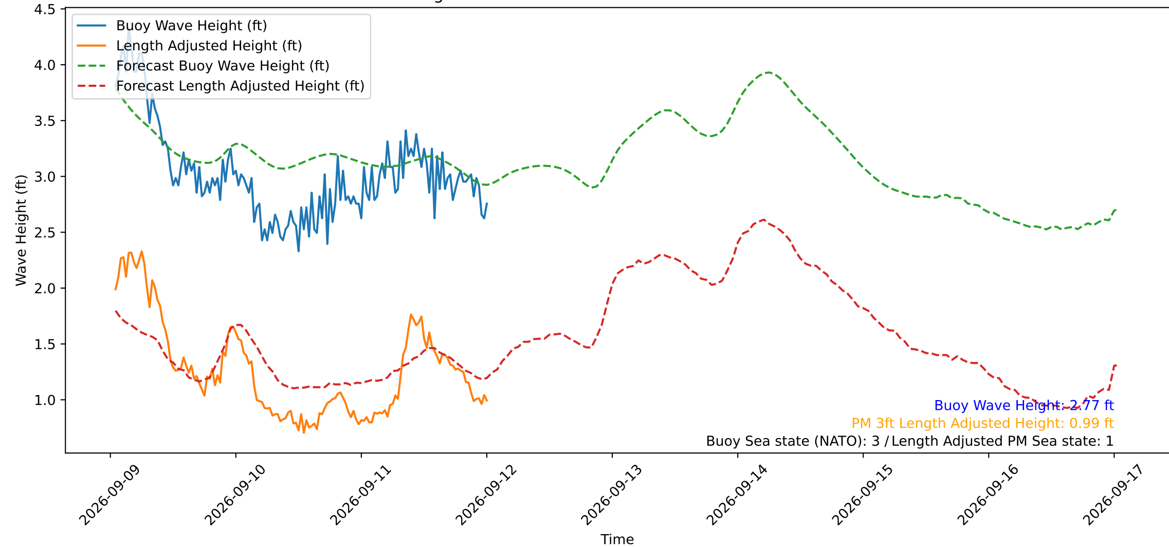
Wave Heights over Time for Red Beach at 2026-09-12 00:50:49
