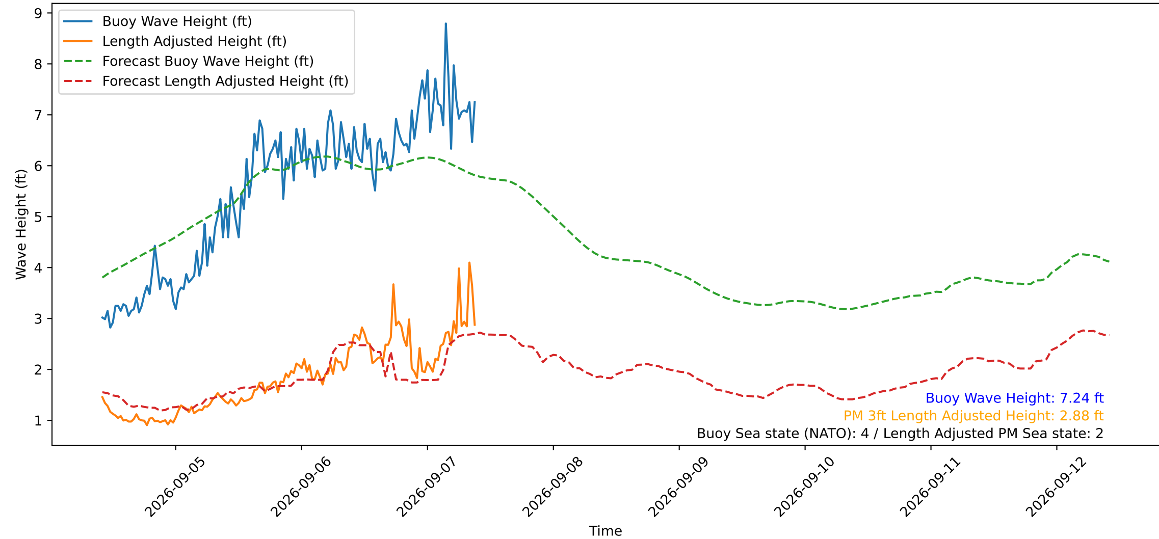
Wave Heights over Time for Green Beach at 2026-09-07 09:51:15
