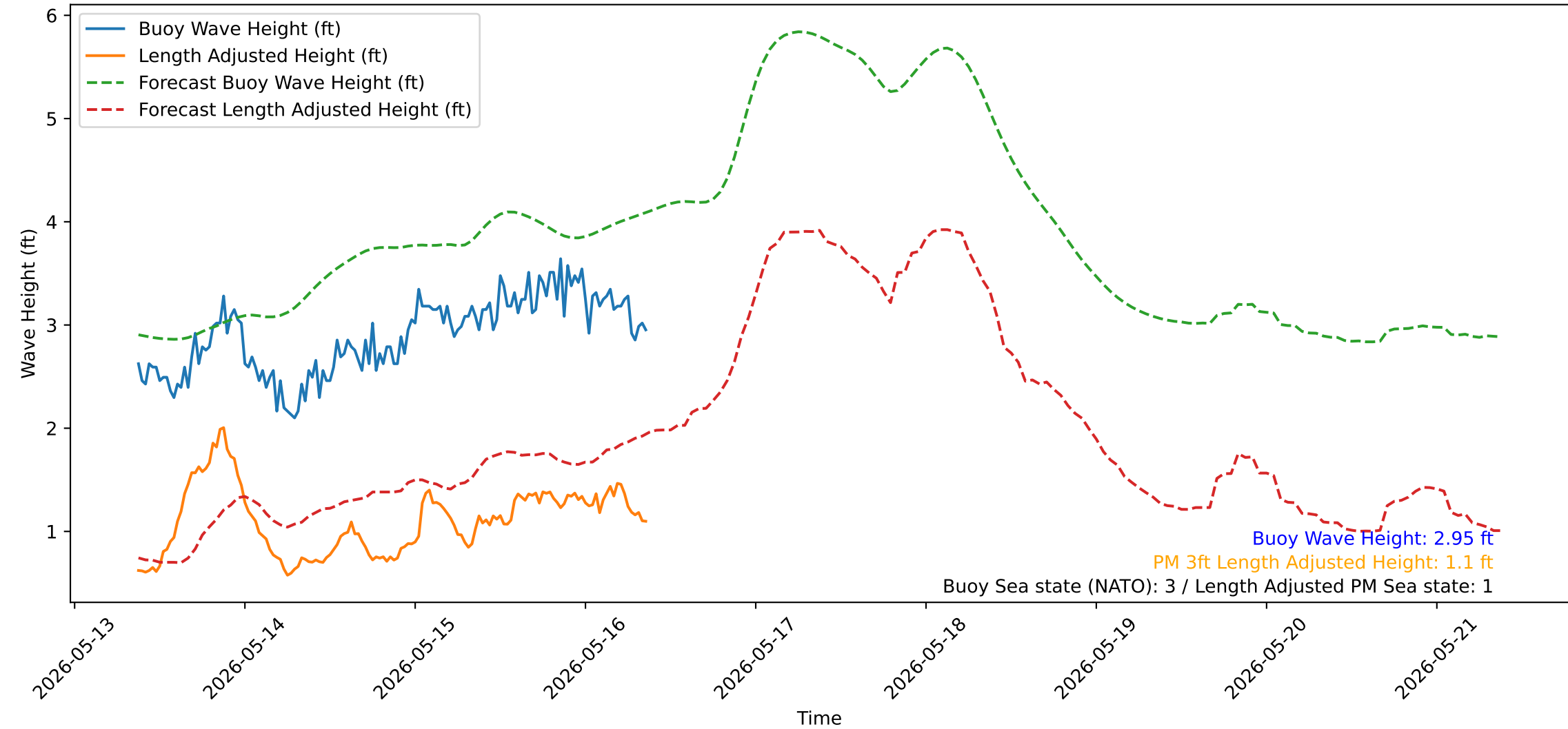
Wave Heights over Time for Green Beach at 2026-05-16 09:11:14
