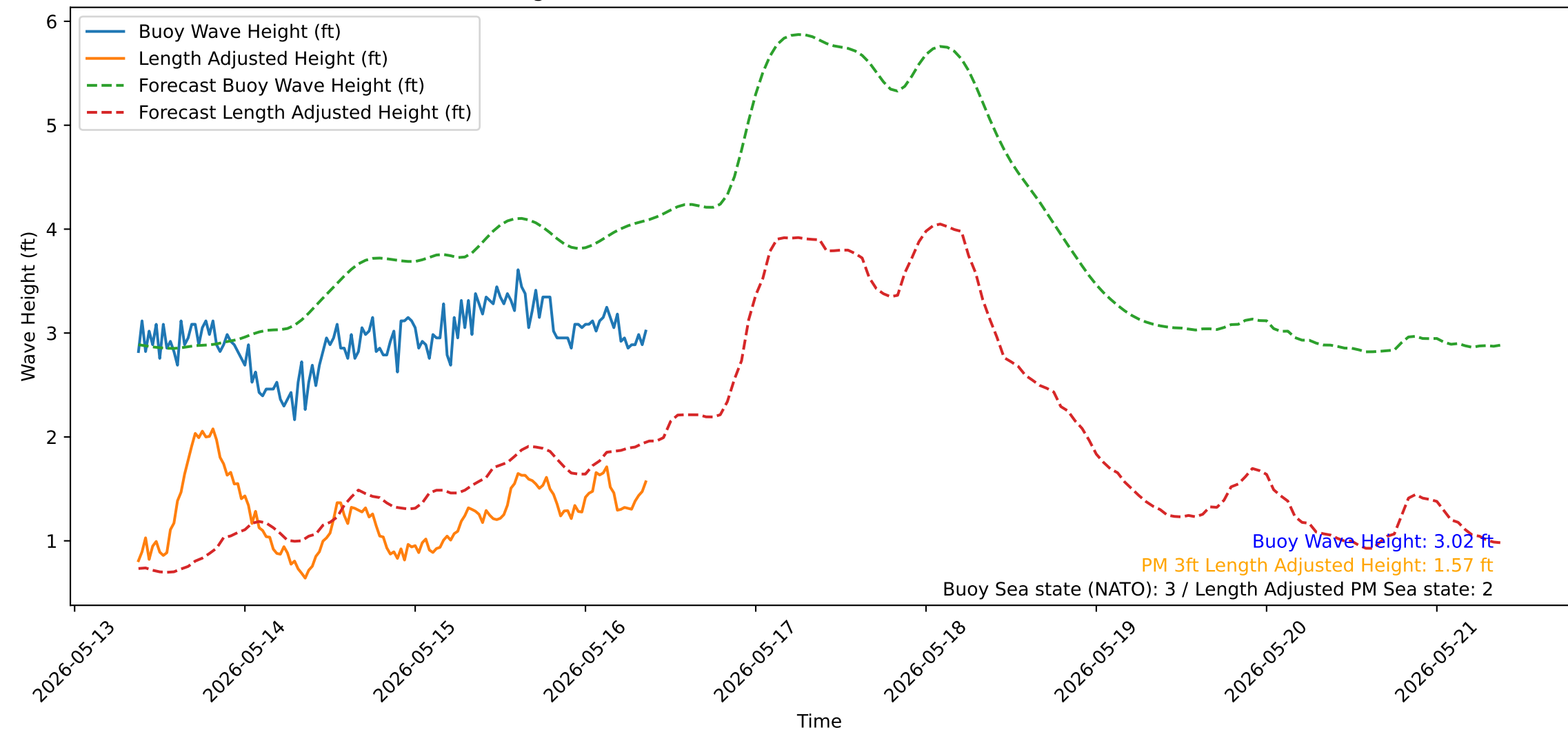
Wave Heights over Time for Oceanside Harbor at 2026-05-16 09:10:31
